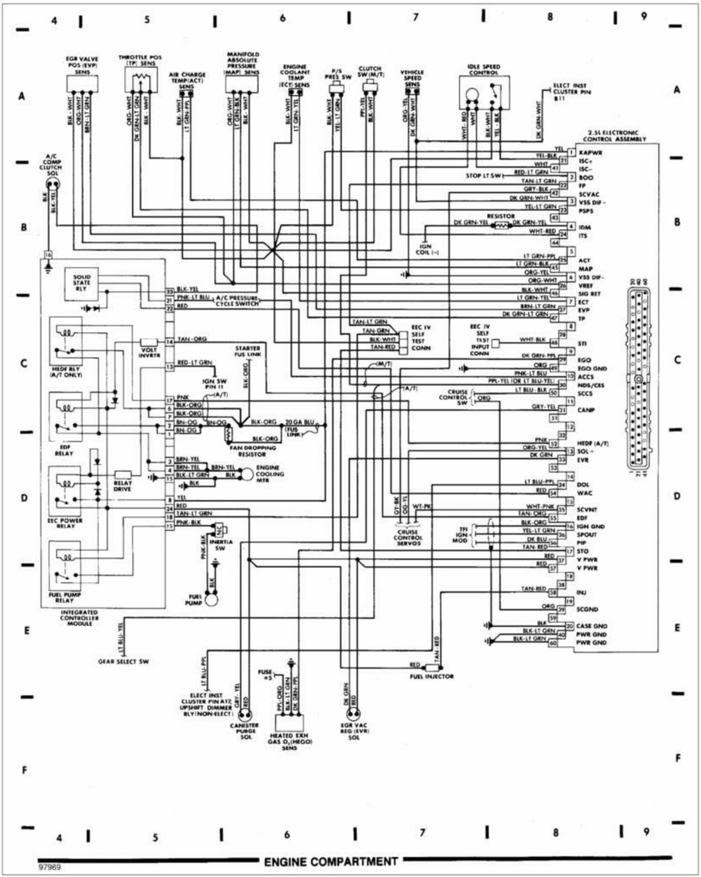
Fig. 2: Engine Compartment (Cont.) 1987 Ford Taurus LX
