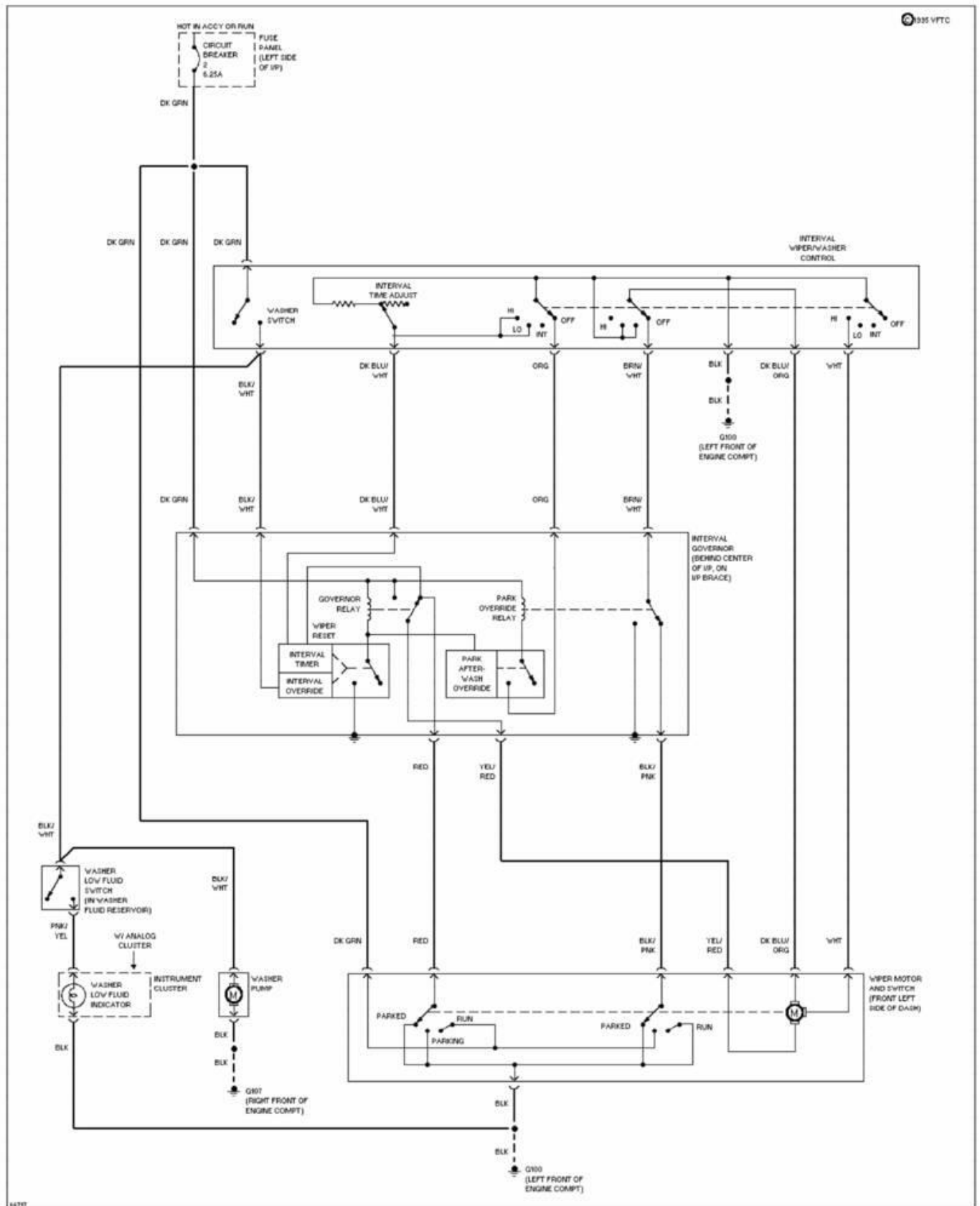
Fig. 17: Interval Wiper/Washer Circuit 1987 Ford Taurus LX
