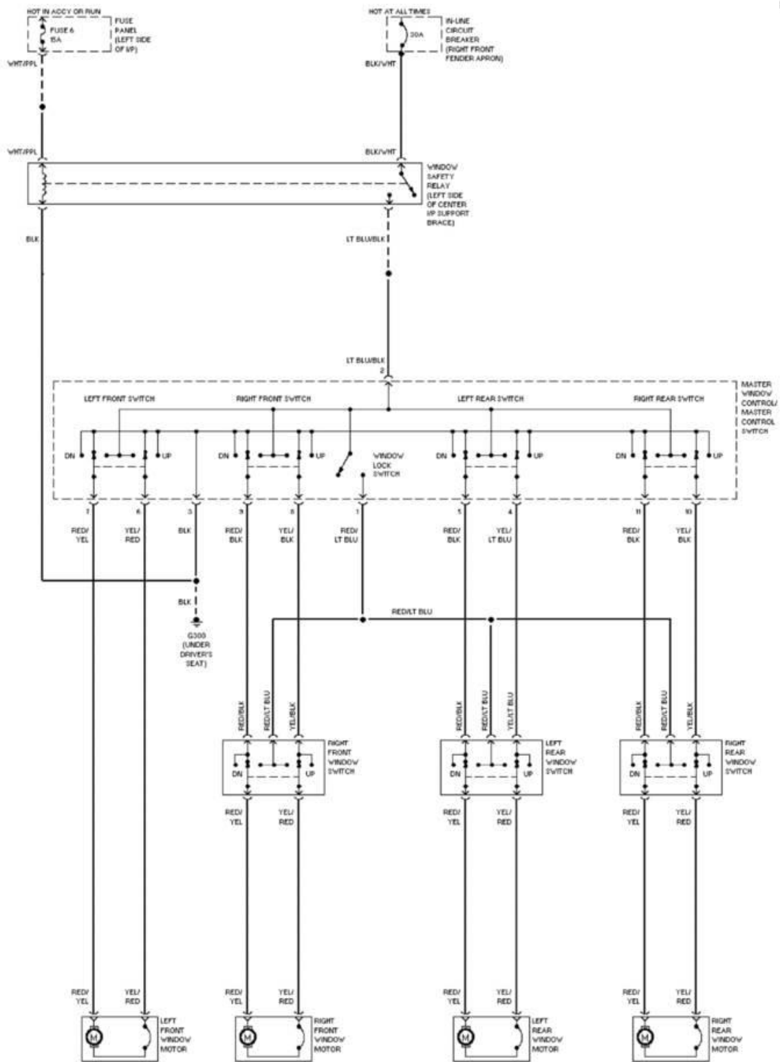
Fig. 9: Power Window Circuit 1987 Ford Taurus LX
