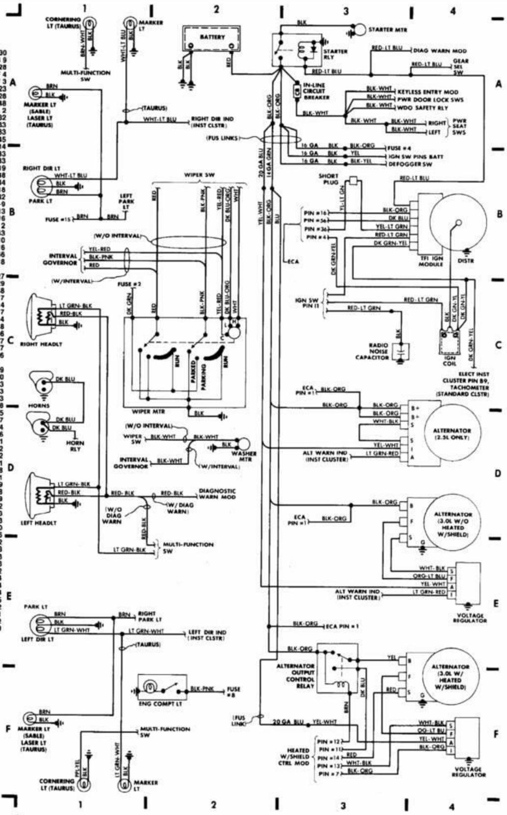
ENGINE COMPARTMENT
