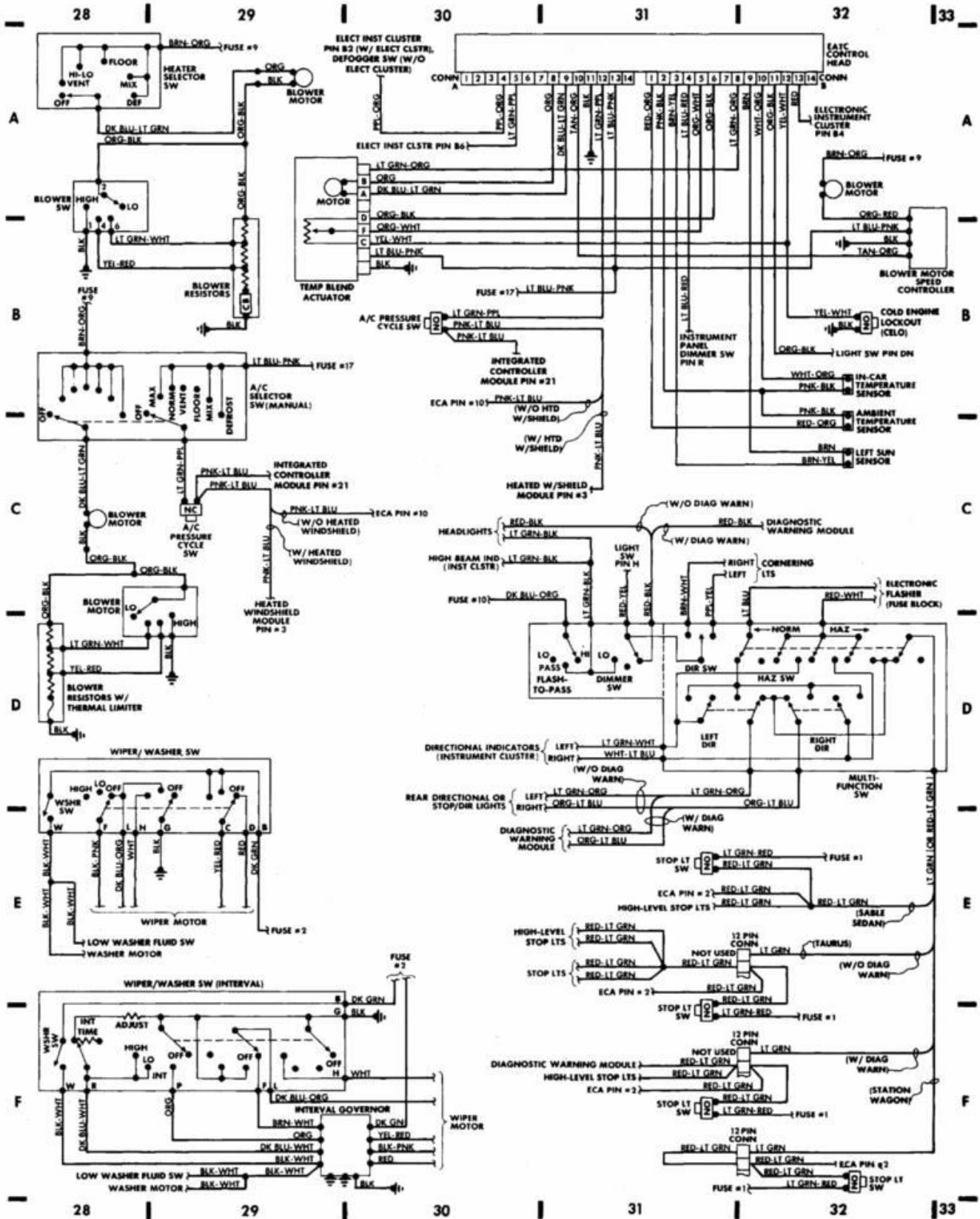
Fig. 7: Instrument Panel (Cont.) 1987 Ford Taurus LX
