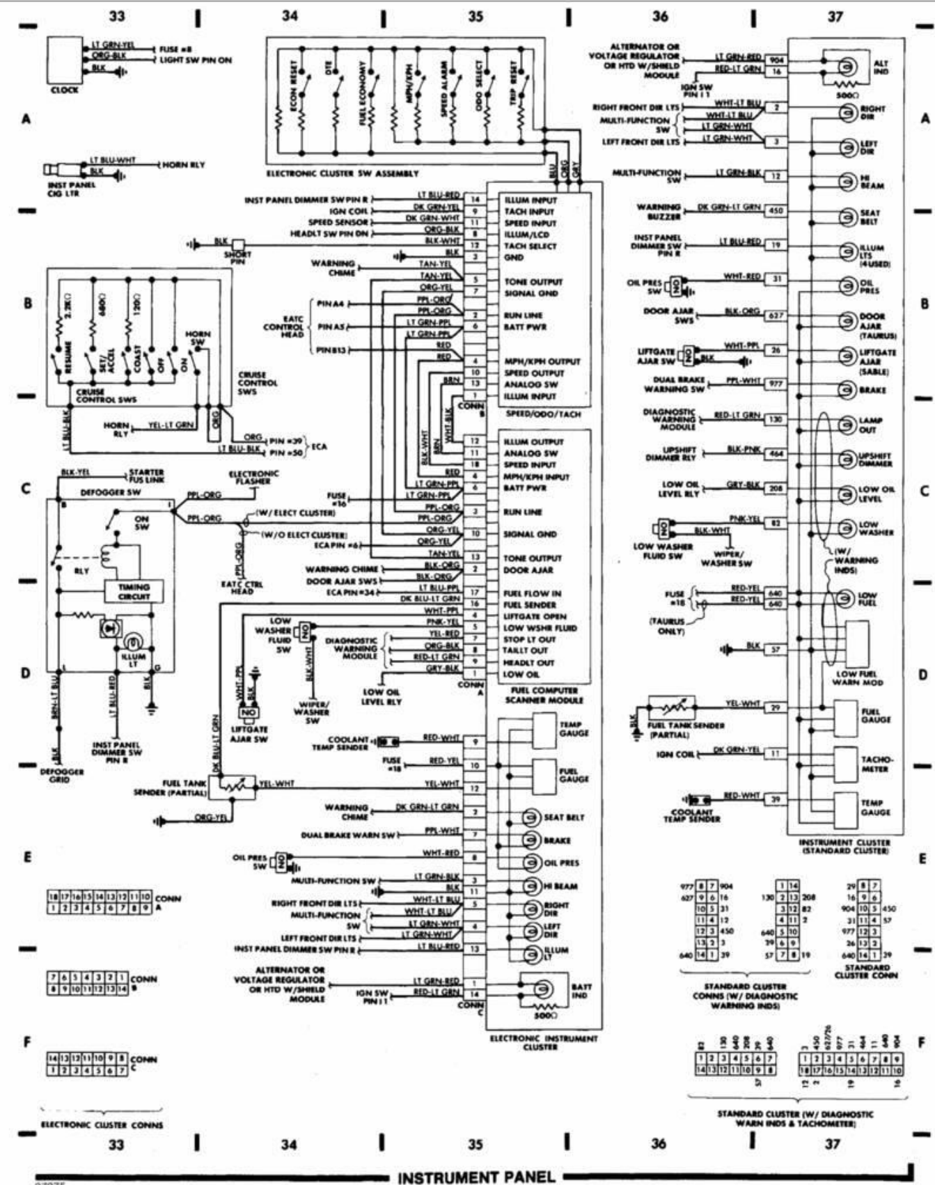
Fig. 8: Instrument Panel (Cont.) 1987 Ford Taurus LX
