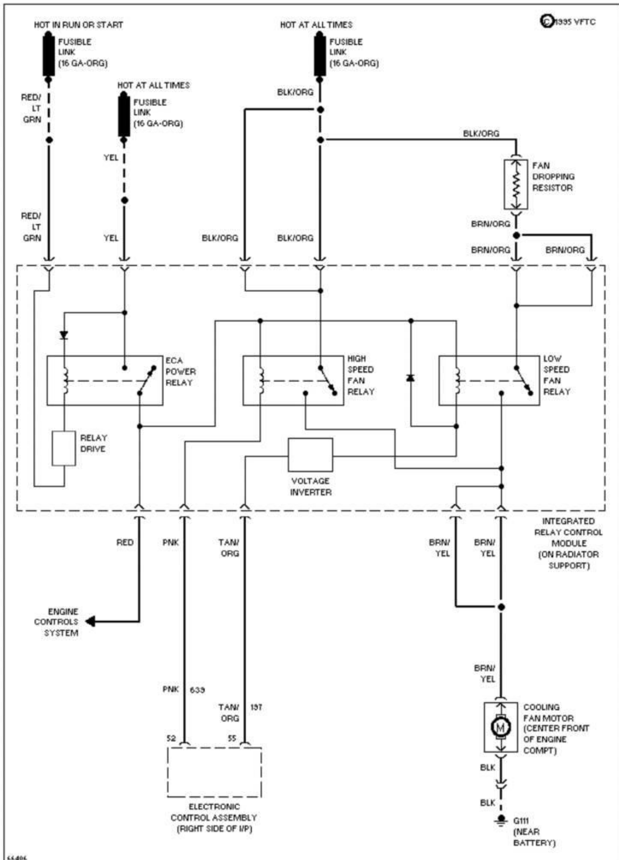
Fig. 1: Cooling Fan Circuit 1987 Ford Taurus LX
