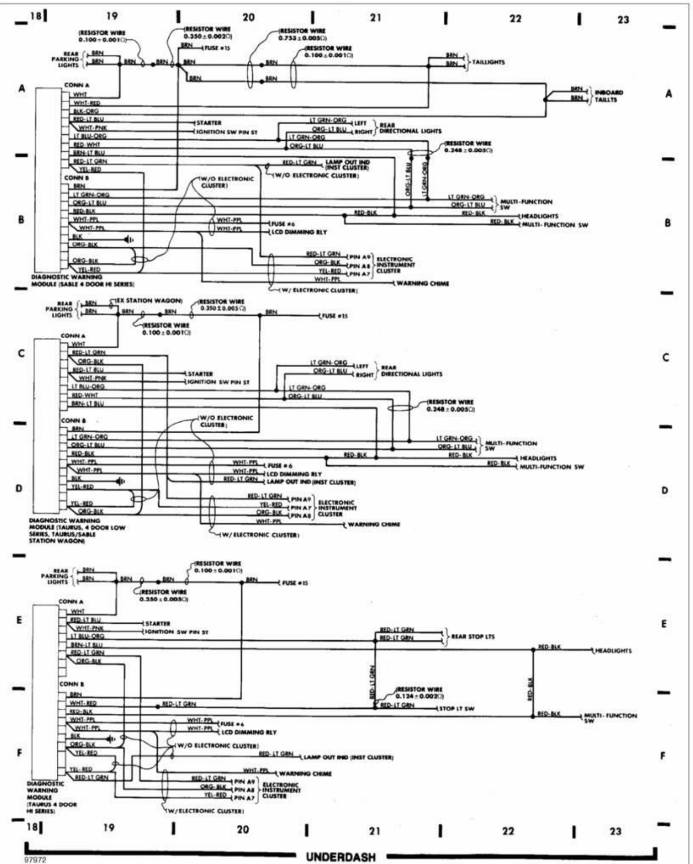
Fig. 5: Underdash (Cont.) 1987 Ford Taurus LX
