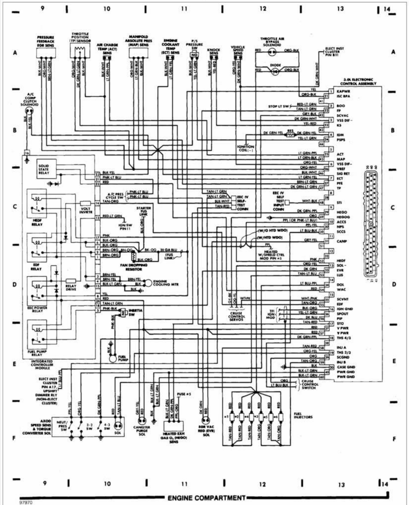
Fig. 3: Engine Compartment (Cont.) 1987 Ford Taurus LX
