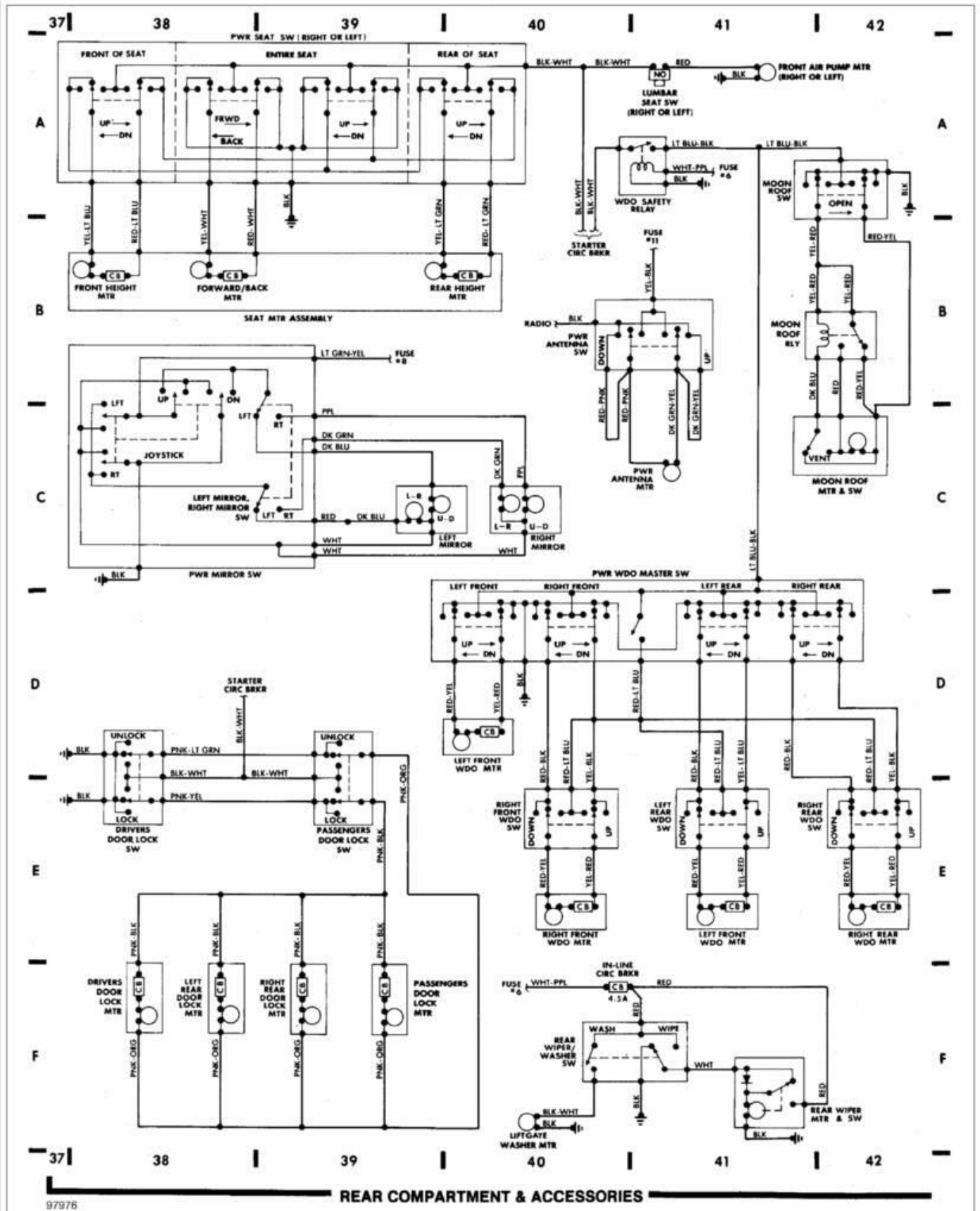
Fig. 9: Rear Compartment & Accessories 1987 Ford Taurus LX
