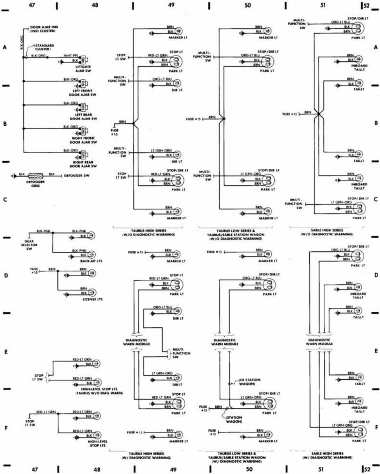
Fig. 11: Rear Compartment & Accessories (Cont.) 1987 Ford Taurus LX
