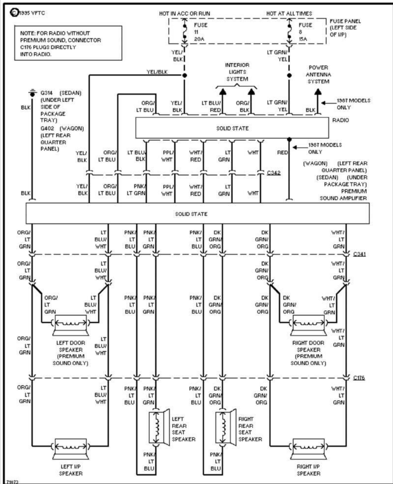
Fig. 10: Radio Circuits 1987 Ford Taurus LX
