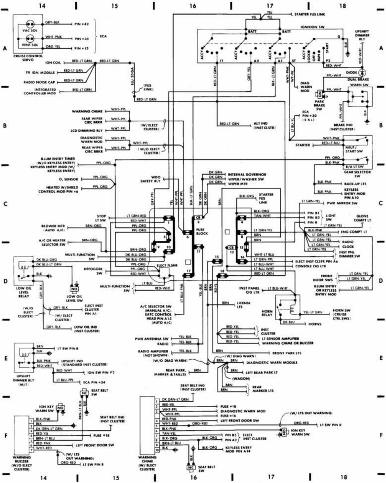
Fig. 4: Fuse Block & Underdash 1987 Ford Taurus LX
