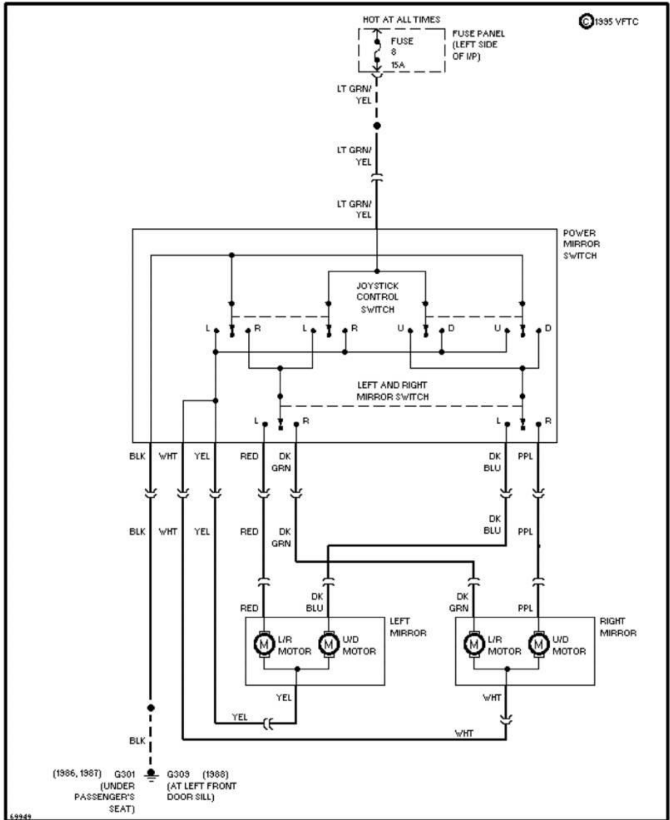
Fig. 6: Power Mirror Circuit 1987 Ford Taurus LX
