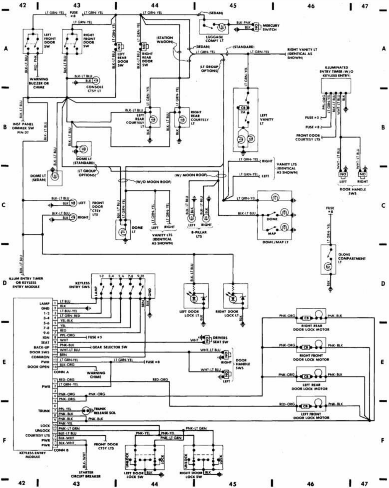
Fig. 10: Rear Compartment & Accessories (Cont.) 1987 Ford Taurus LX
