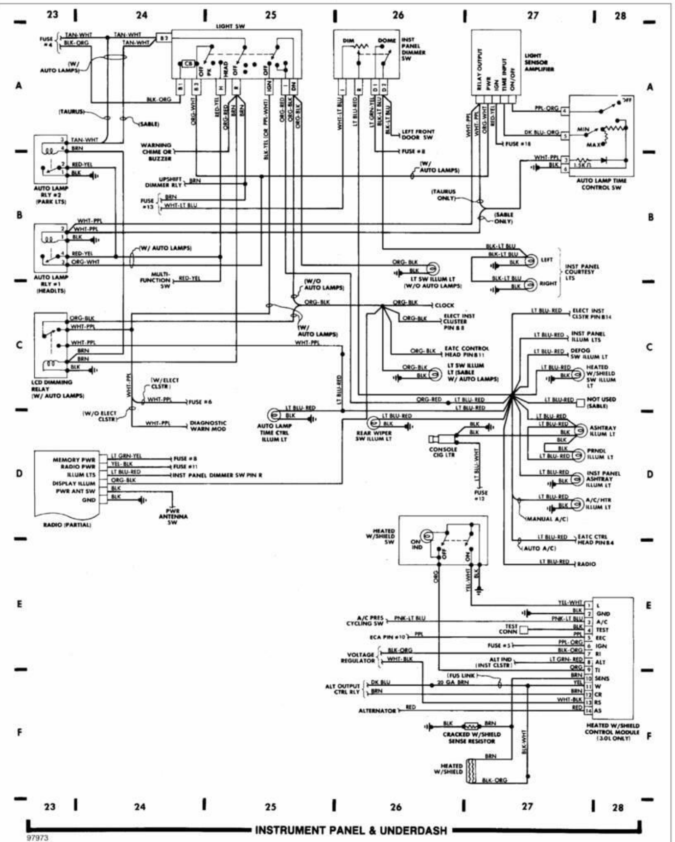
Fig. 6: Underdash (Cont.) & Instrument Panel 1987 Ford Taurus LX
