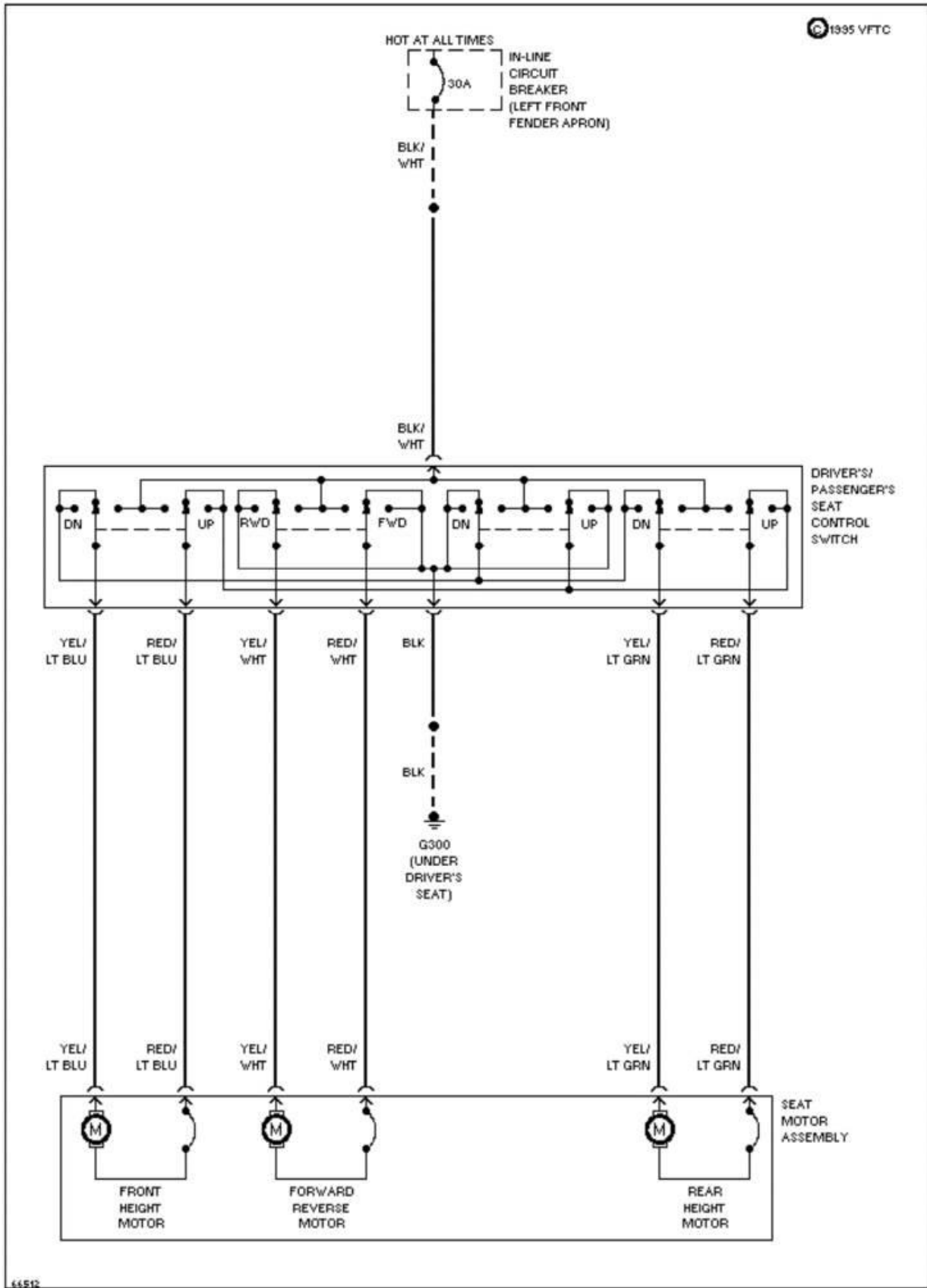
Fig. 8: Power Seat Circuit 1987 Ford Taurus LX
