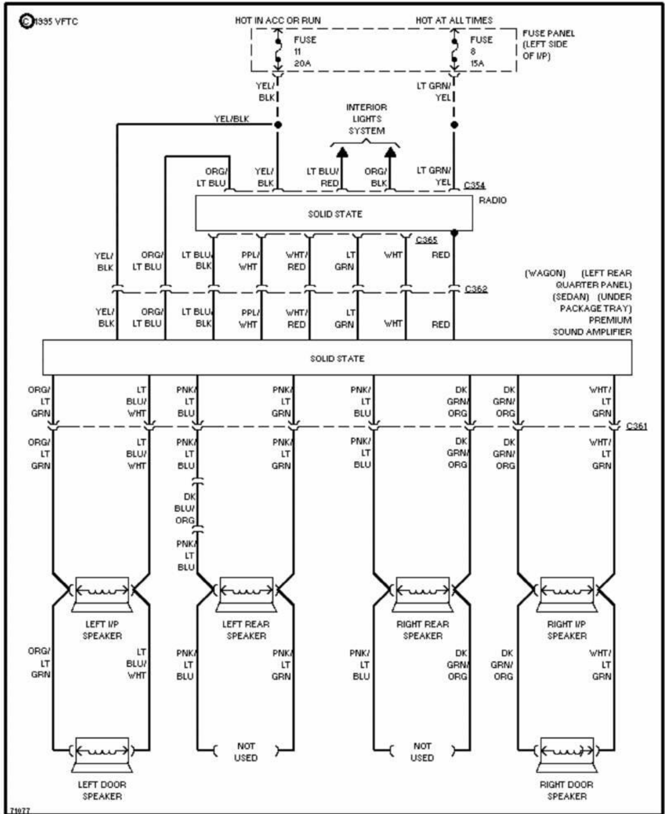
Fig. 14: Premium Sound Radio Circuit, Standard/AAV 1989 Ford Taurus LX
