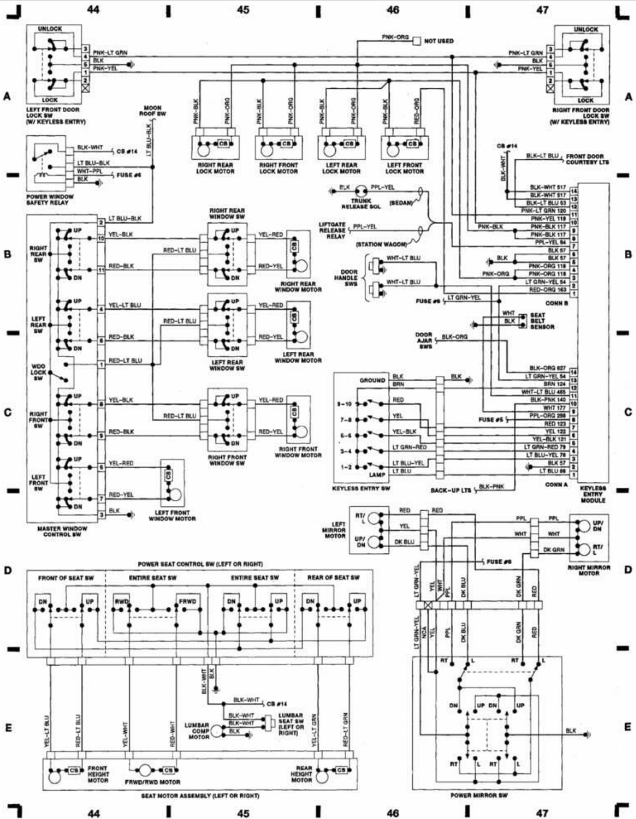
Fig. 12: Passenger Compartment 1989 Ford Taurus LX
