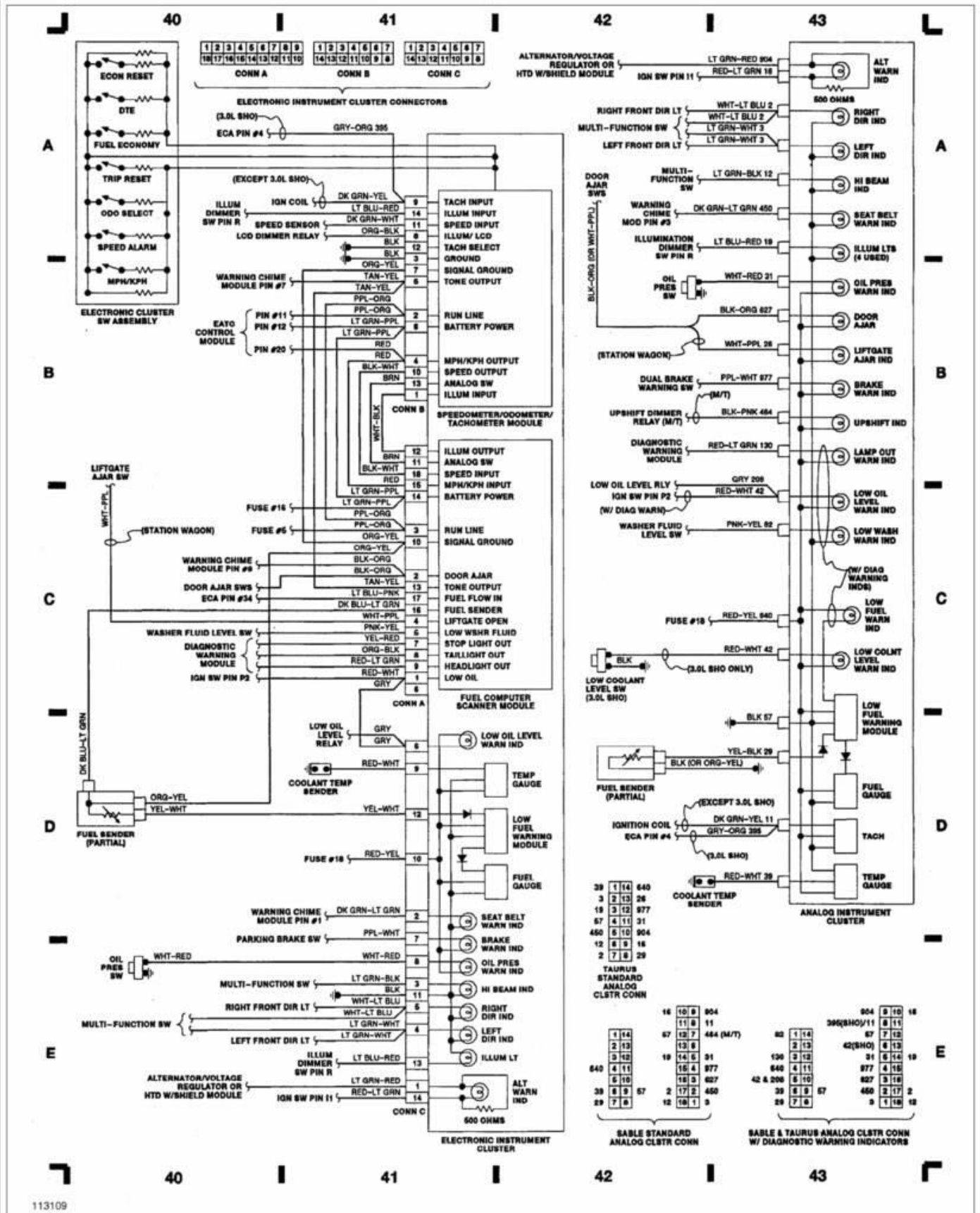
Fig. 11: Instrument Panel 1989 Ford Taurus LX
