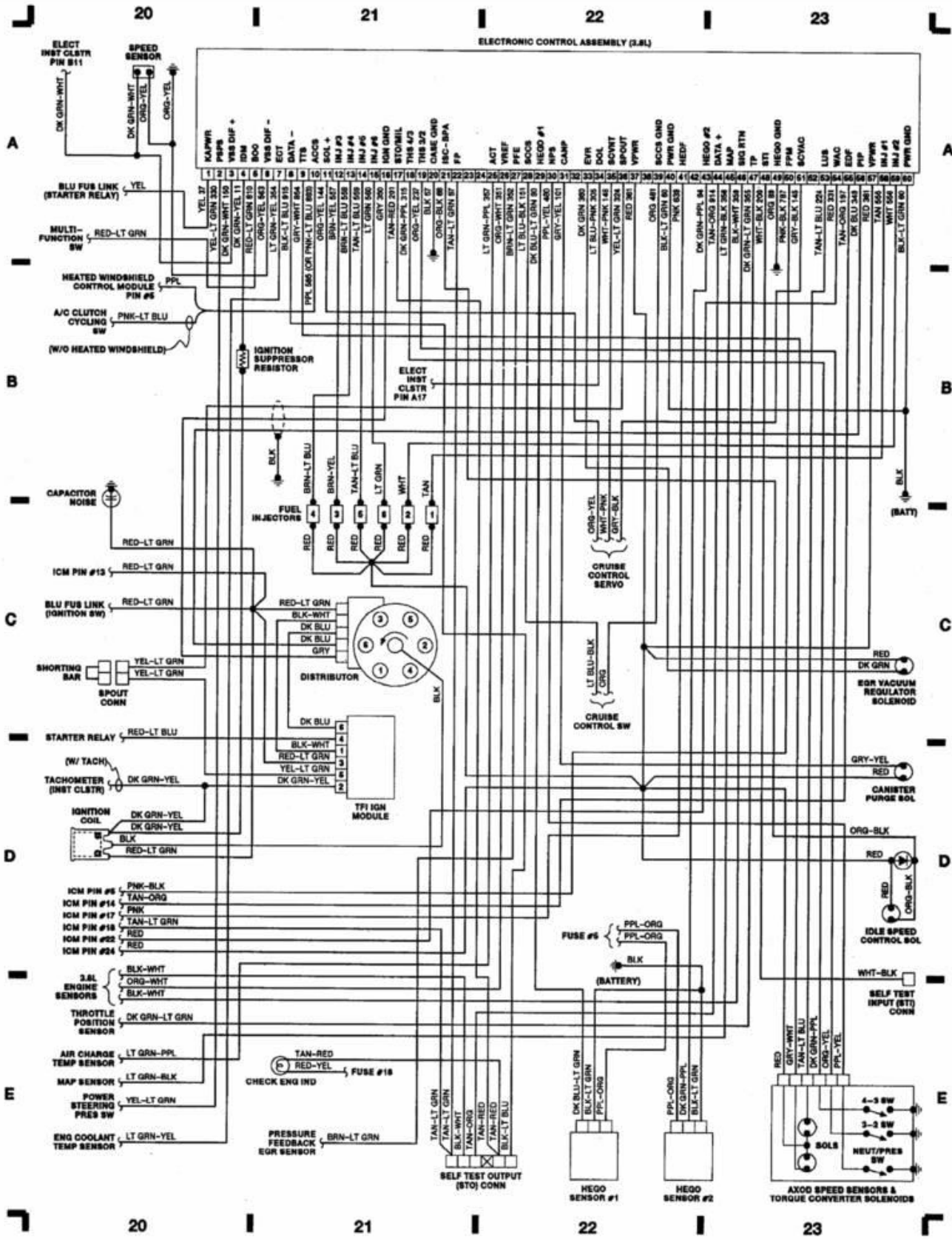
Fig. 6: Computer Engine Control (3.8L) 1989 Ford Taurus LX
