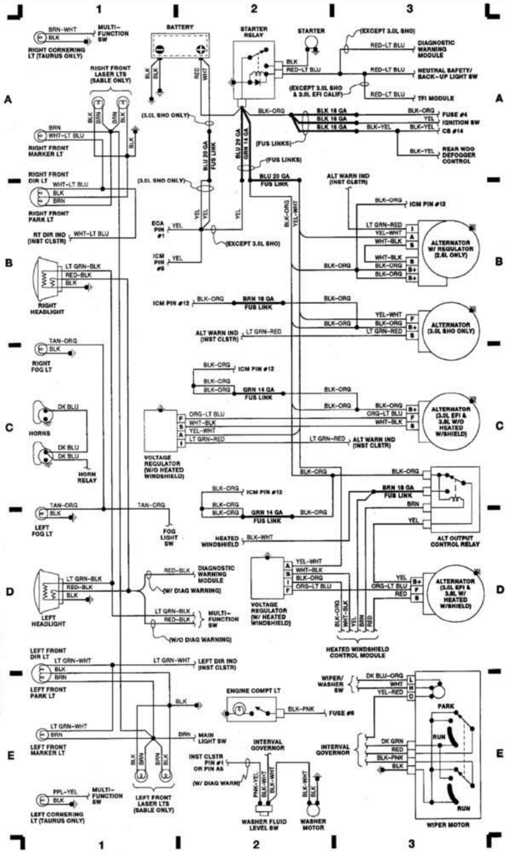
Fig. 1: Engine Compartment & Headlights 1989 Ford Taurus LX
