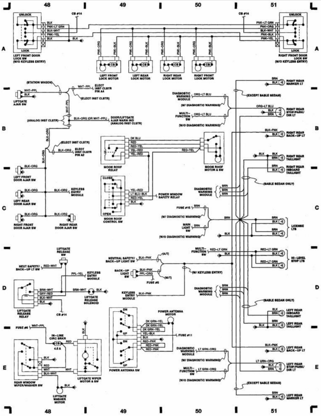
Fig. 13: Passenger Compartment (Cont.) & Taillights 1989 Ford Taurus LX
