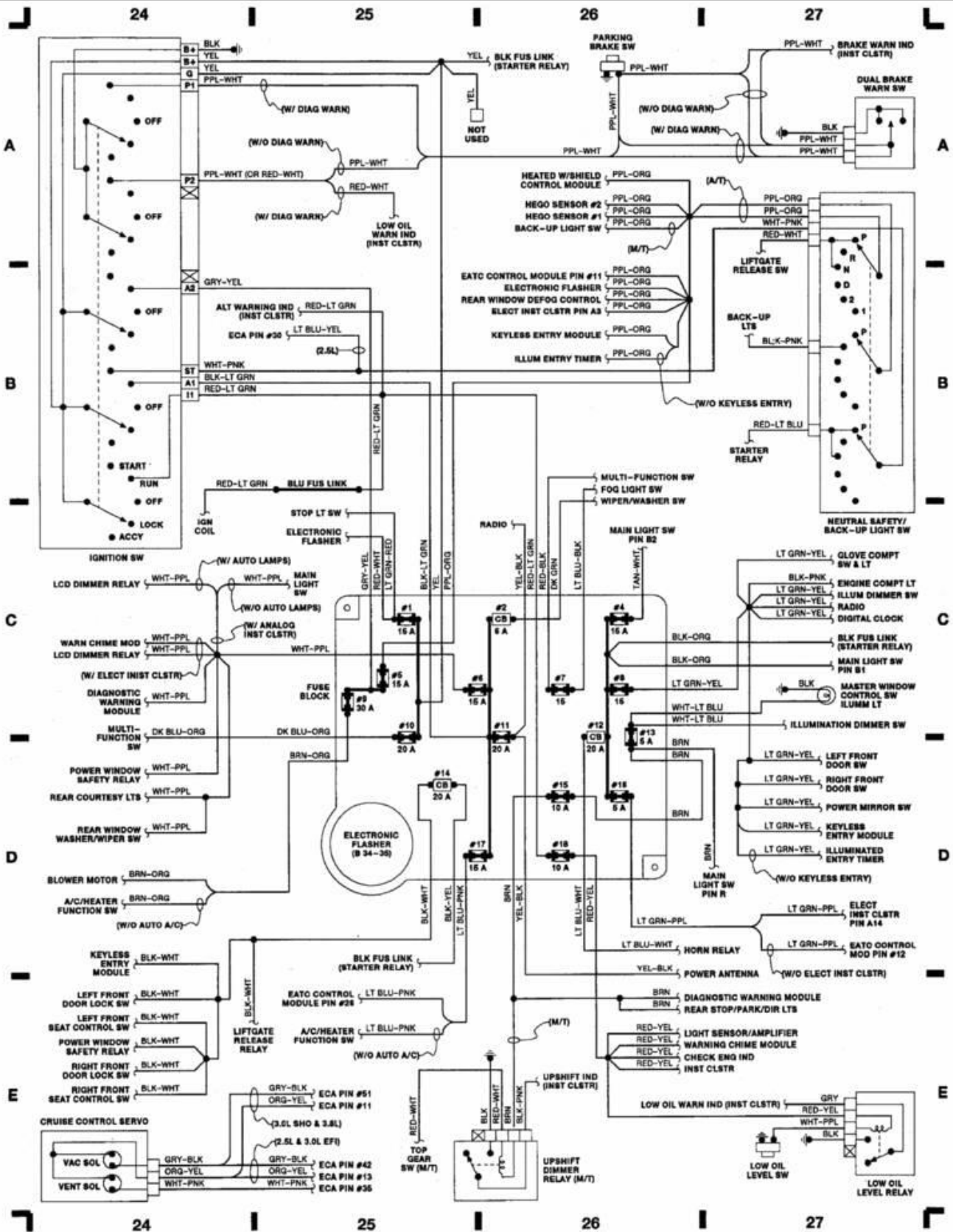
Fig. 7: Fuse Block 1989 Ford Taurus LX
