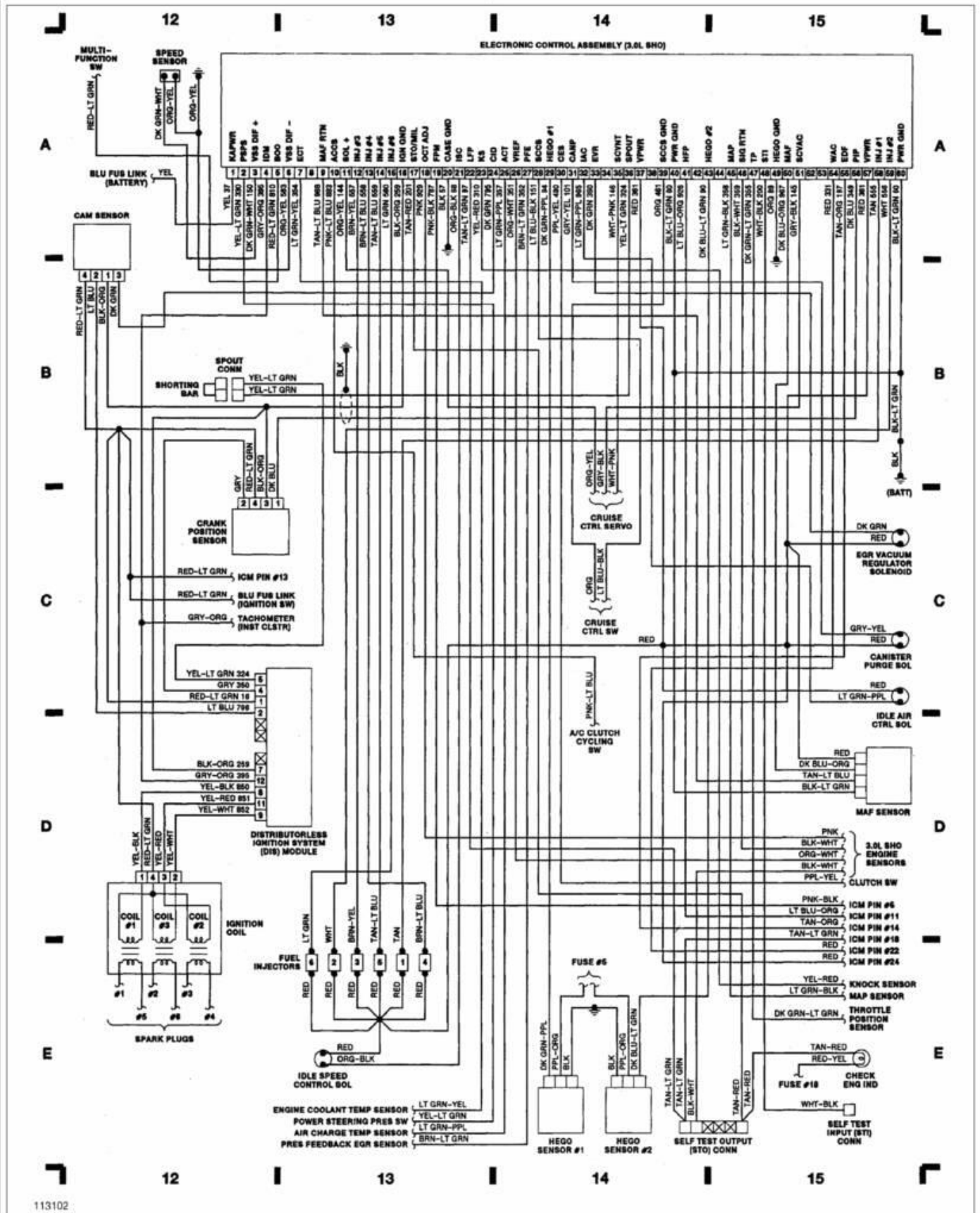
Fig. 4: Computer Engine Control (3.0L SHO) 1989 Ford Taurus LX
