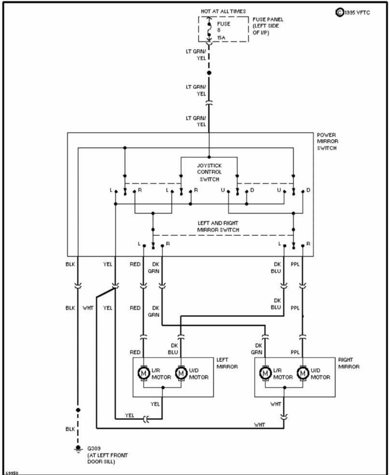
Fig. 10: Power Mirror Circuit 1989 Ford Taurus LX
