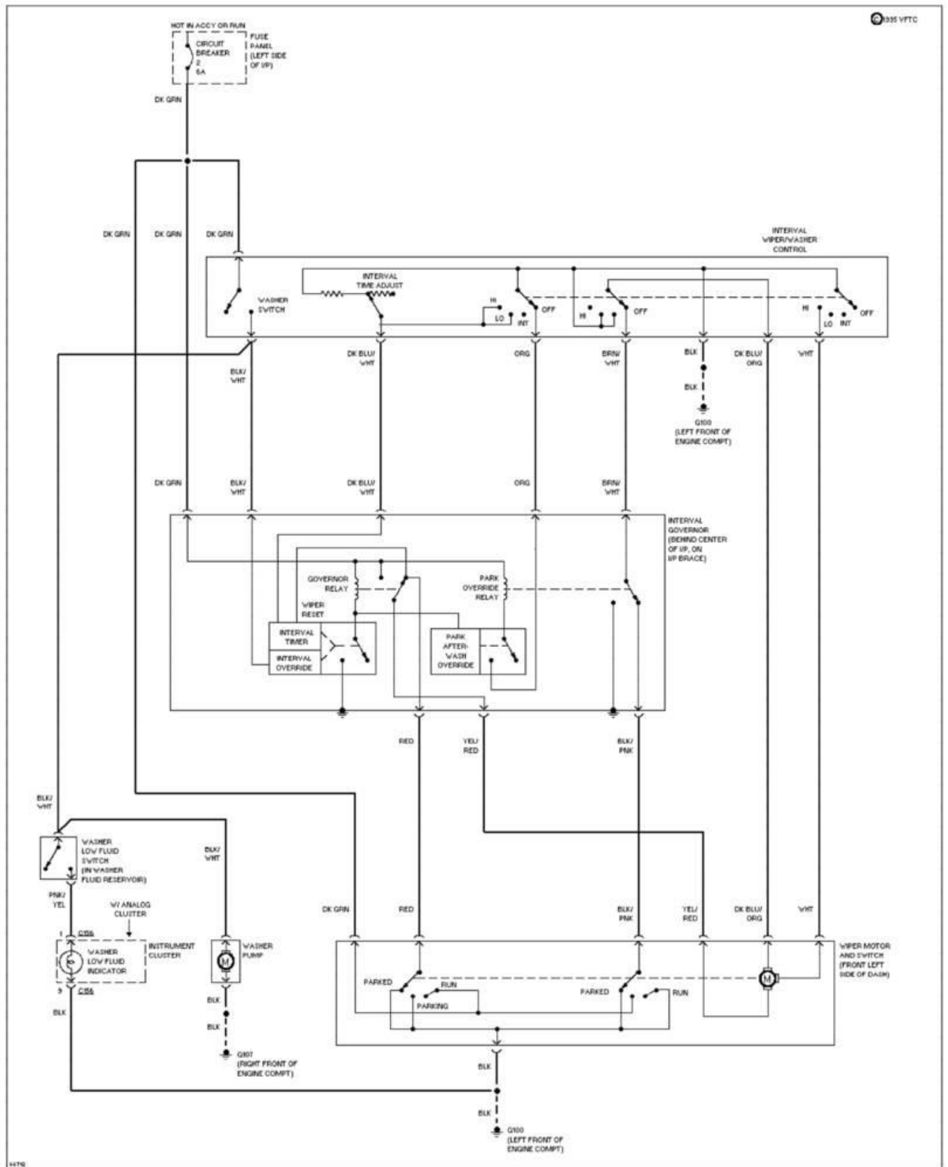
Fig. 27: Interval Wiper/Washer Circuit 1989 Ford Taurus LX
