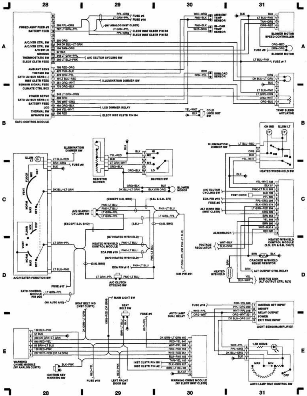
Fig. 8: A/C & Heater 1989 Ford Taurus LX
