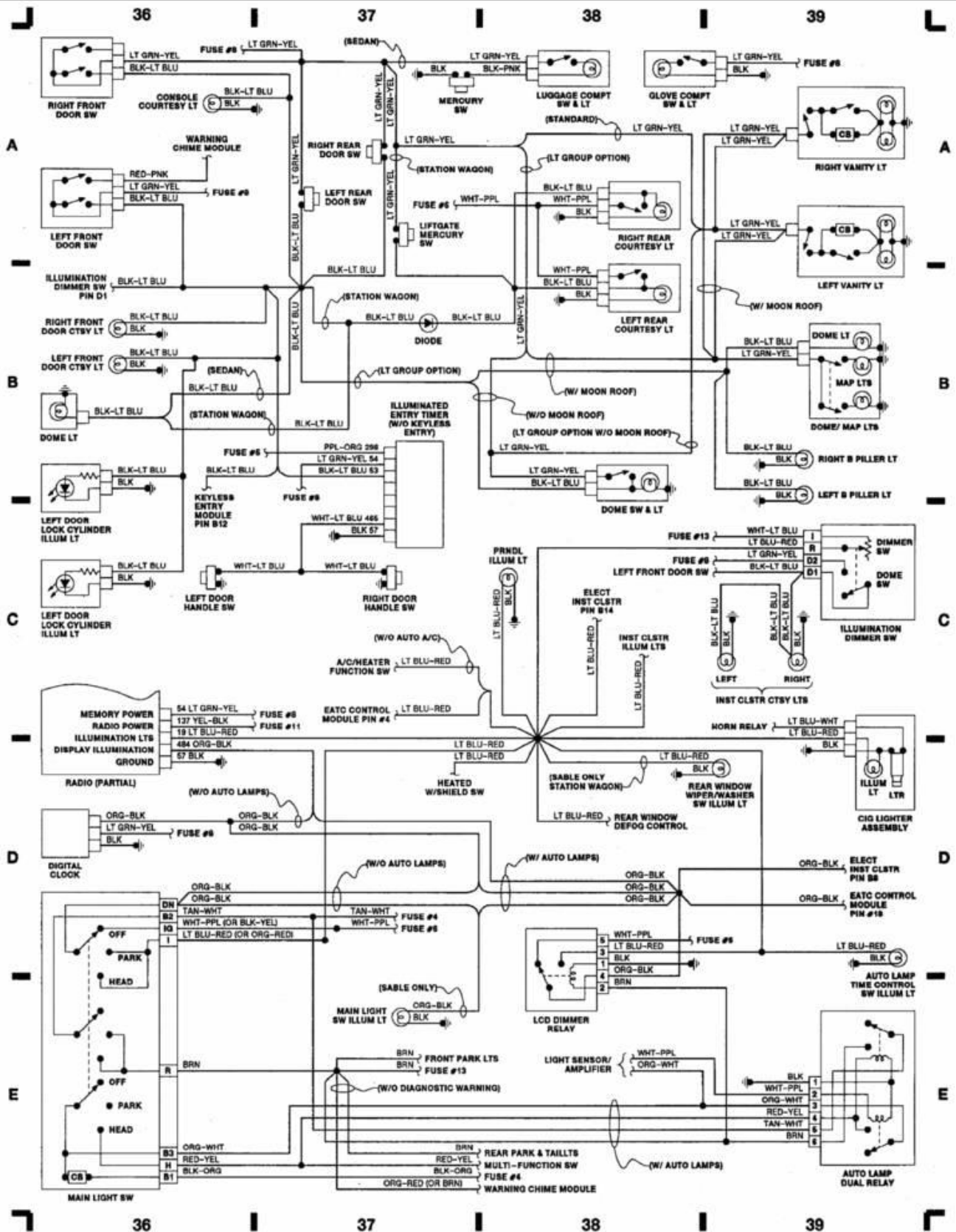
Fig. 10: Accessories 1989 Ford Taurus LX
