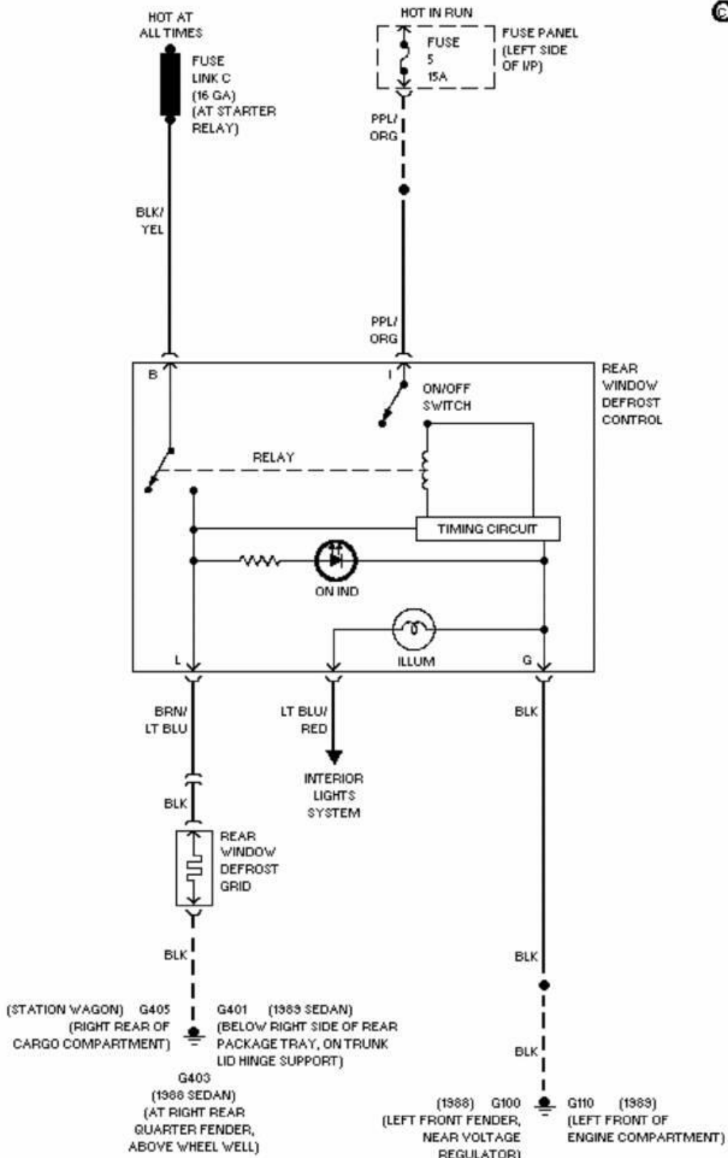
Fig. 5: Defogger Circuit 1989 Ford Taurus LX
