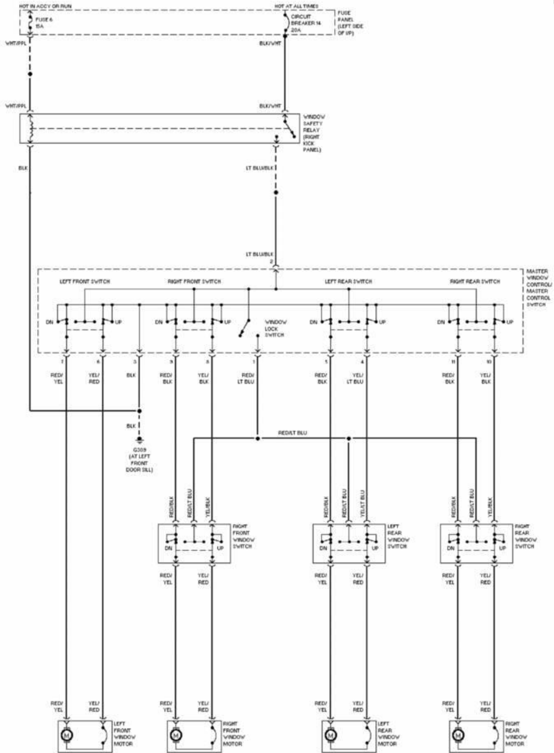
Fig. 13: Power Window Circuit 1989 Ford Taurus LX
