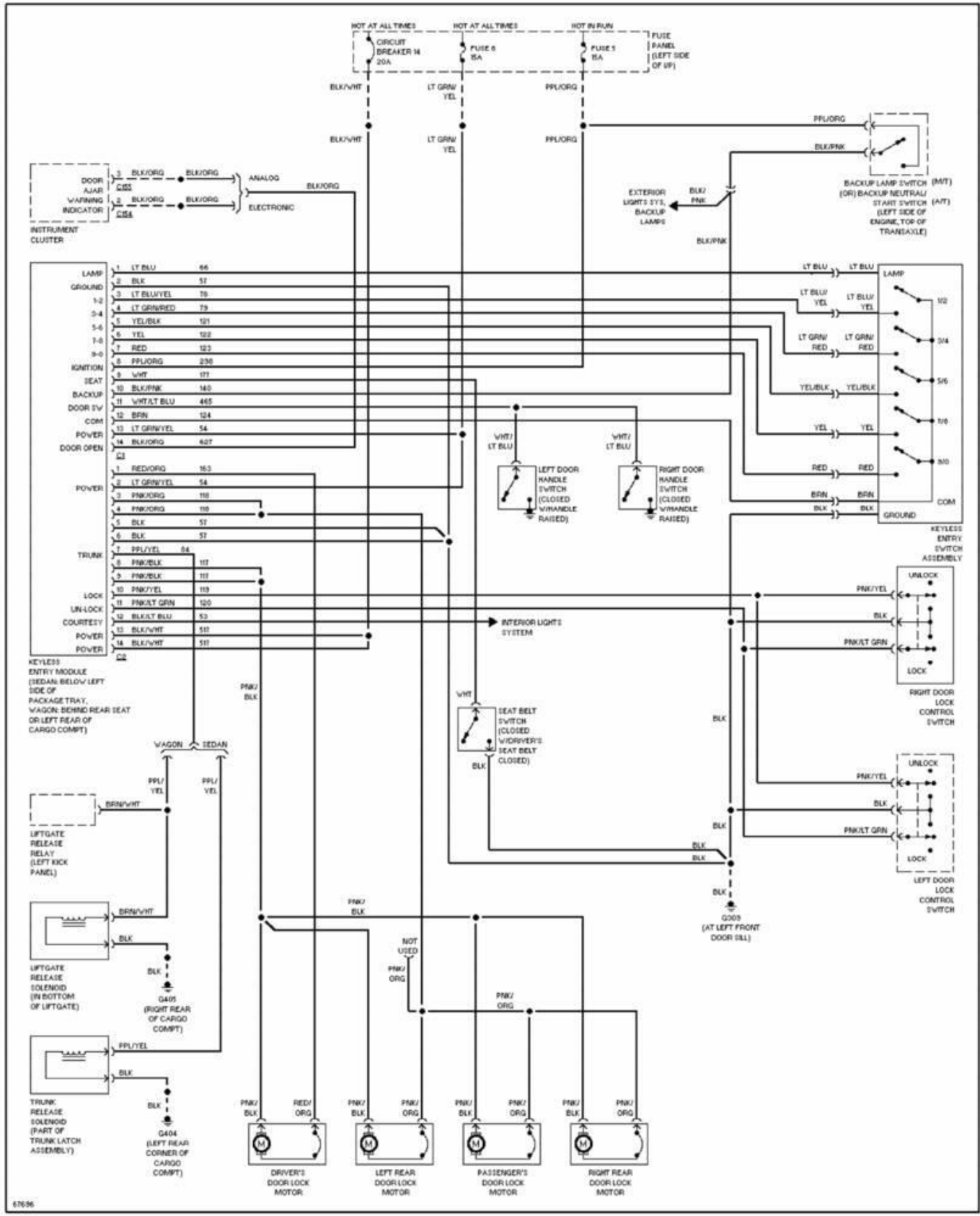
Fig. 9: Keyless Entry Circuit 1989 Ford Taurus LX
