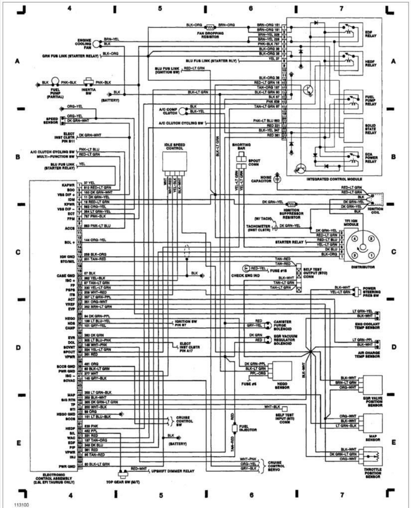
Fig. 2: Computer Engine Control (2.5L) 1989 Ford Taurus LX
