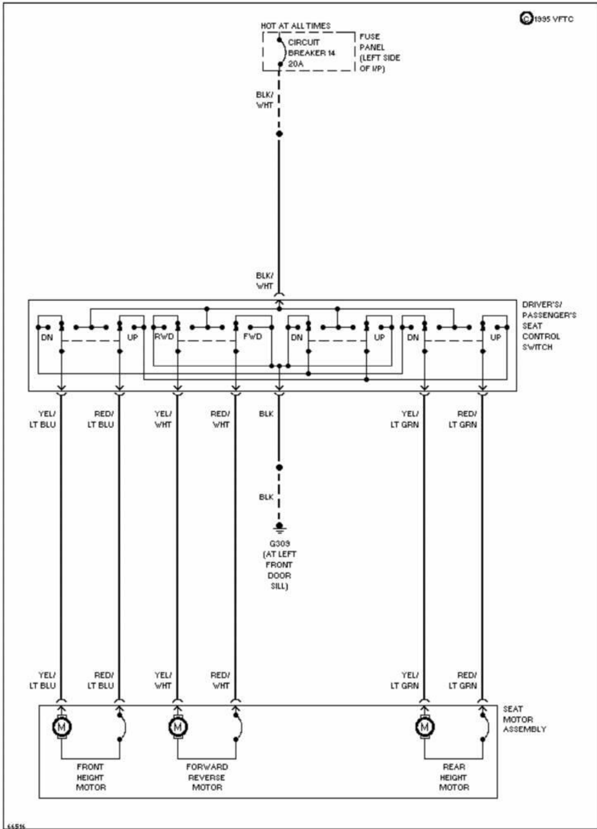
Fig. 12: Power Seat Circuit 1989 Ford Taurus LX
