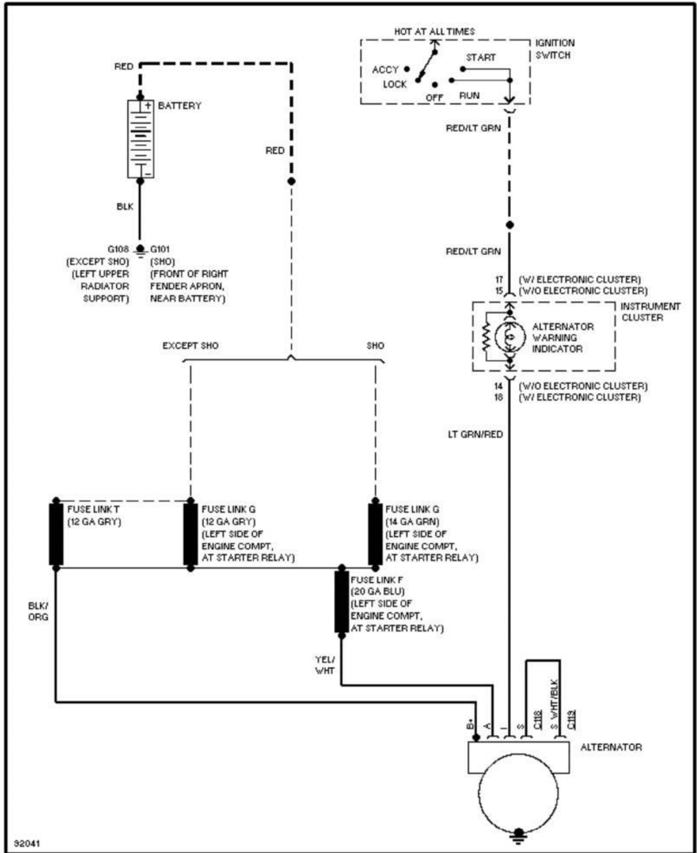
Fig. 18: Charging Circuit, W/O Heated Windshield 1991 Ford Taurus LX
