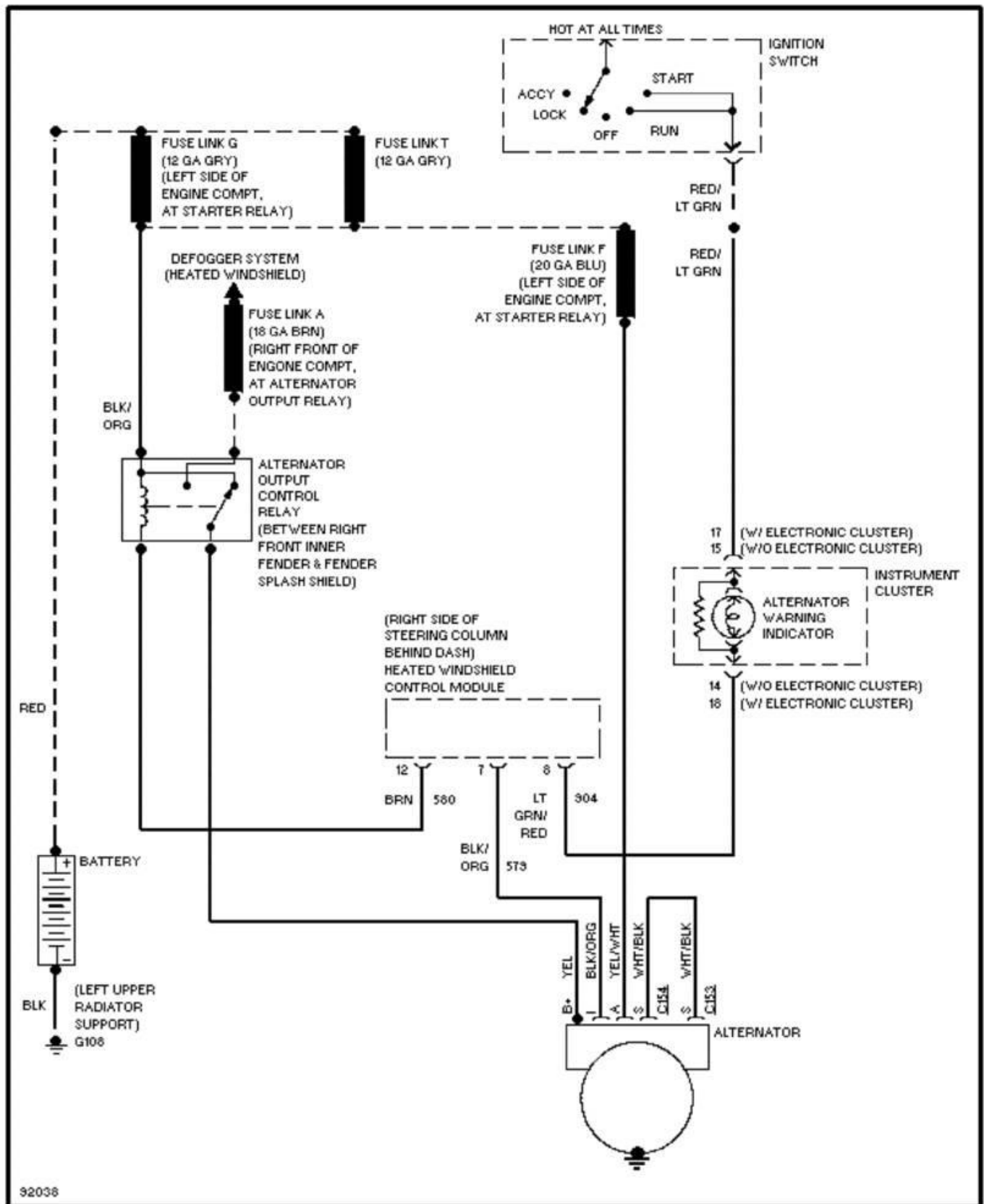
Fig. 17: Charging Circuit, W/ Heated Windshield 1991 Ford Taurus LX
