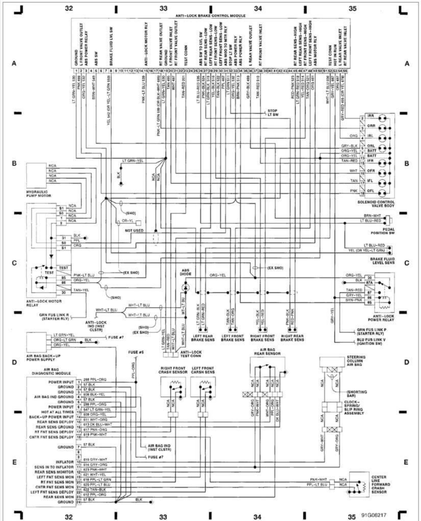
Fig. 9: ABS, Air Bag (Grid 32-35) 1991 Ford Taurus LX
