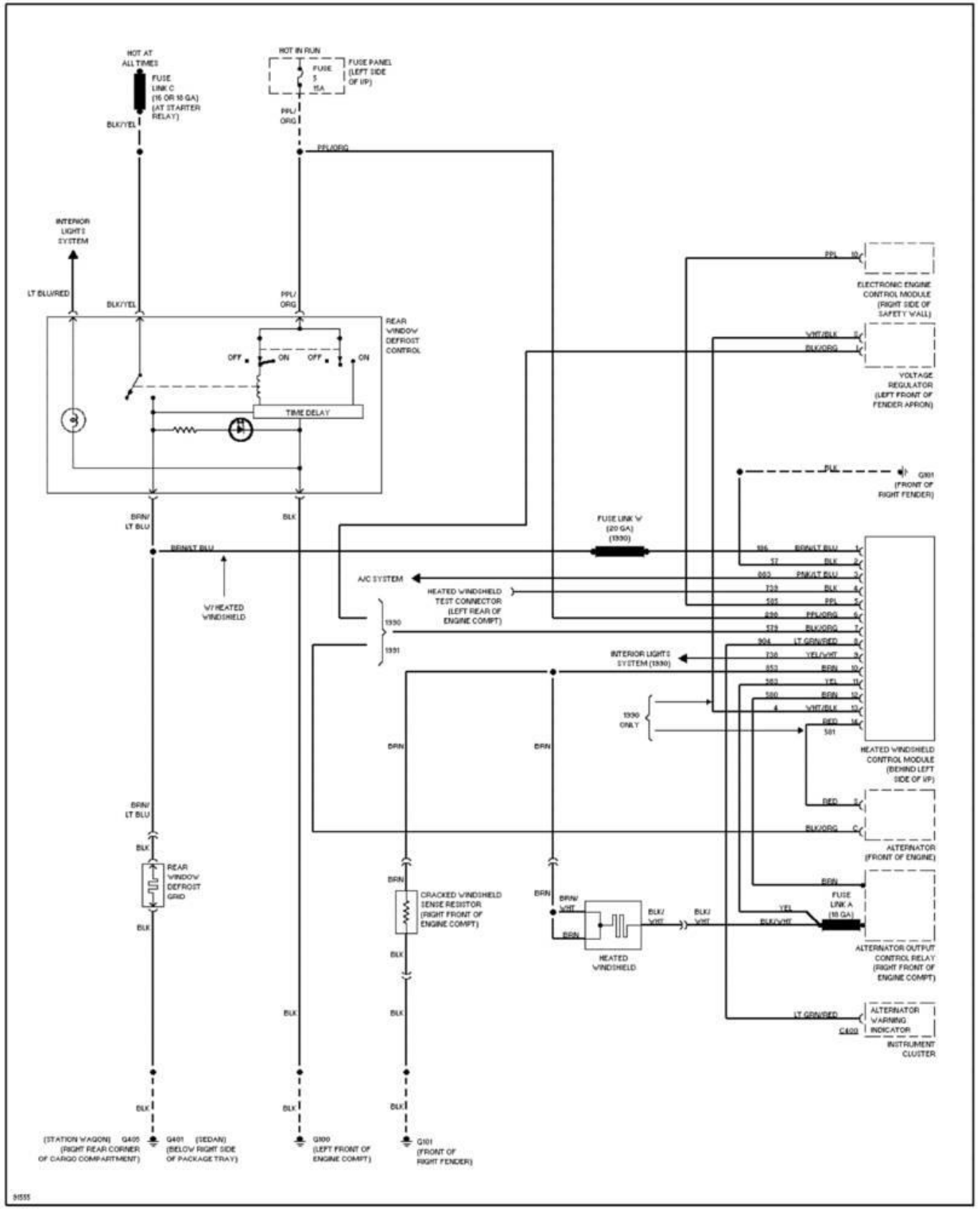
Fig. 5: Defogger Circuit 1991 Ford Taurus LX
