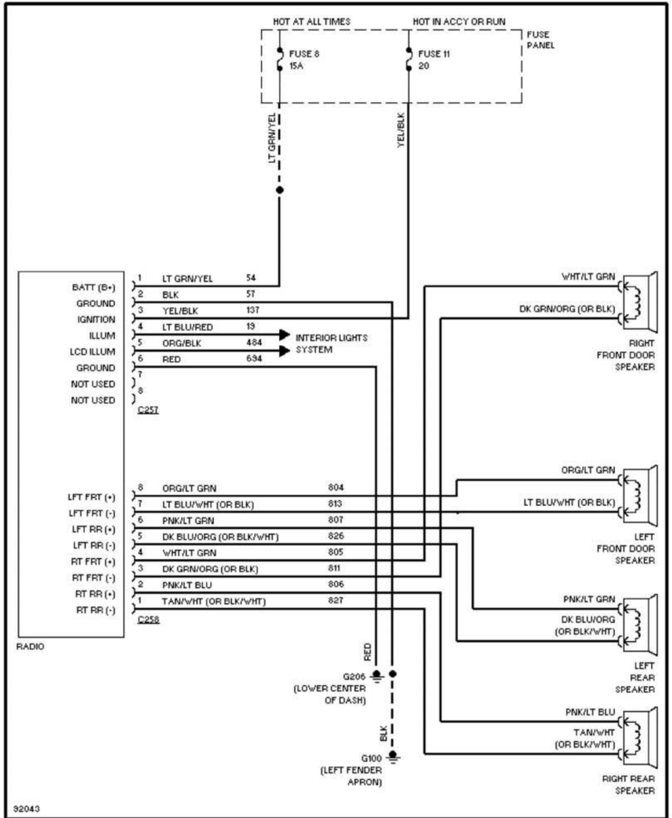
Fig. 14: Radio Circuits 1991 Ford Taurus LX
