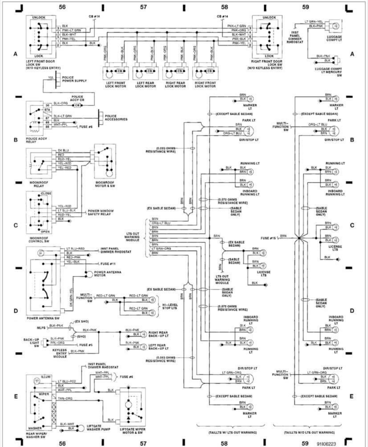
Fig. 15: Power Doors (W/O Keyless), Taillights (Grid 56-59) 1991 Ford Taurus LX
