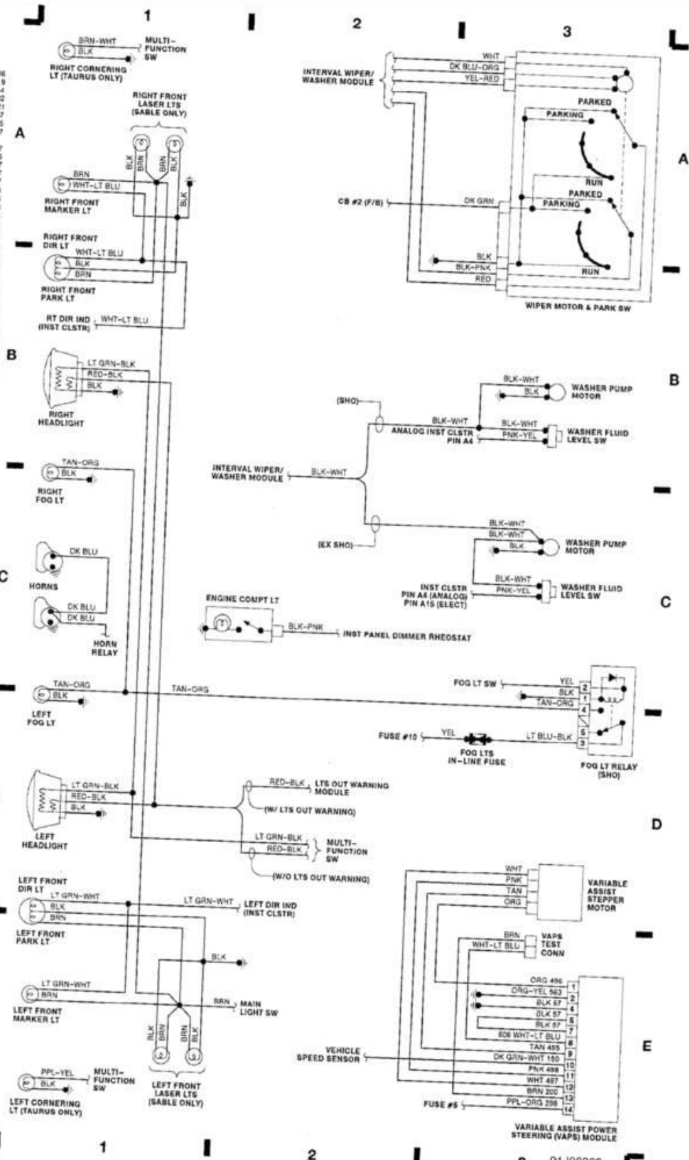
Fig. 1: Headlights & Washer/Wiper, VAPS (Grid 1-3) 1991 Ford Taurus LX
