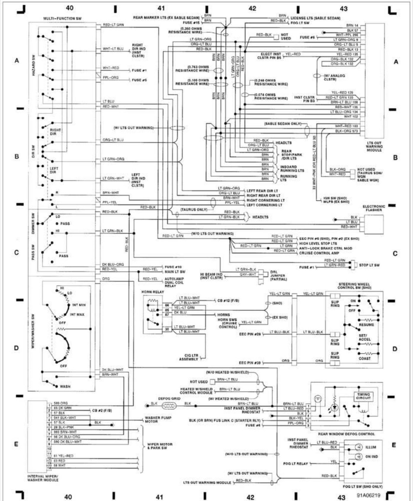
Fig. 11: Multi-Function Sw, Steering Wheel Ctrl Sw (Grid 40-43) 1991 Ford Taurus LX
