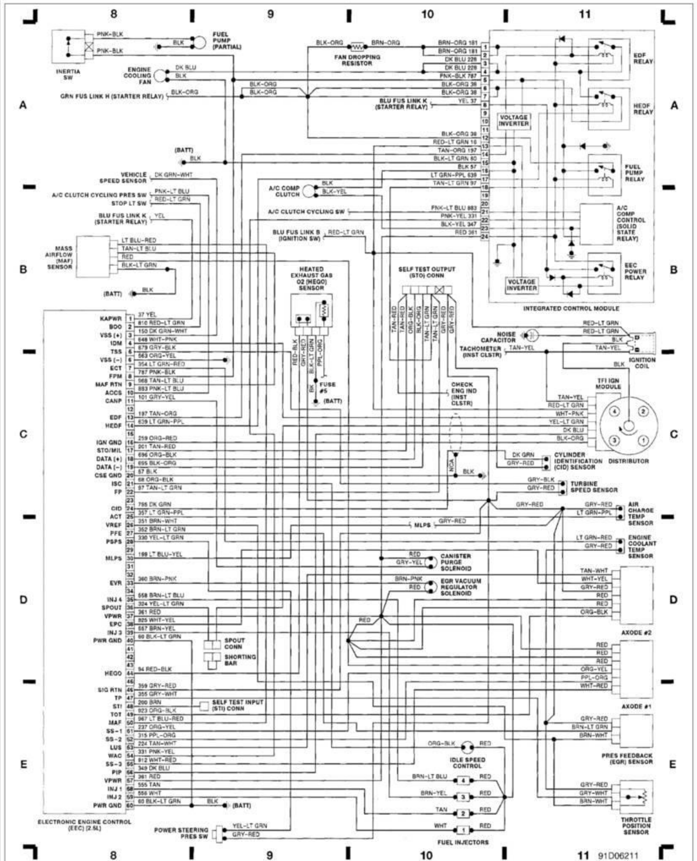
Fig. 3: Elect Engine Control (2.5L) (Grid 8-11) 1991 Ford Taurus LX
