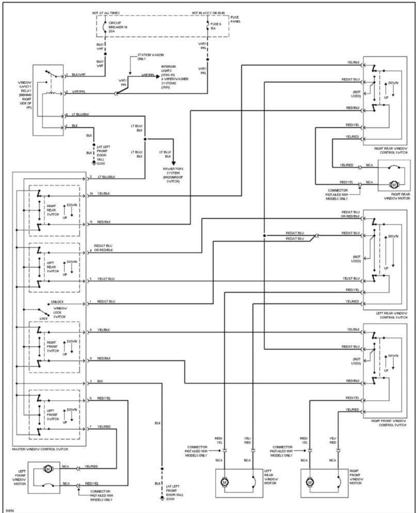
Fig. 13: Power Window Circuit 1991 Ford Taurus LX
