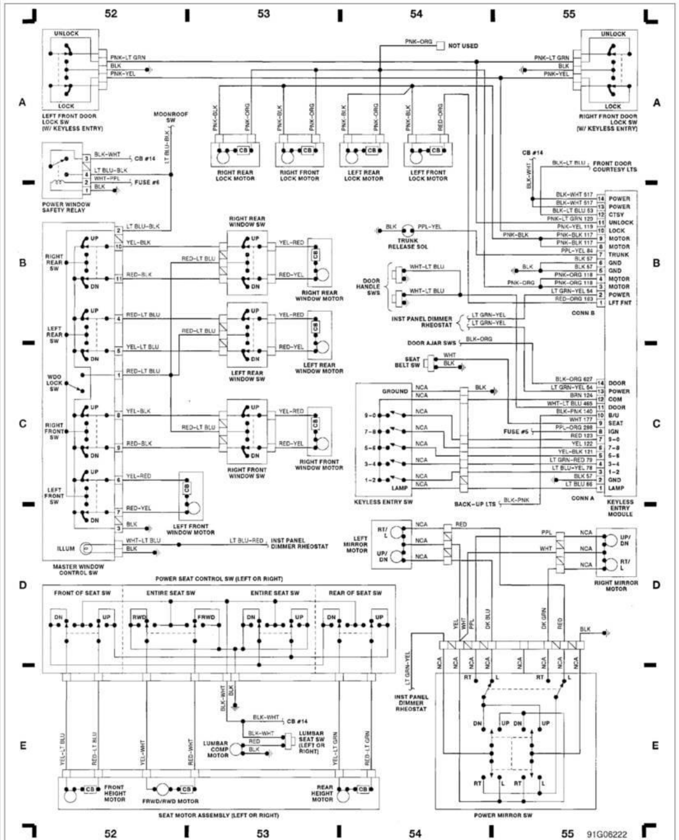
Fig. 14: Keyless Entry, Power Seat/Window (Grid 52-55) 1991 Ford Taurus LX
