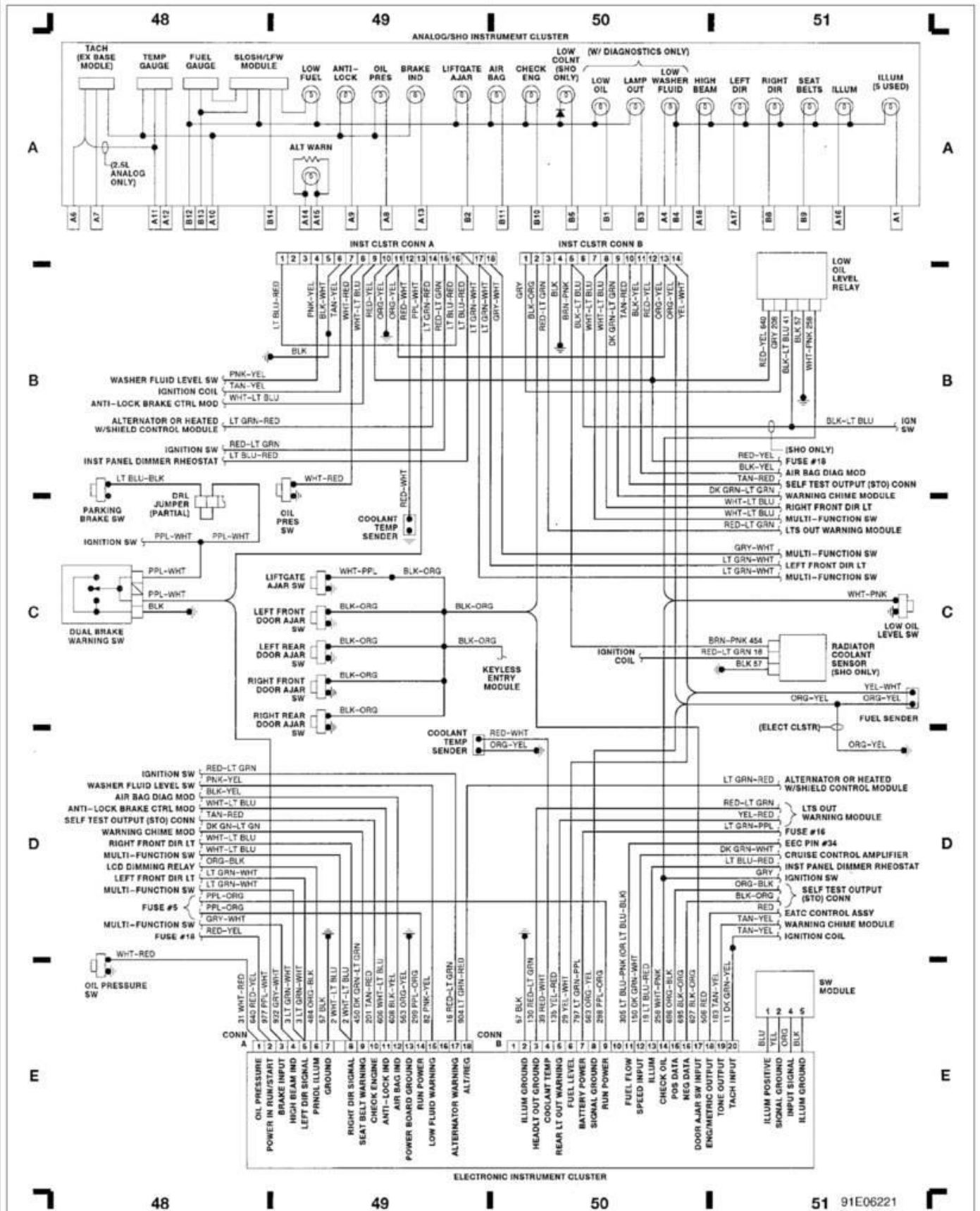
Fig. 13: Instrument Clusters (Grid 48-51) 1991 Ford Taurus LX
