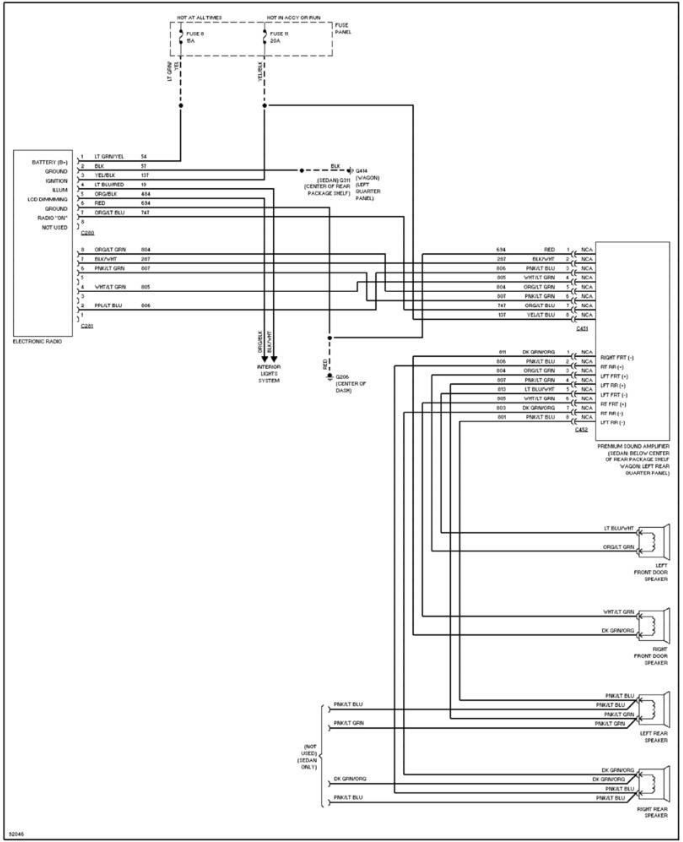
Fig. 16: Radio Circuits, Premium Radio 1991 Ford Taurus LX
