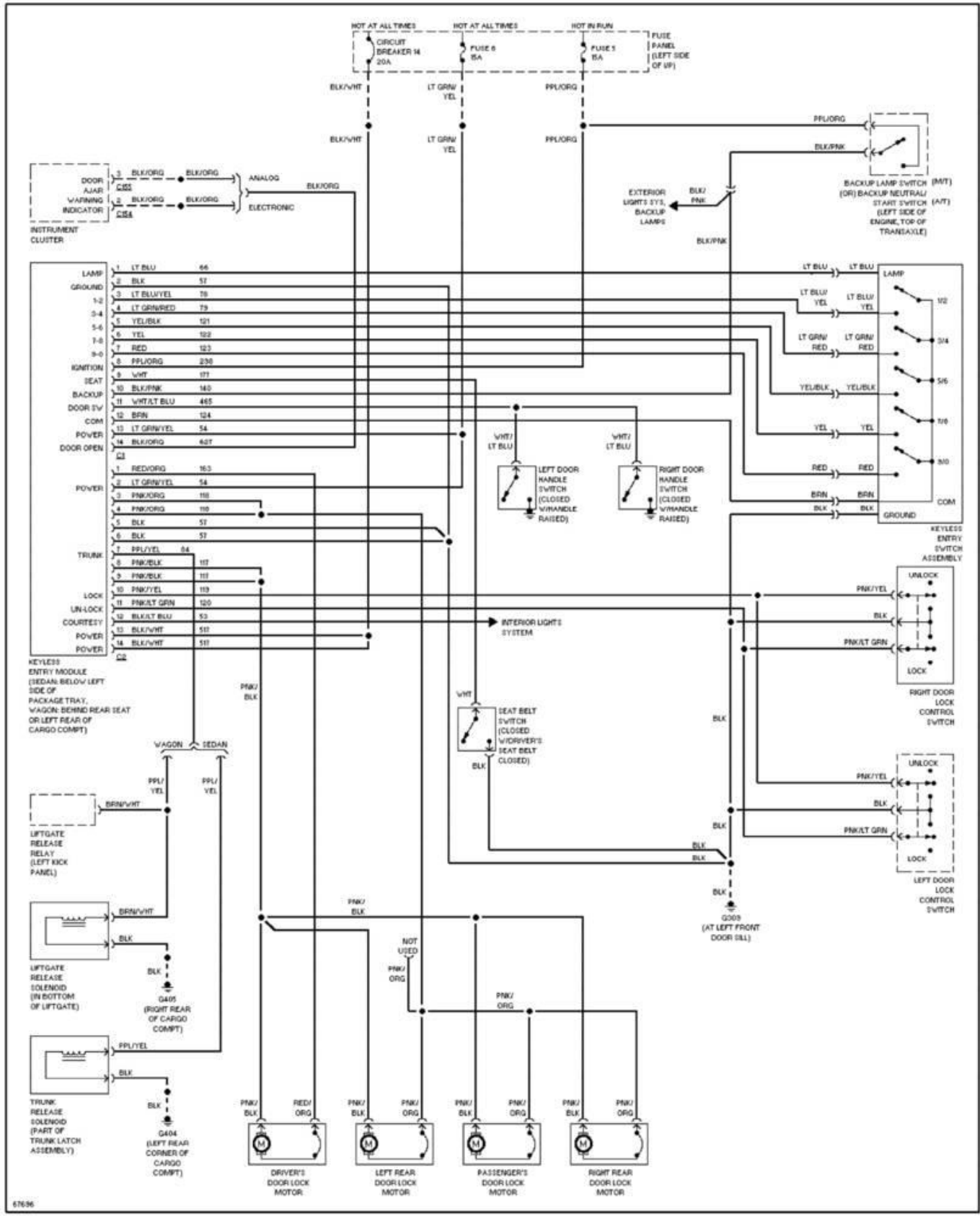
Fig. 9: Keyless Entry Circuit 1991 Ford Taurus LX
