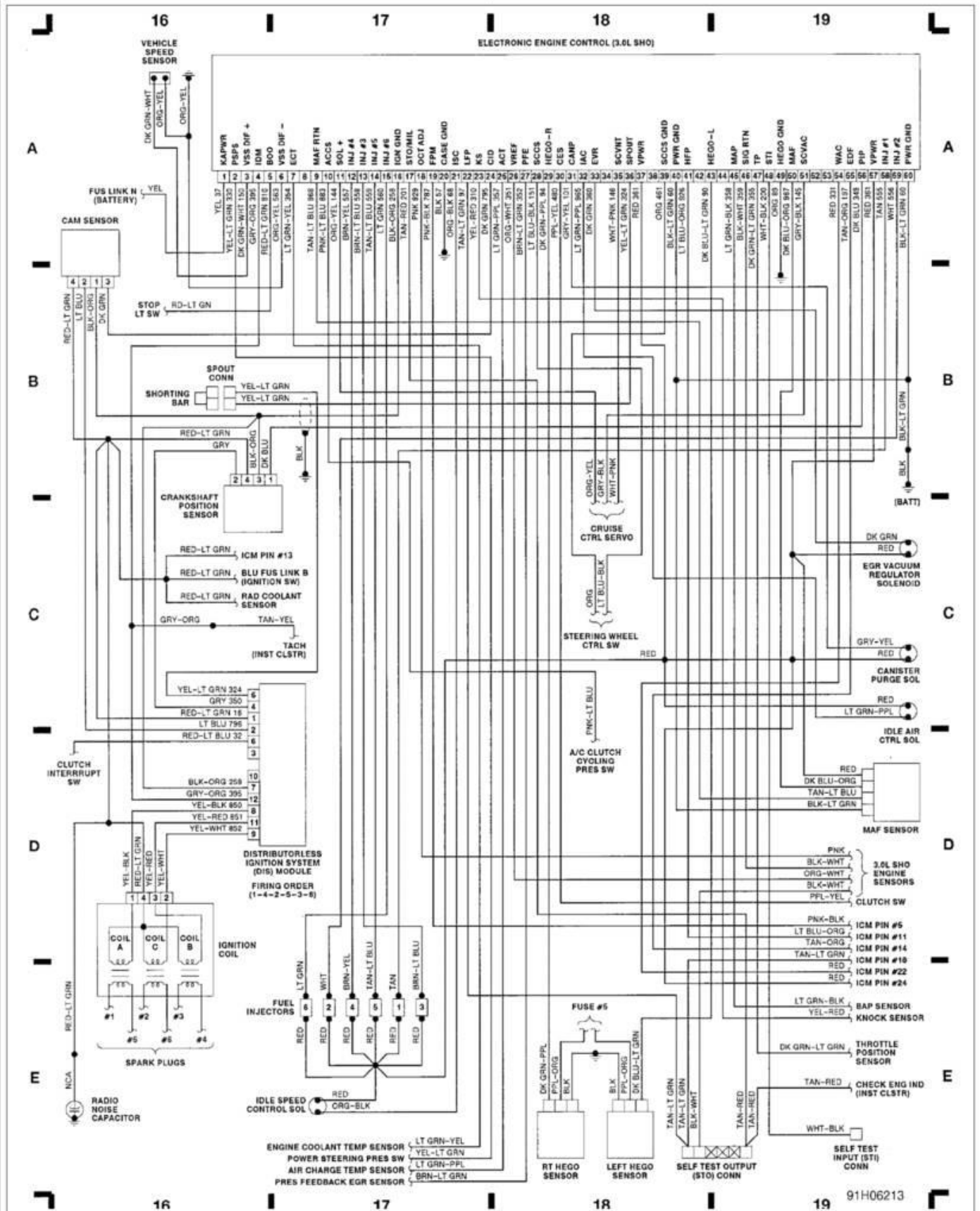
Fig. 5: Elect Engine Control (3.0L SHO) (Grid 16-19) 1991 Ford Taurus LX
