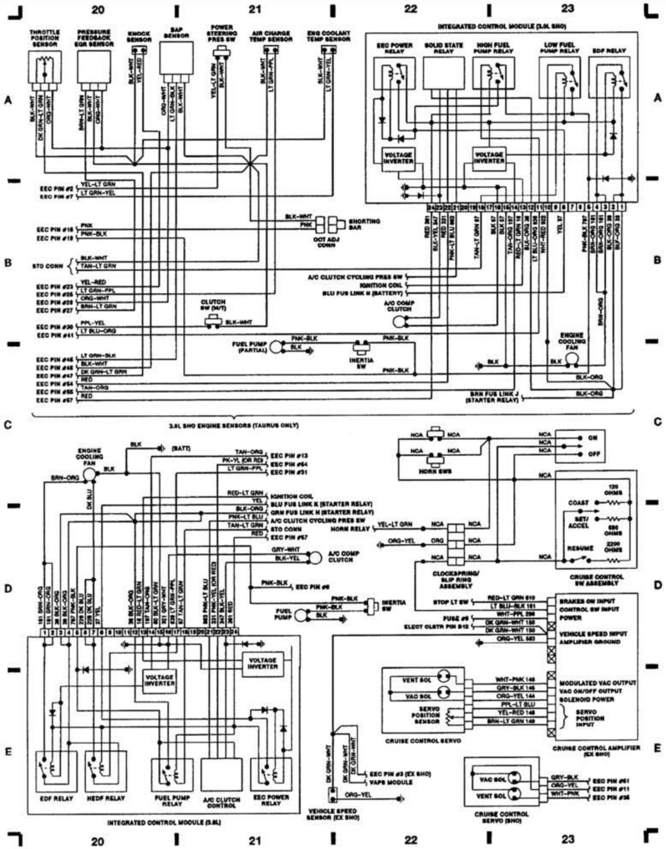
Fig. 6: Cruise Control, ICM (3.0L SHO/3.8L) (Grid 20-23) 1991 Ford Taurus LX
