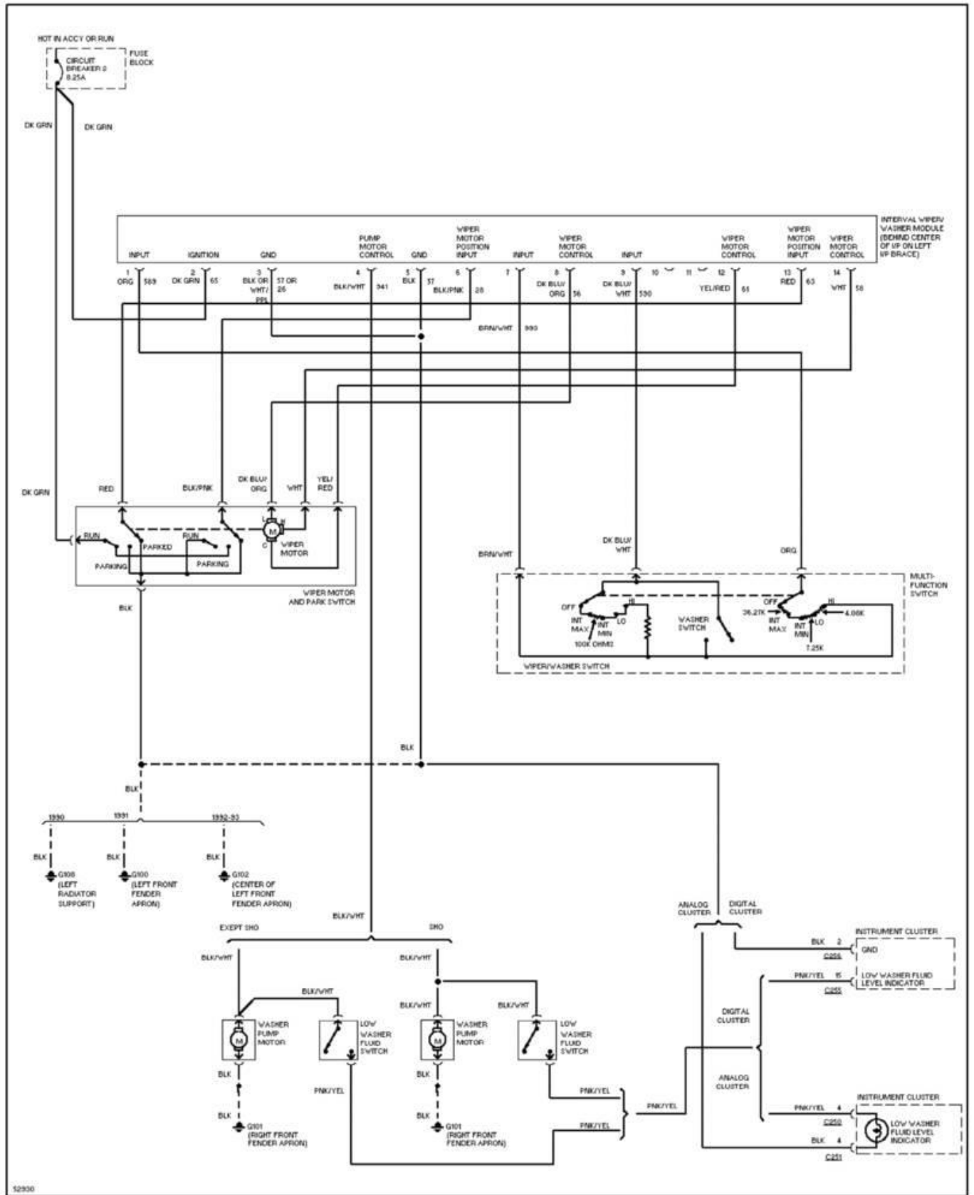
Fig. 21: Interval Wiper/Washer Circuit 1991 Ford Taurus LX
