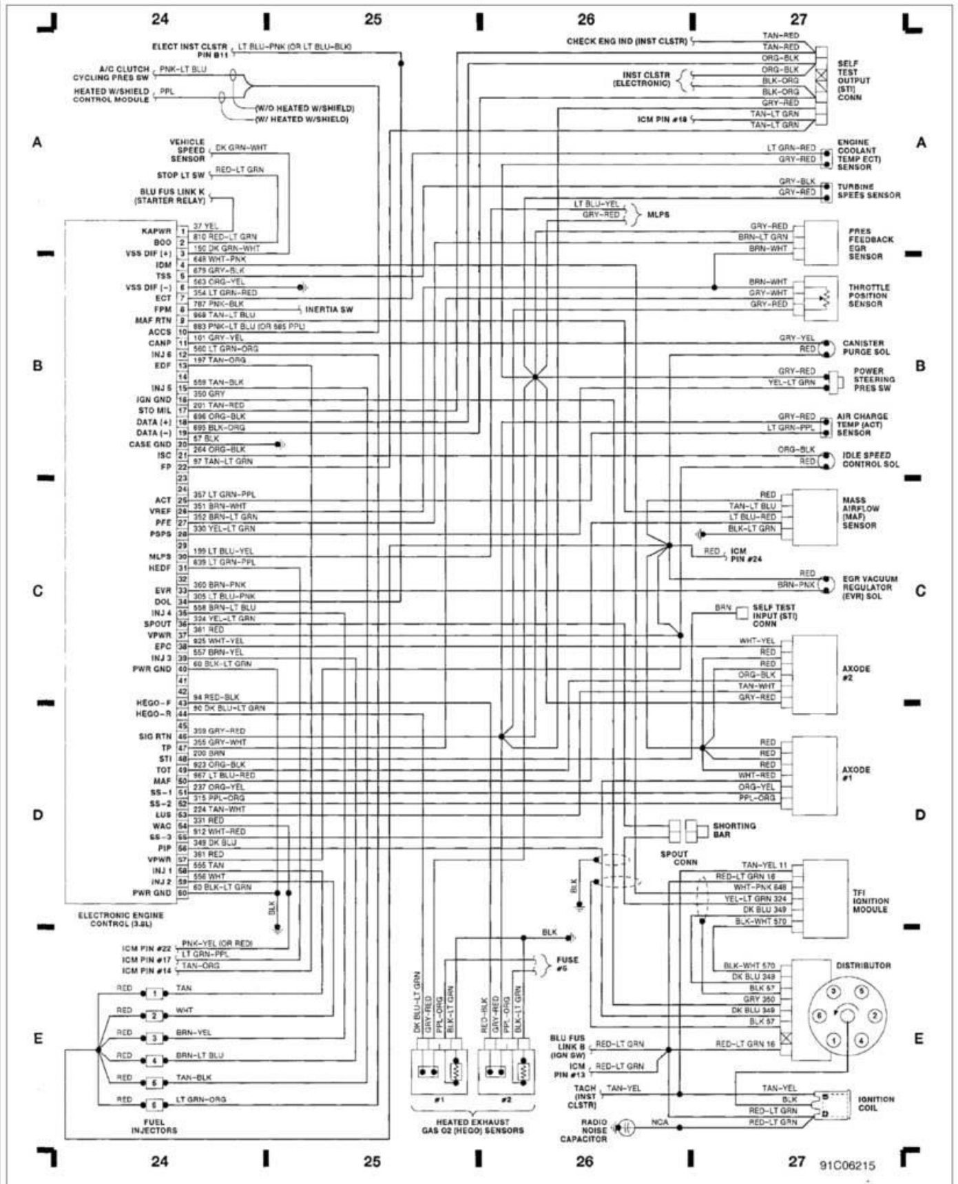
Fig. 7: Elect Engine Control (3.8L) (Grid 24-27) 1991 Ford Taurus LX
