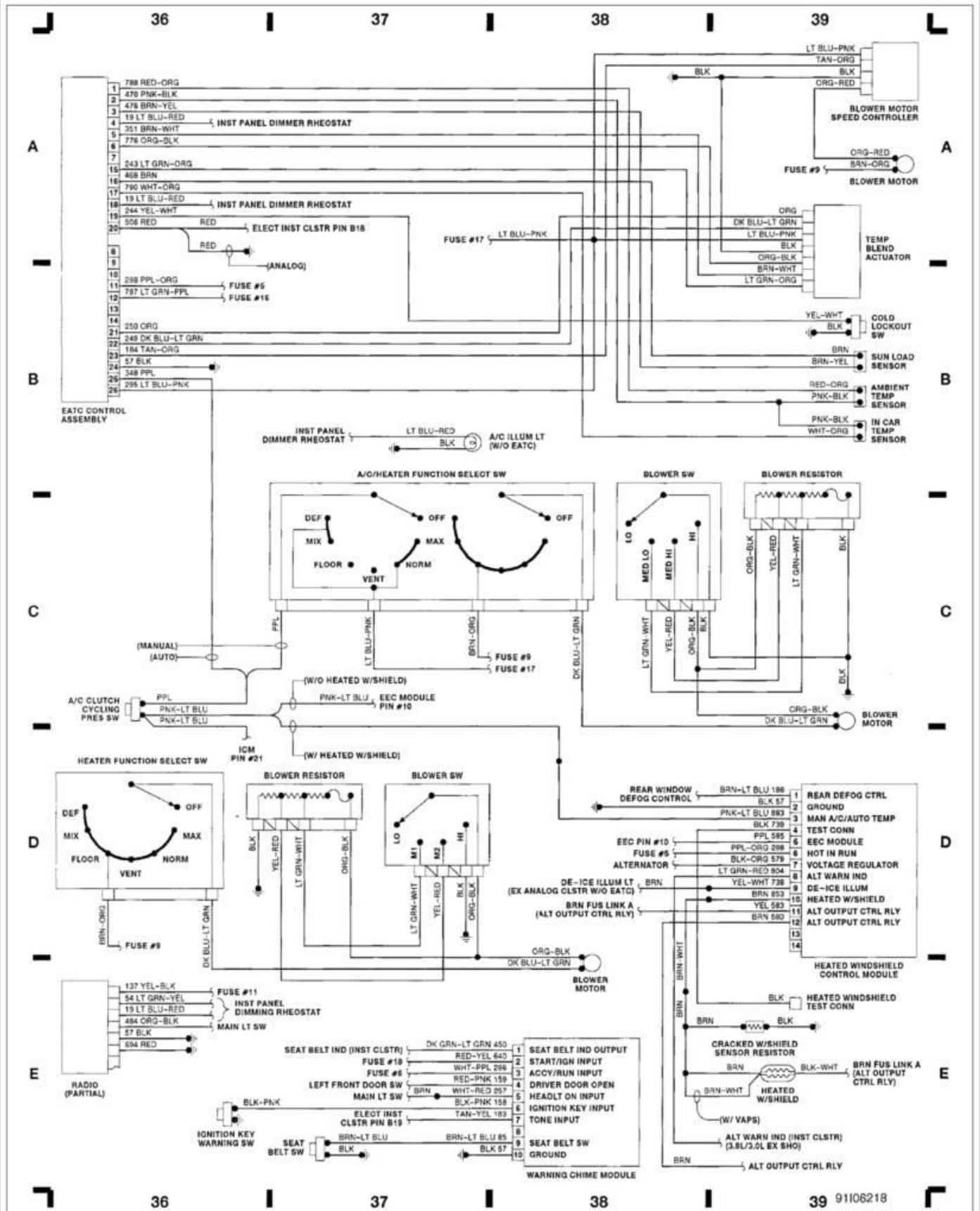
Fig. 10: EATC, A/C/Heater (Grid 36-39) 1991 Ford Taurus LX
