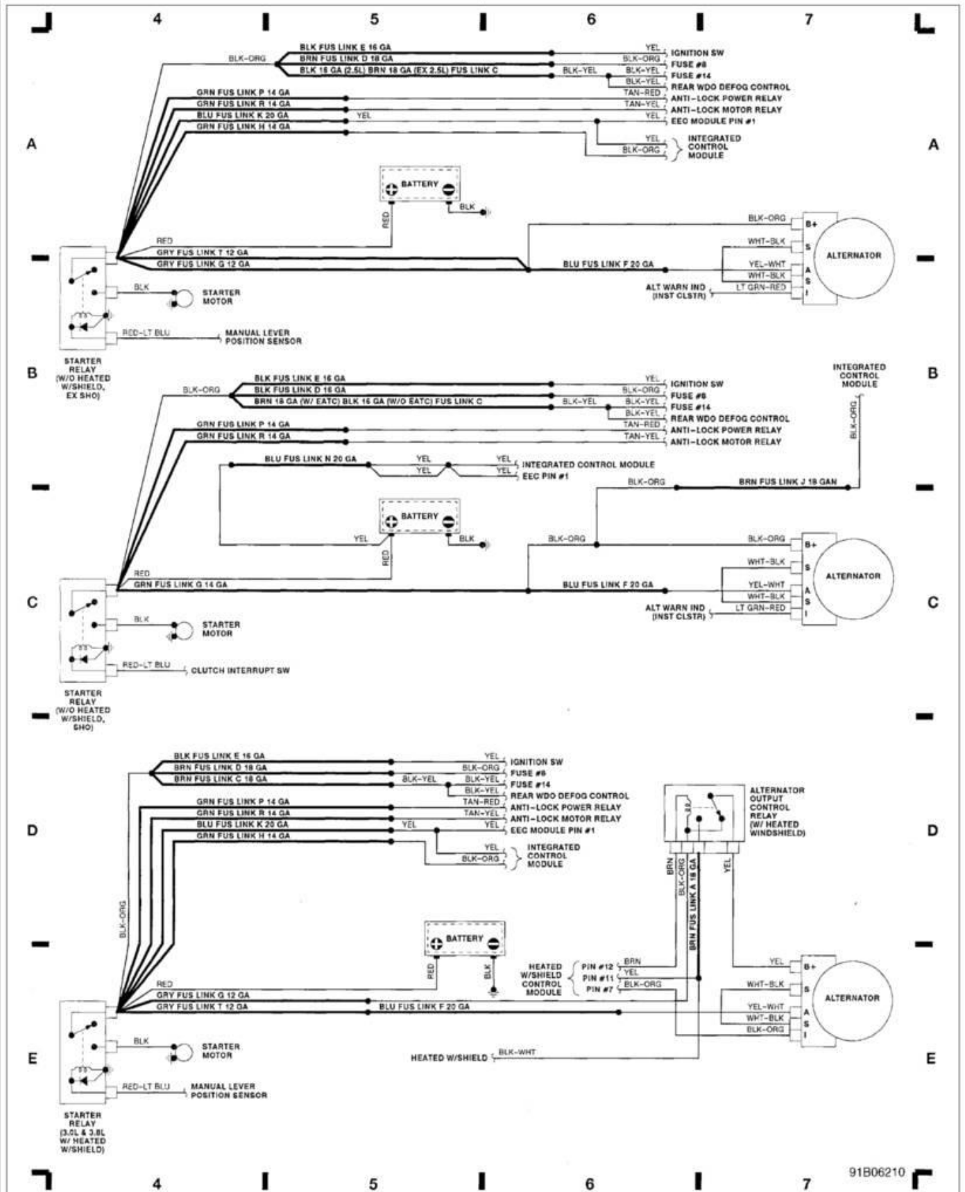
Fig. 2: Engine Compartment (Grid 4-7) 1991 Ford Taurus LX
