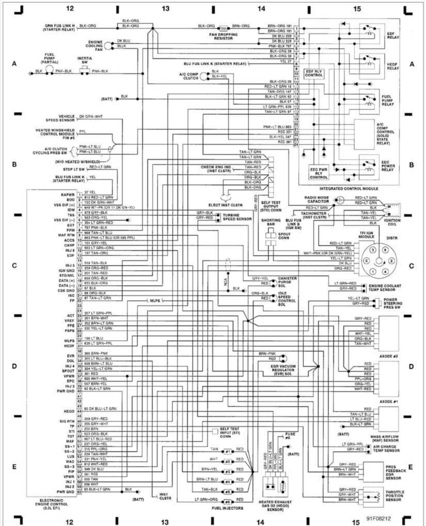
Fig. 4: Elect Engine Control (3.0L EFI) (Grid 12-15) 1991 Ford Taurus LX
