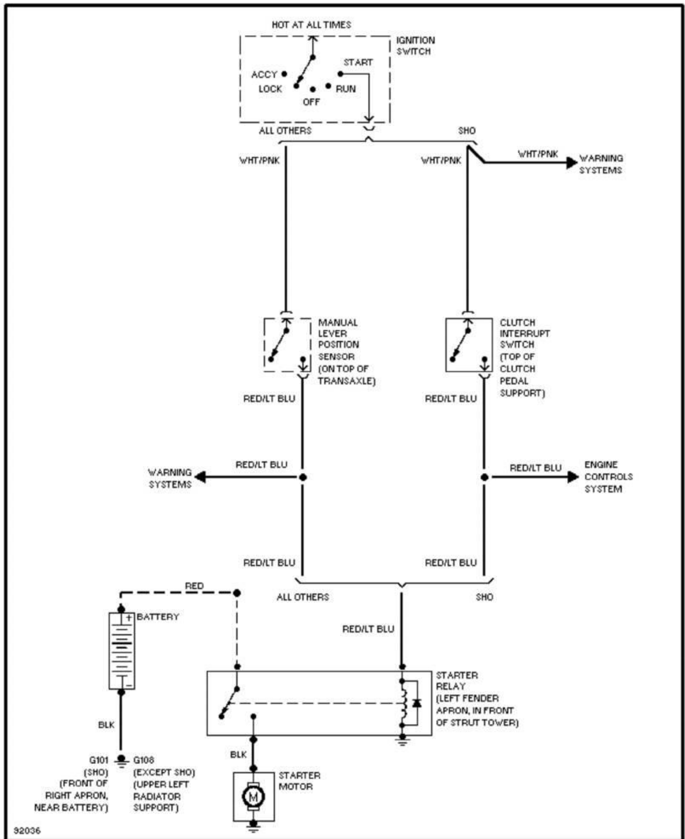
Fig. 19: Starting Circuit 1991 Ford Taurus LX
