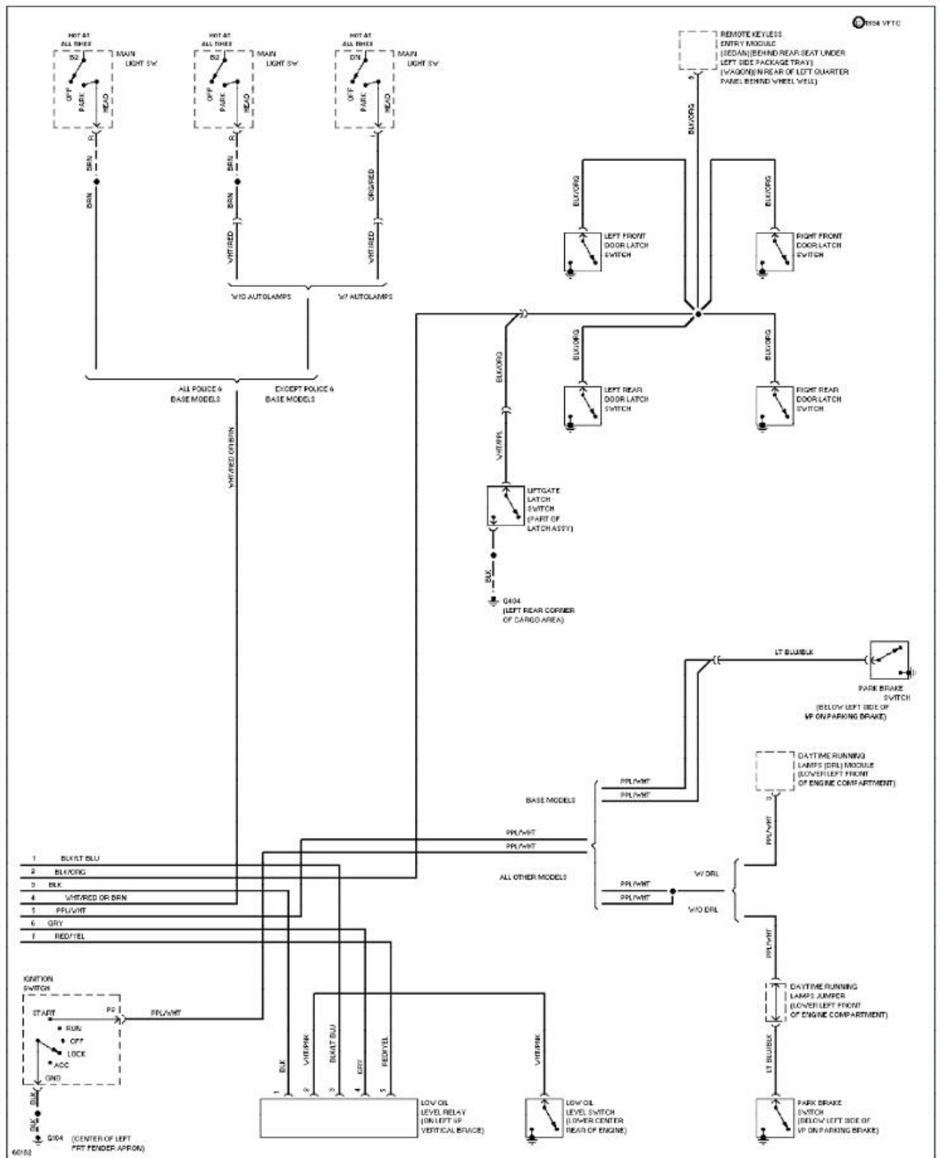
Fig. 44: 3.0L Flex Fuel, Analog Cluster Circuit (2 of 2) 1994 Ford Taurus LX
