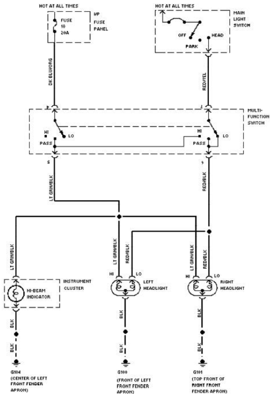
Fig. 39: Headlamps Circuit, W/O DRL 1994 Ford Taurus LX
