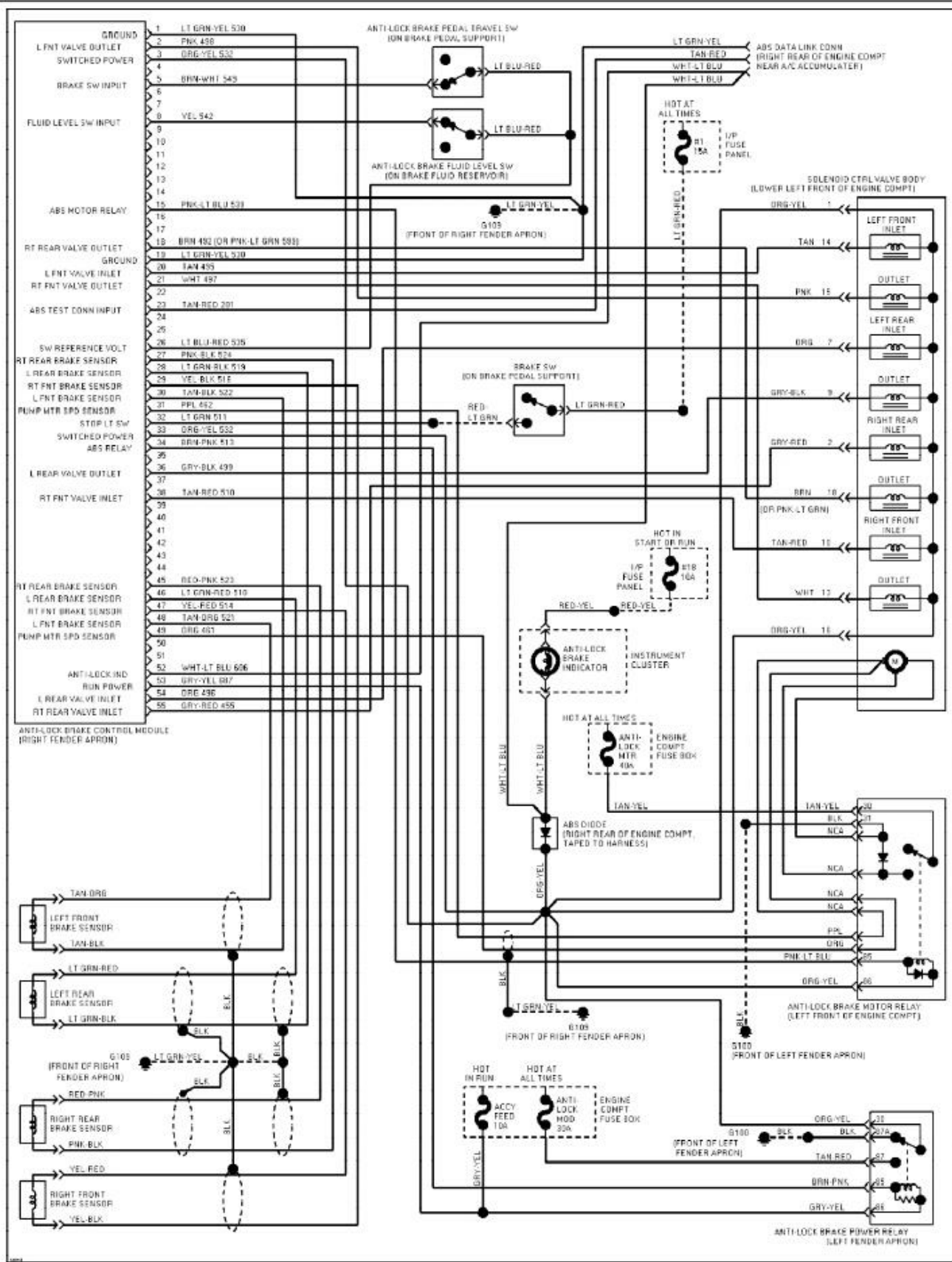
Fig. 3: 3.0L, Anti-lock Brake Circuits 1994 Ford Taurus LX
