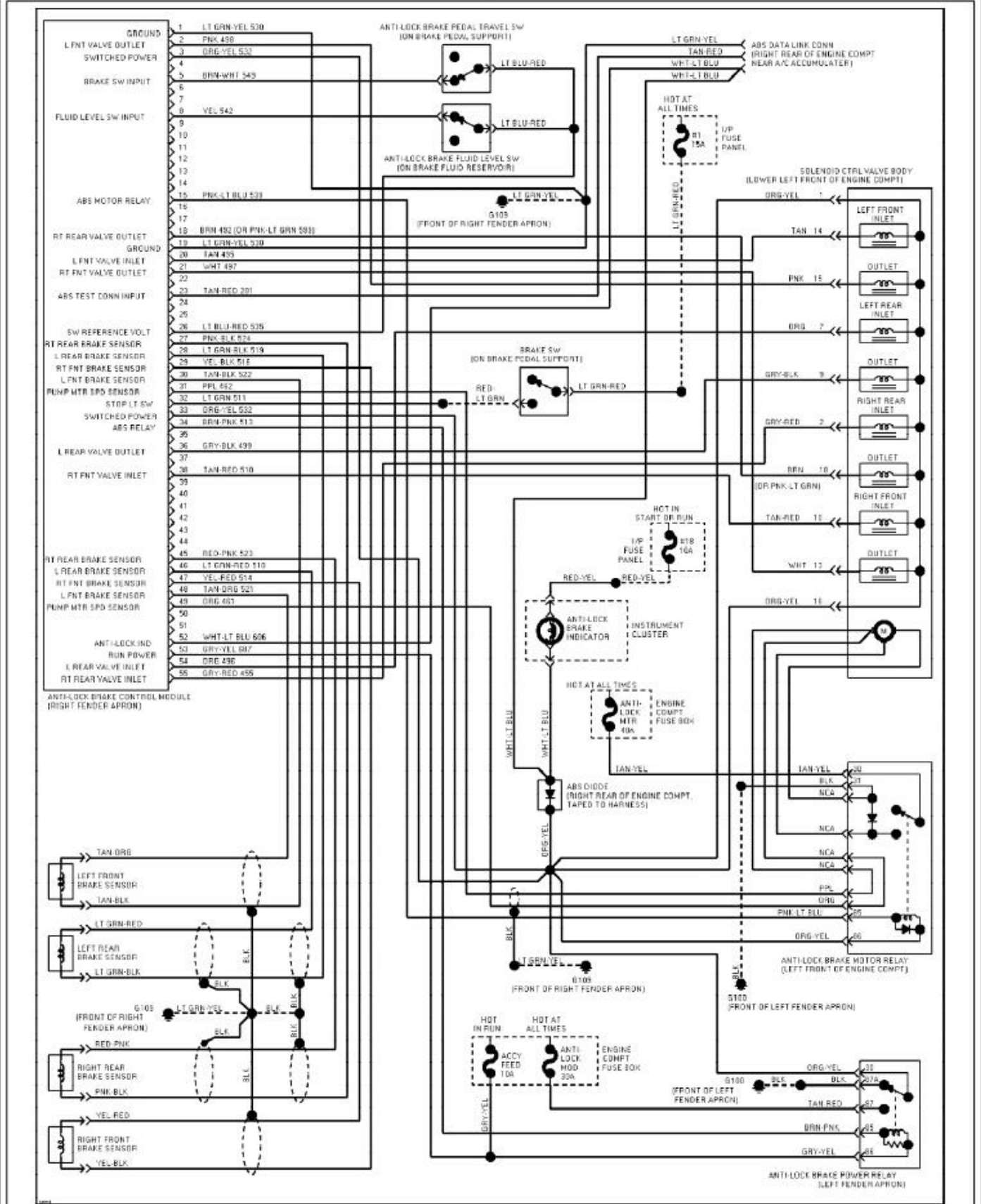
Fig. 1: 3.0L Flex Fuel, Anti-lock Brake Circuits 1994 Ford Taurus LX
