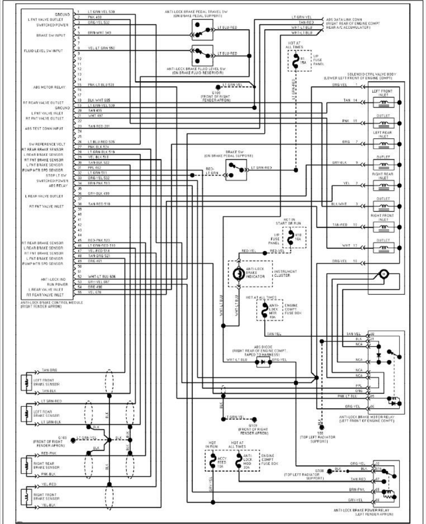
Fig. 2: 3.0L SHO, Anti-lock Brake Circuits 1994 Ford Taurus LX
