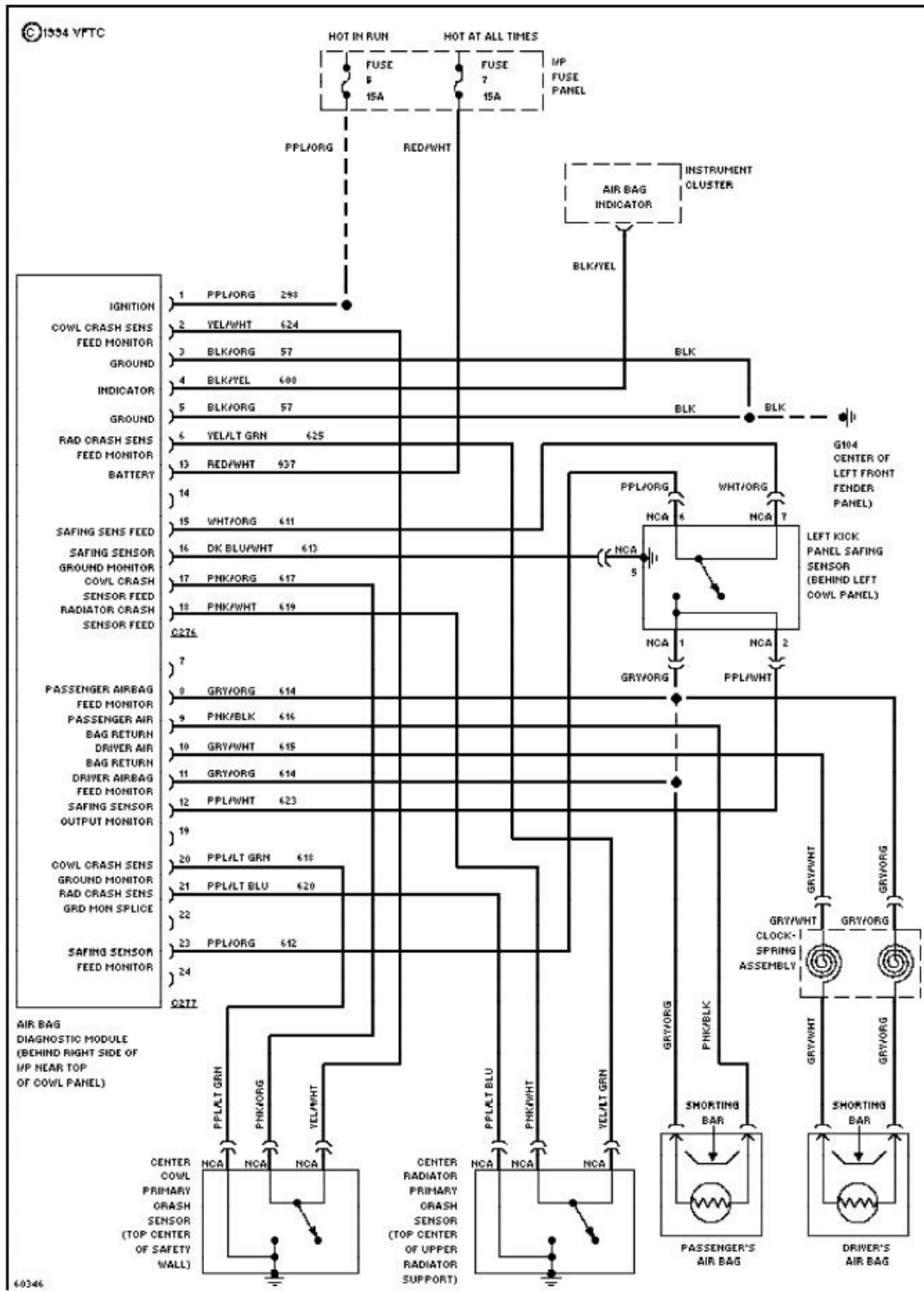
Fig. 99: Supplemental Restraint Circuit 1994 Ford Taurus LX
