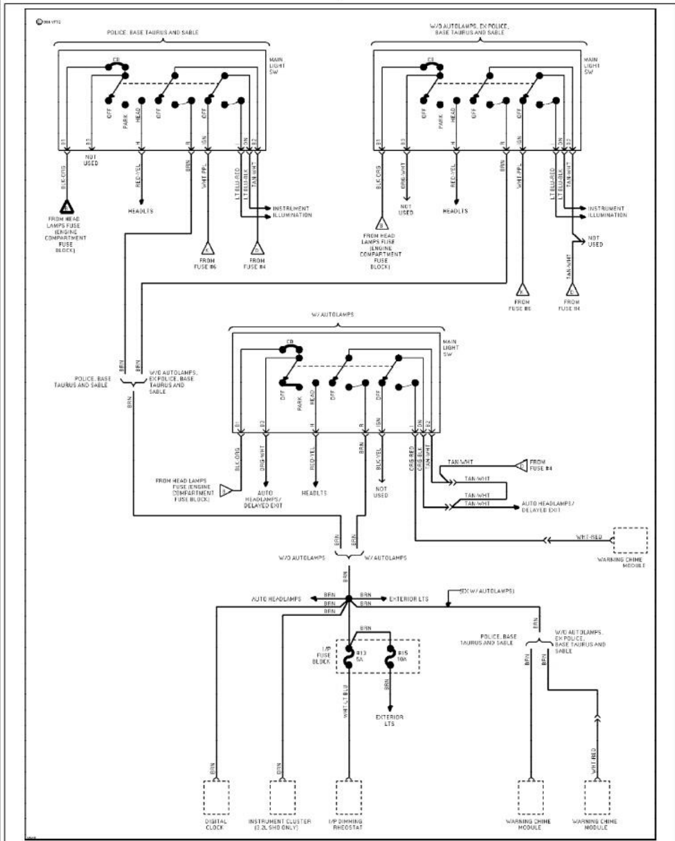
Fig. 74: Power Distribution Circuit (6 of 6) 1994 Ford Taurus LX
