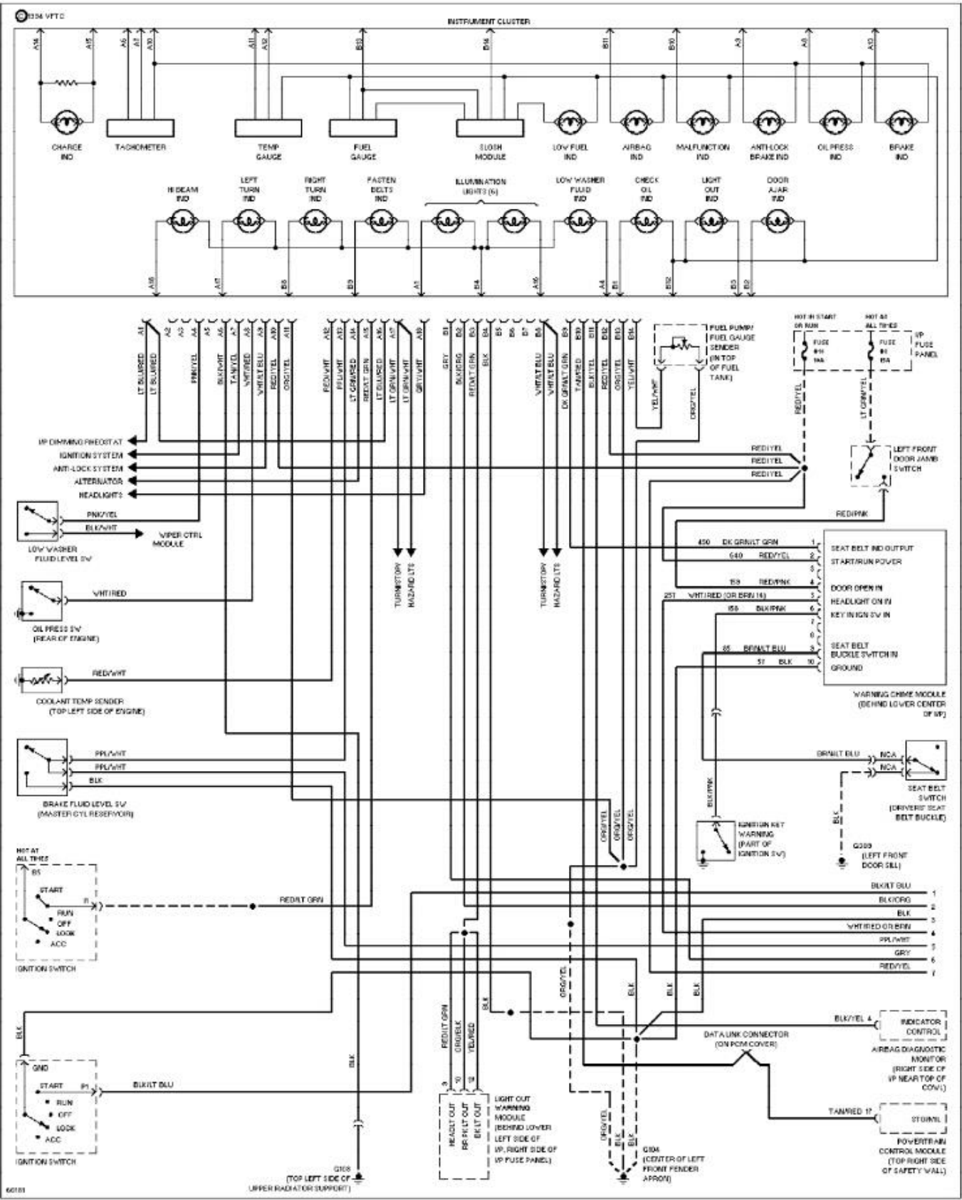
Fig. 59: 3.8L, Analog Cluster Circuit (1 of 2) 1994 Ford Taurus LX
