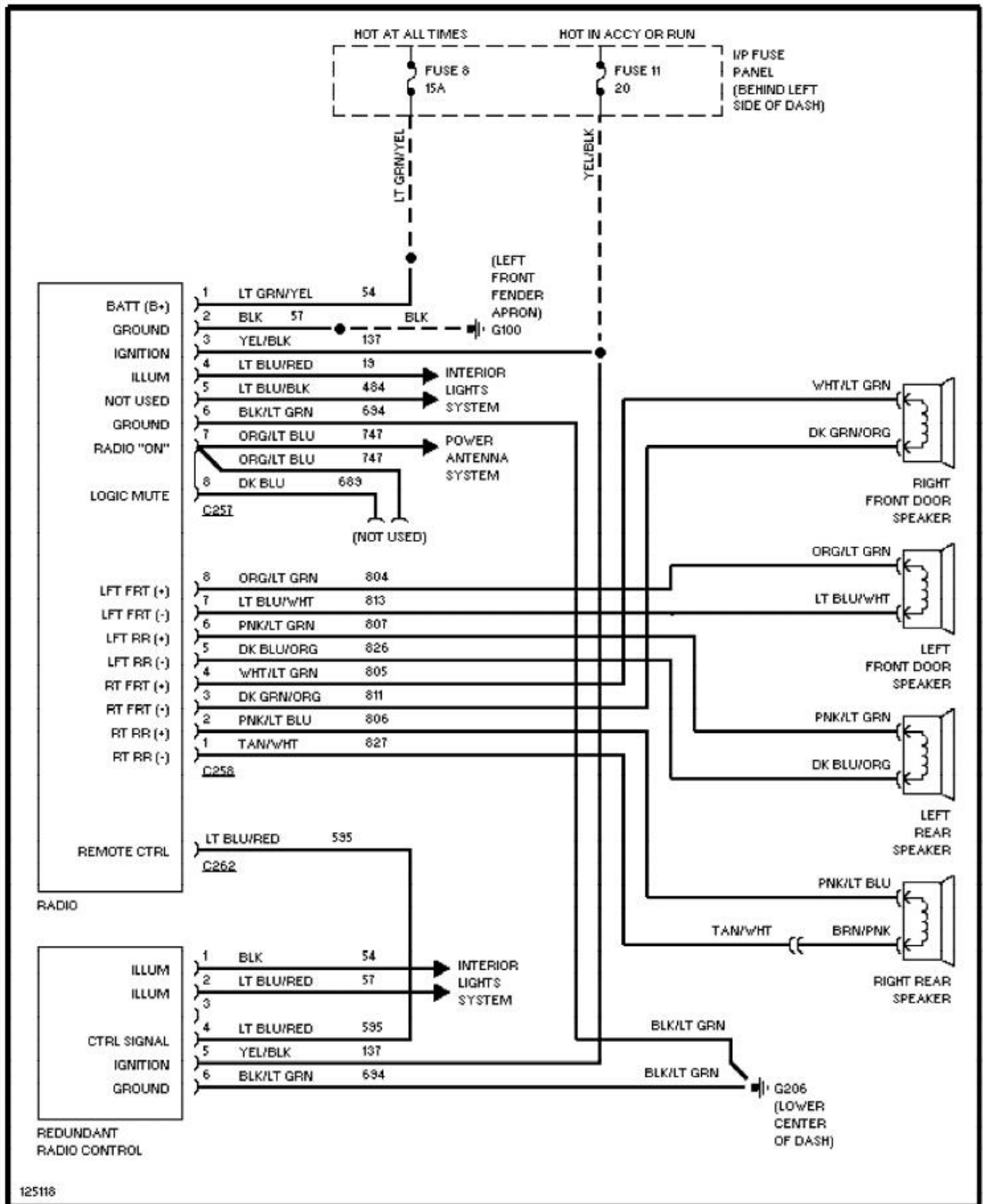
Fig. 86: Base Radio 1994 Ford Taurus LX
