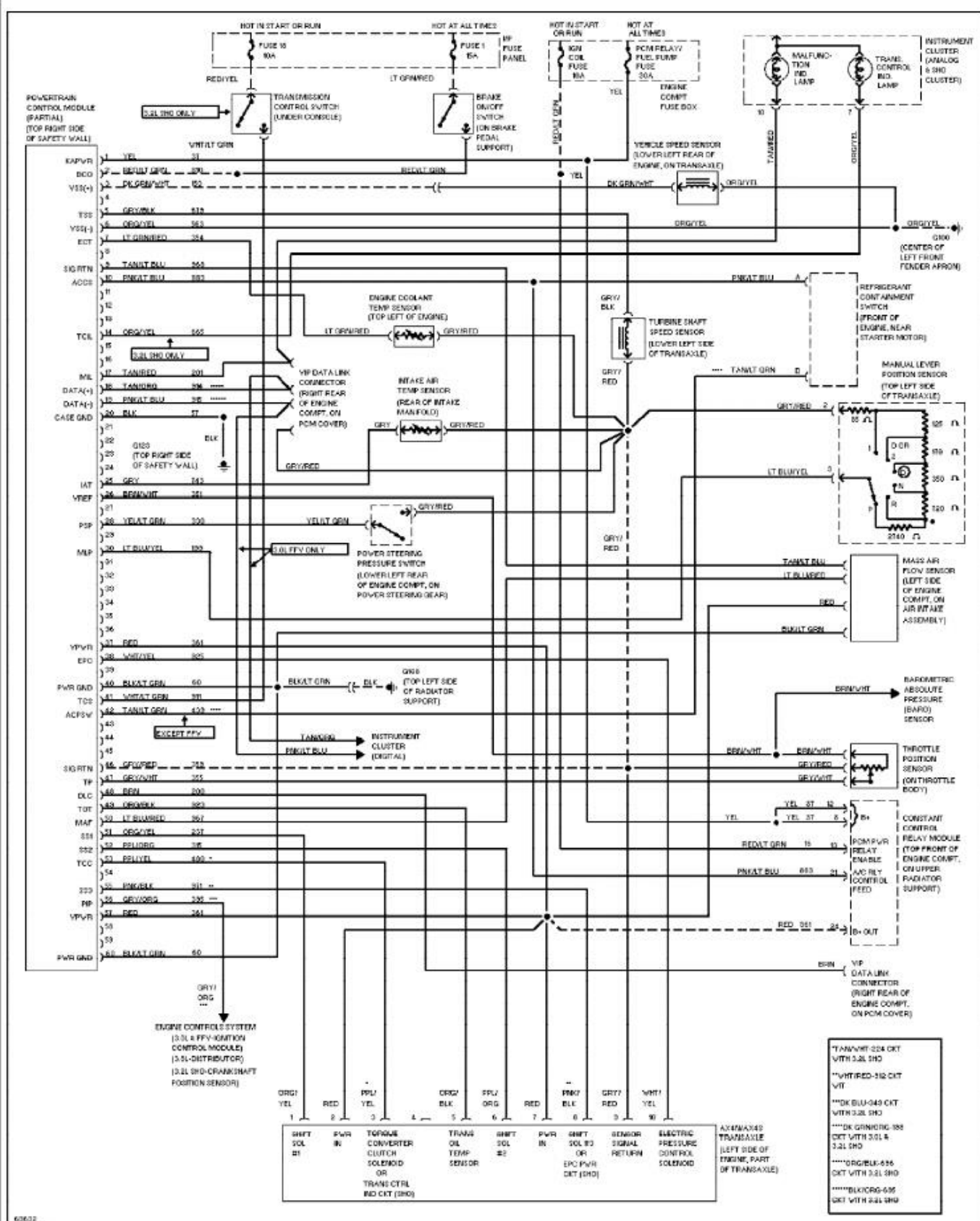
Fig. 100: Transmission Circuit 1994 Ford Taurus LX
