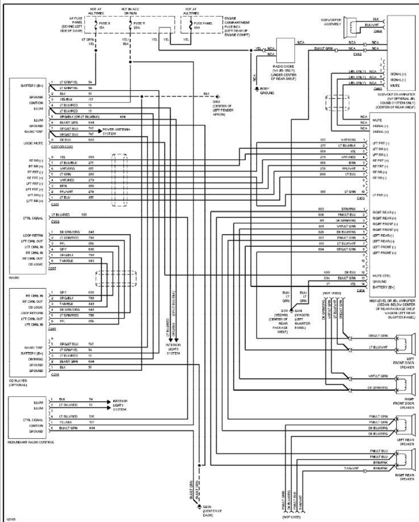
Fig. 87: JBL System 1994 Ford Taurus LX
