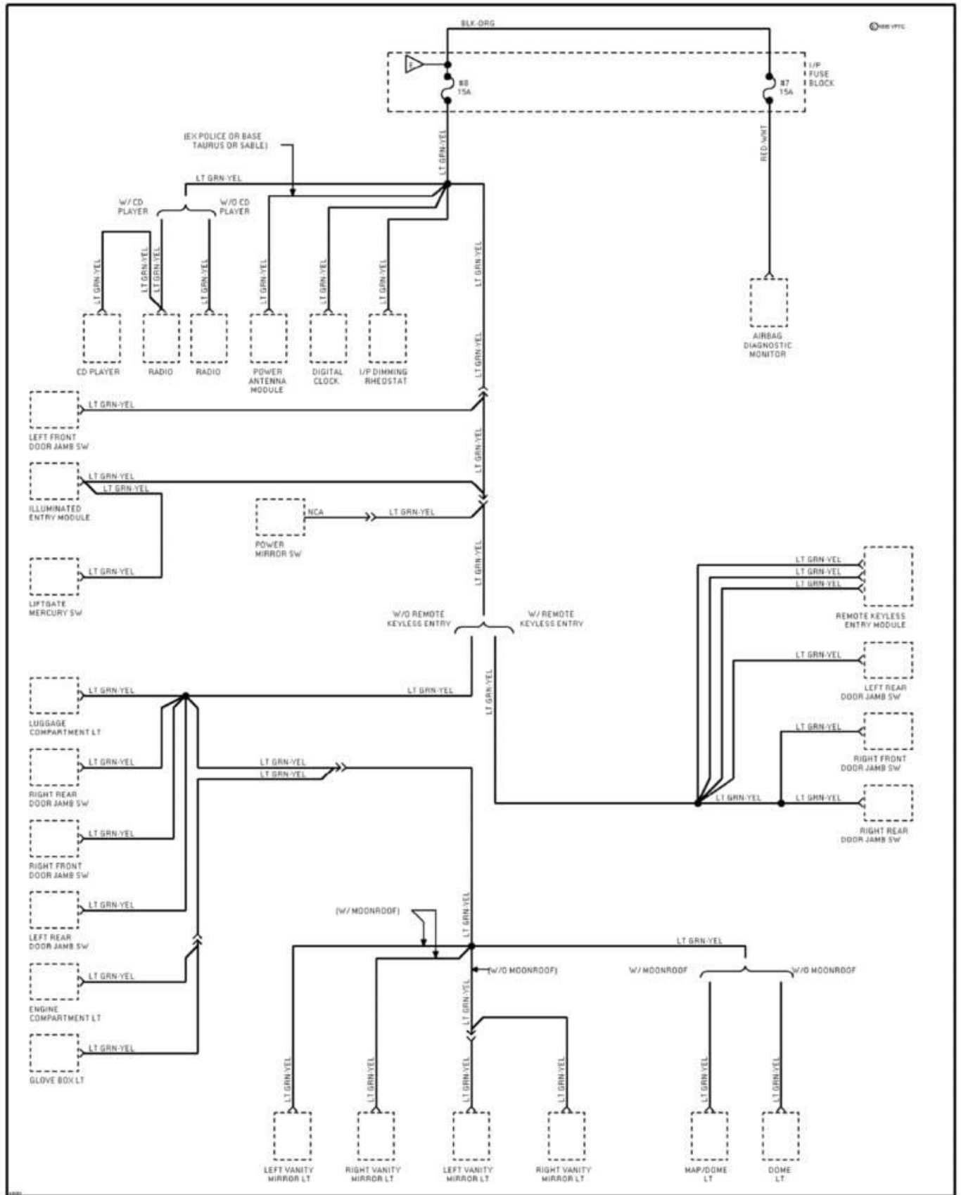
Fig. 85: Power Distribution Circuit (3 of 6) 1995 Ford Taurus LX
