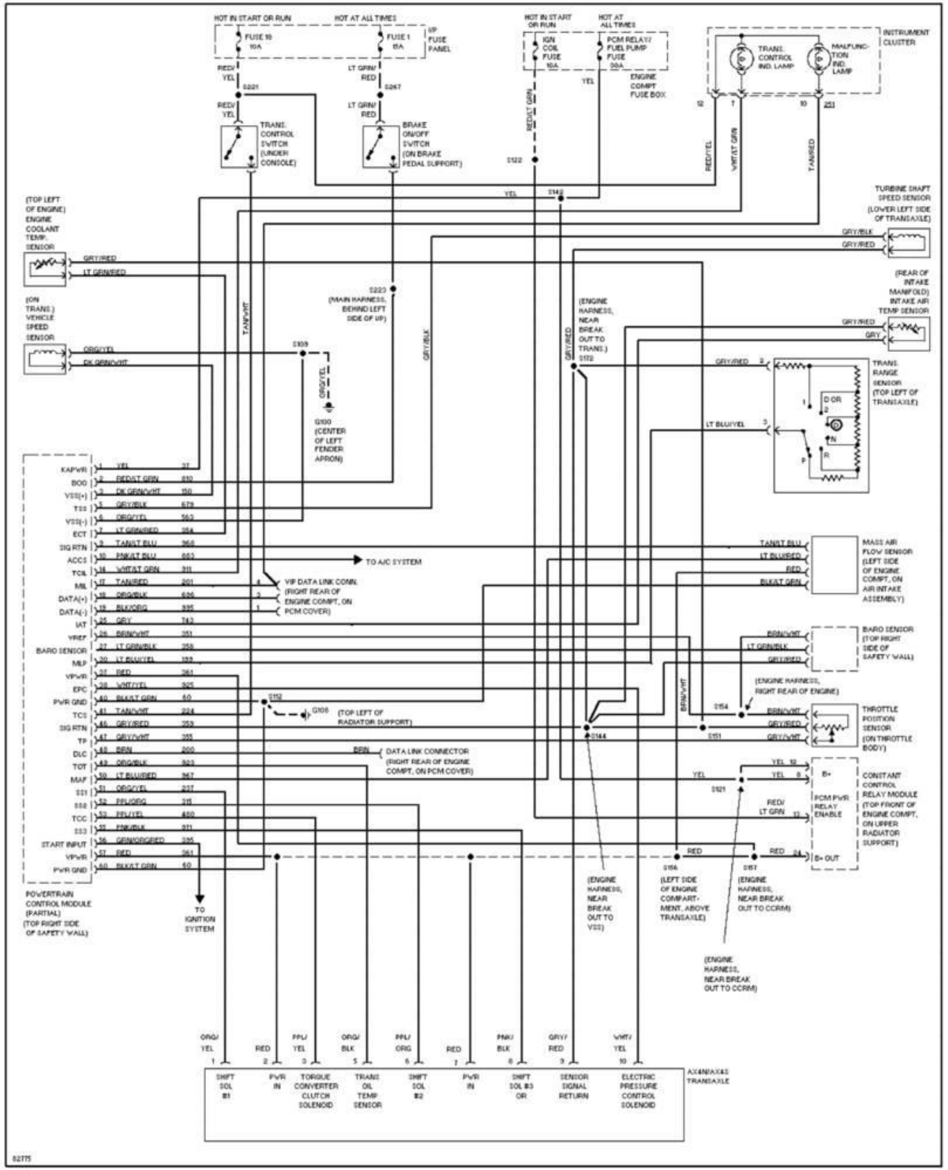
Fig. 113: 3.2L SHO, Transmission Circuit 1995 Ford Taurus LX
