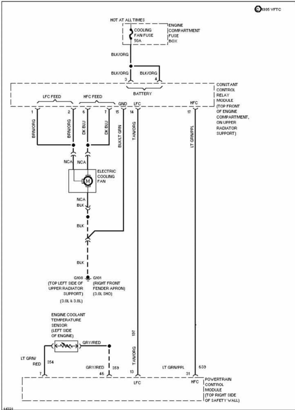
Fig. 25: 3.8L, Cooling Fan Circuit 1995 Ford Taurus LX
