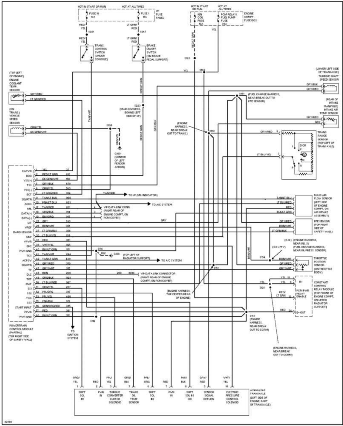
Fig. 112: 3.0L, Transmission Circuit 1995 Ford Taurus LX
