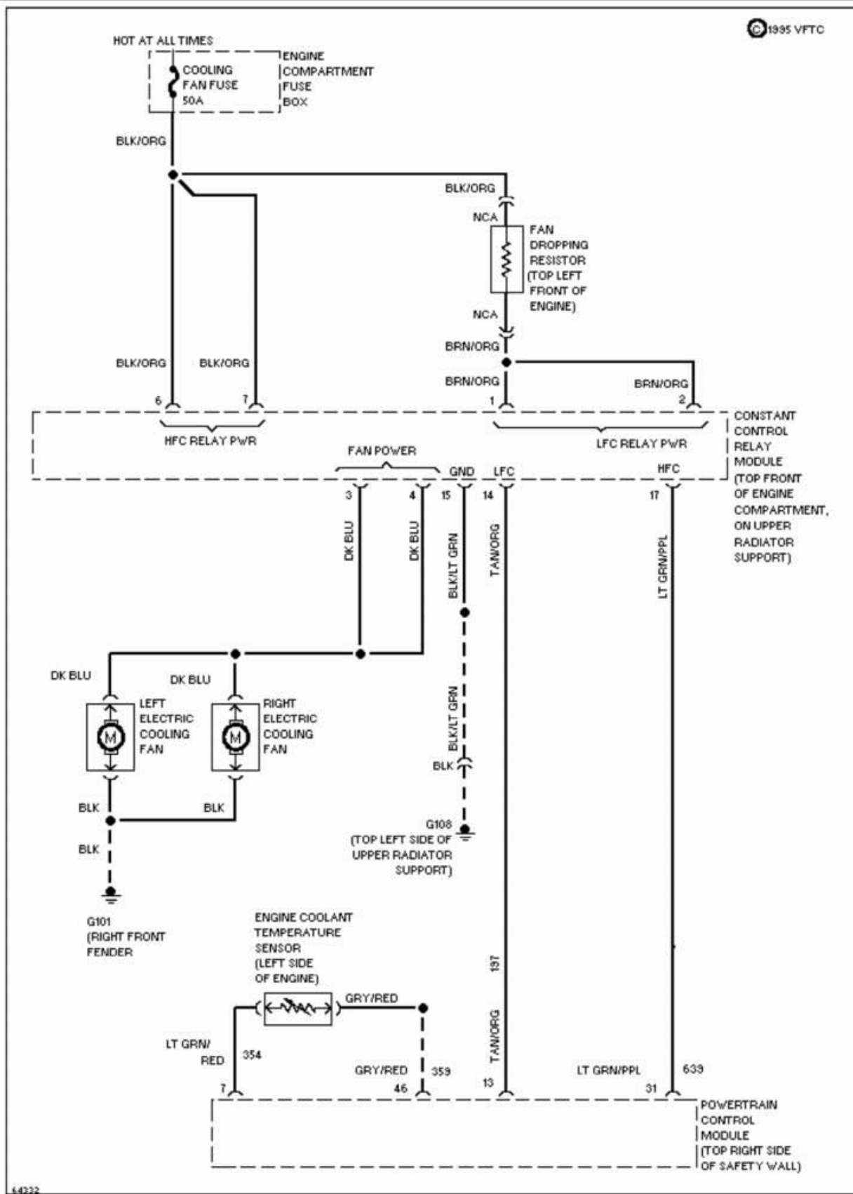
Fig. 24: 3.2L SHO, Cooling Fan Circuit 1995 Ford Taurus LX
