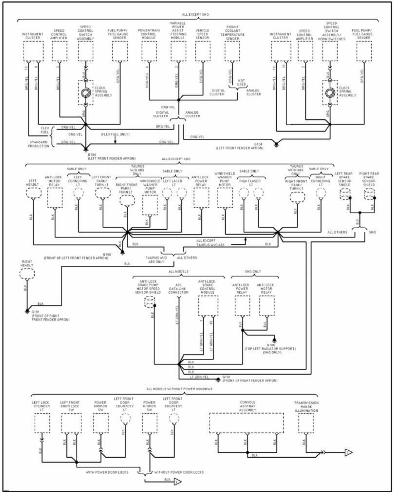
Fig. 47: Ground Distribution Circuit (2 of 5) 1995 Ford Taurus LX
