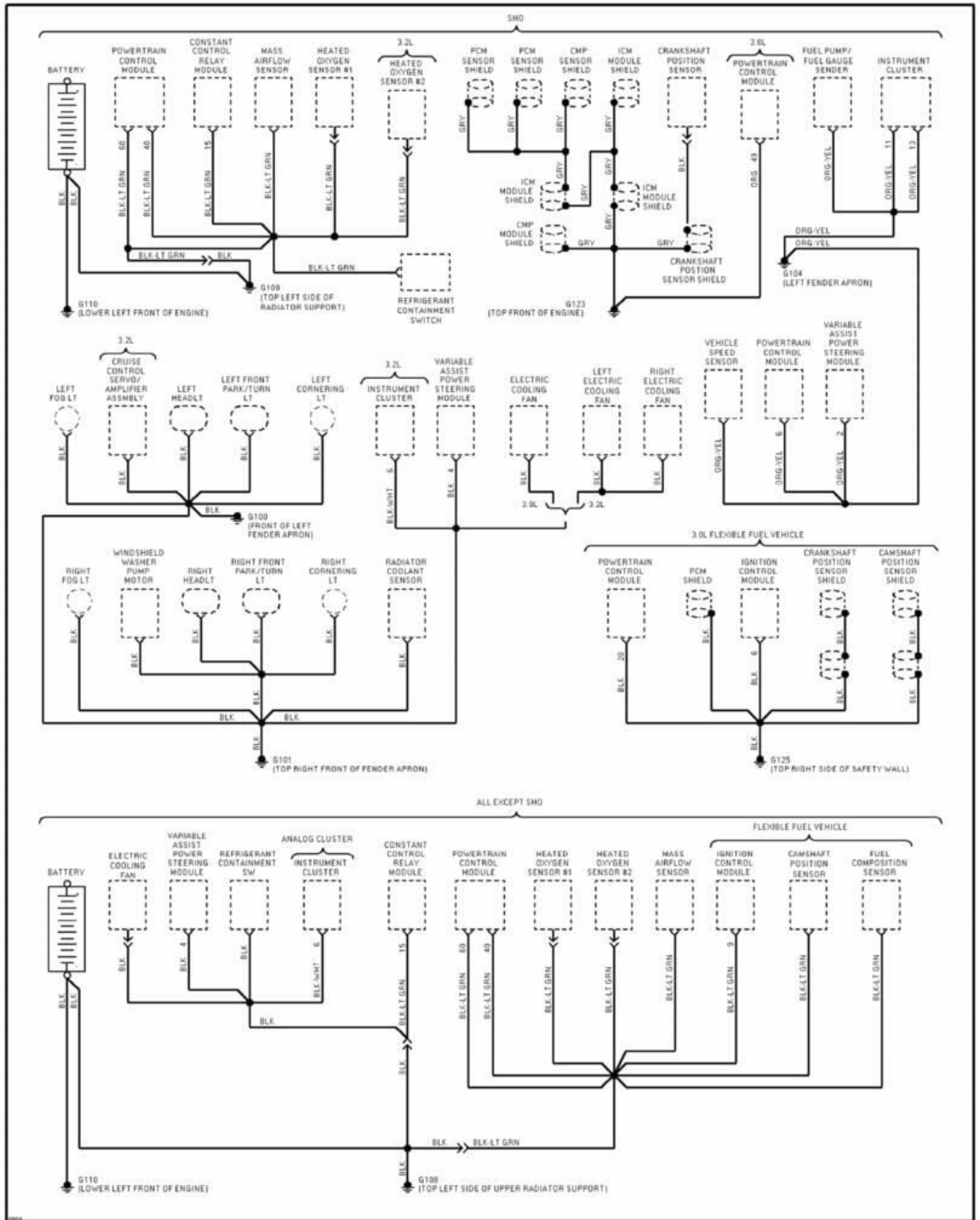
Fig. 46: Ground Distribution Circuit (1 of 5) 1995 Ford Taurus LX
