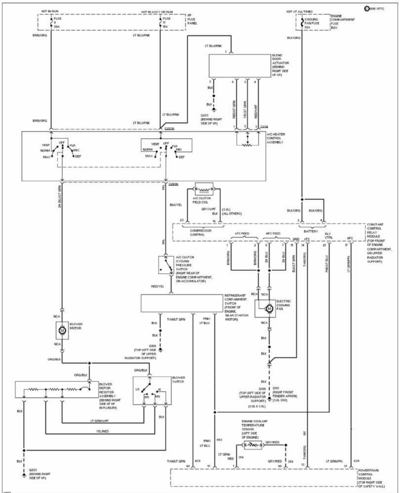
Fig. 10: 3.8L, A/C Circuit, Manual A/C 1995 Ford Taurus LX
