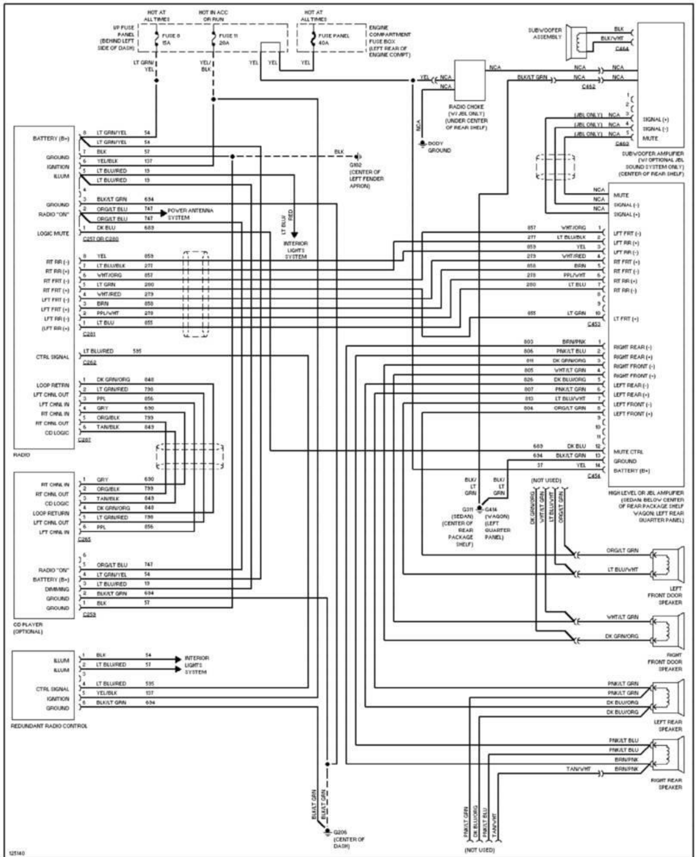
Fig. 98: JBL System 1995 Ford Taurus LX
