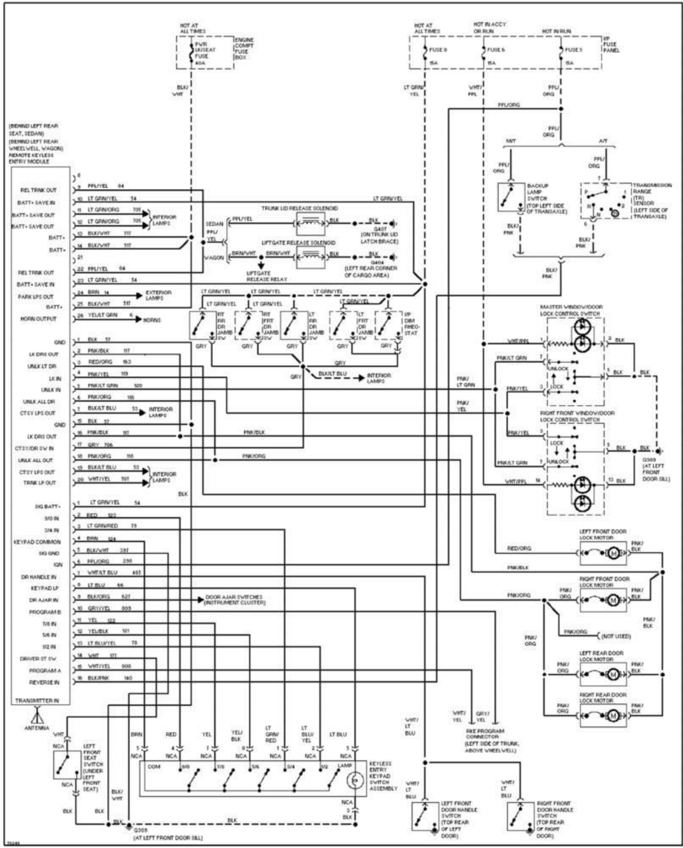
Fig. 91: Keyless Entry Circuit 1995 Ford Taurus LX
