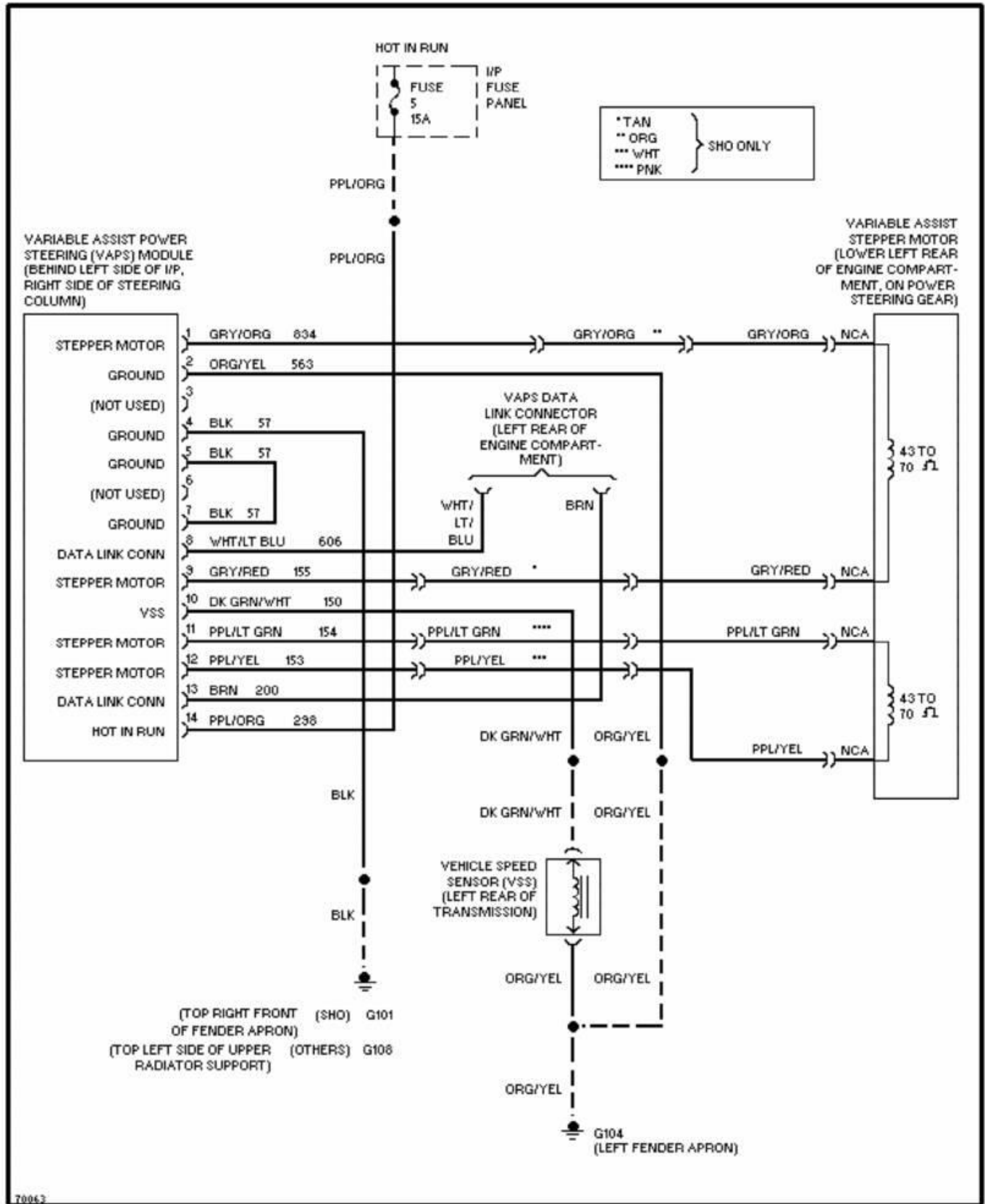
Fig. 32: Electronic Power Steering Circuit 1995 Ford Taurus LX
