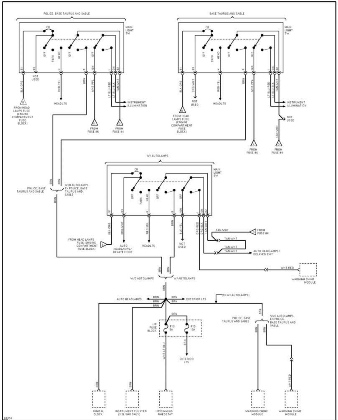
Fig. 88: Power Distribution Circuit (6 of 6) 1995 Ford Taurus LX
