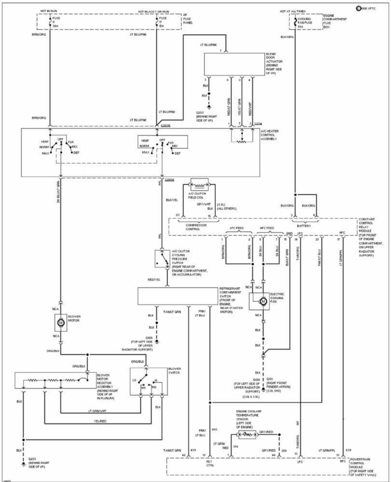
Fig. 4: 3.0L SHO, A/C Circuit, Manual A/C 1995 Ford Taurus LX
