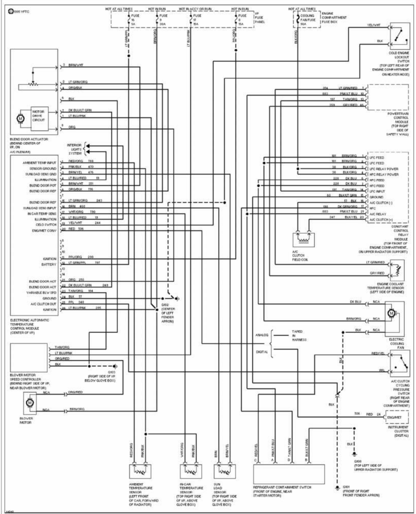
Fig. 3: 3.0L SHO, A/C Circuit, Auto A/C 1995 Ford Taurus LX
