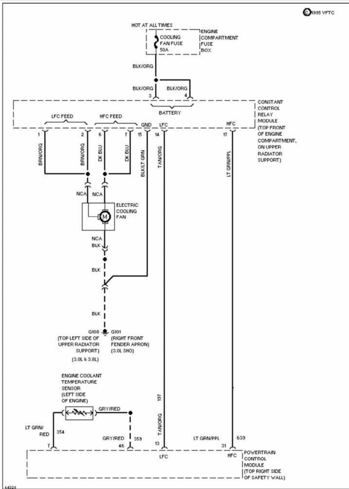
Fig. 21: 3.0L Flex Fuel, Cooling Fan Circuit 1995 Ford Taurus LX
