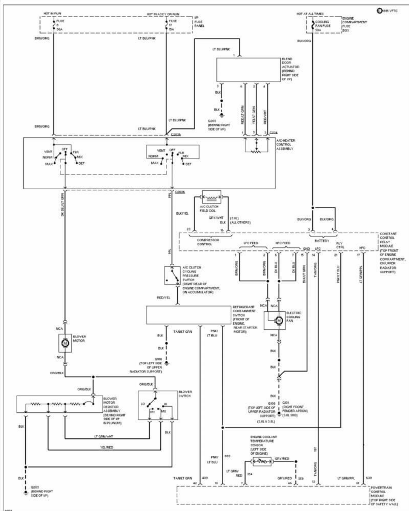
Fig. 2: 3.0L Flex Fuel, A/C Circuit, Manual A/C 1995 Ford Taurus LX
