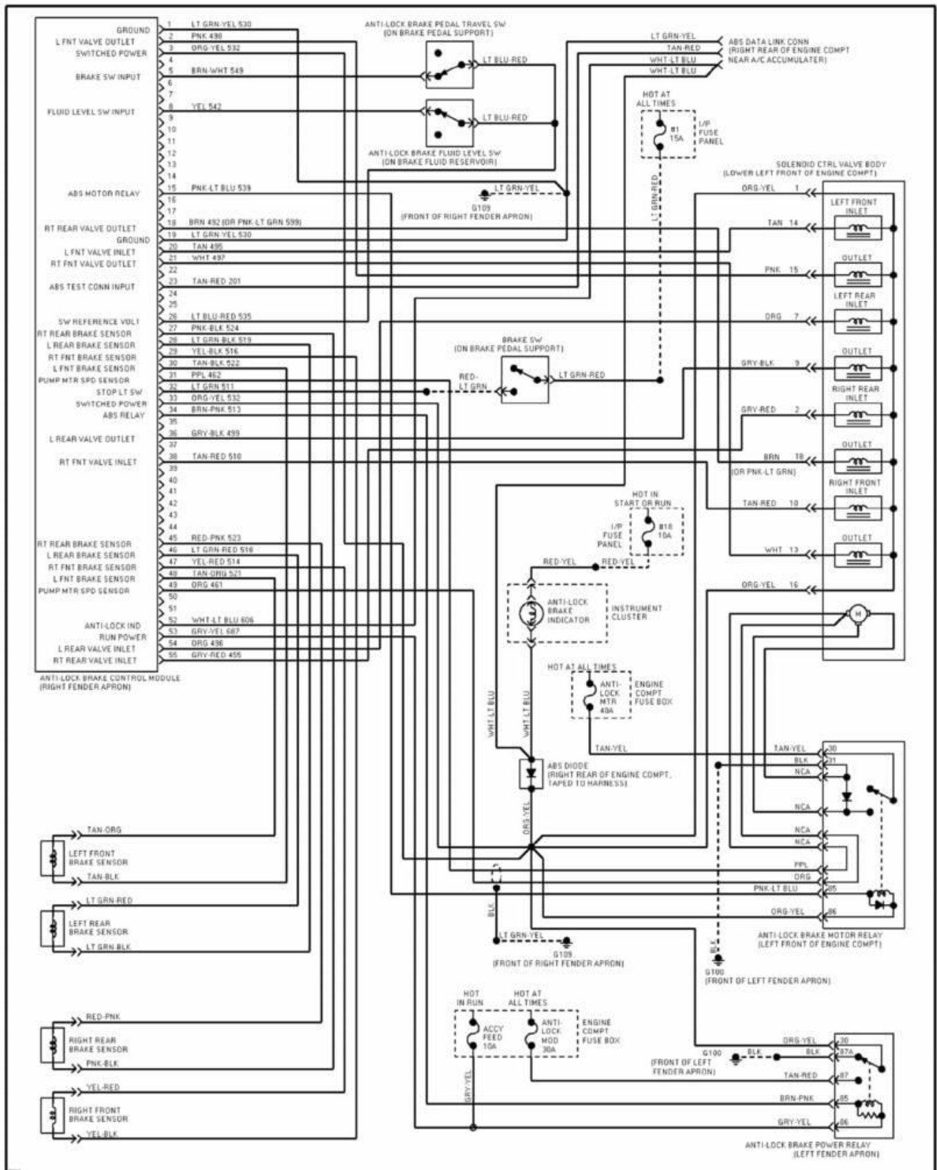
Fig. 15: 3.8L, Anti-lock Brake Circuits 1995 Ford Taurus LX
