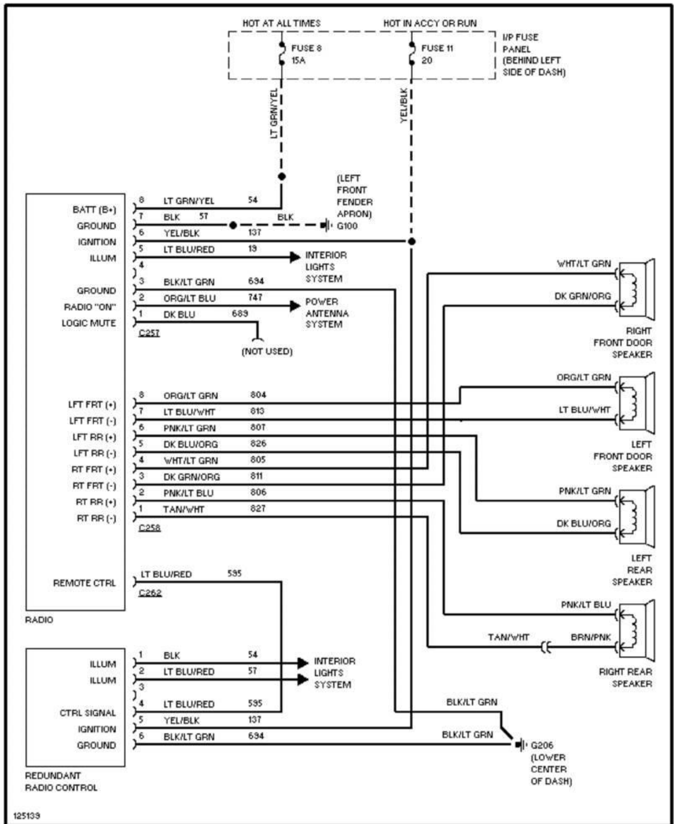
Fig. 97: Base Radio 1995 Ford Taurus LX
