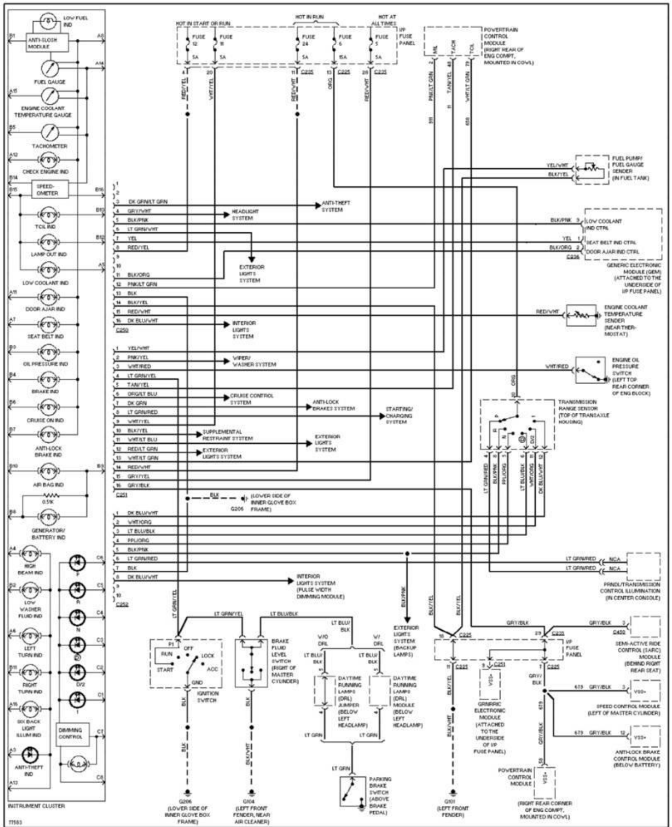
Fig. 47: 3.0L, Instrument Cluster Circuit 1996 Ford Taurus LX
