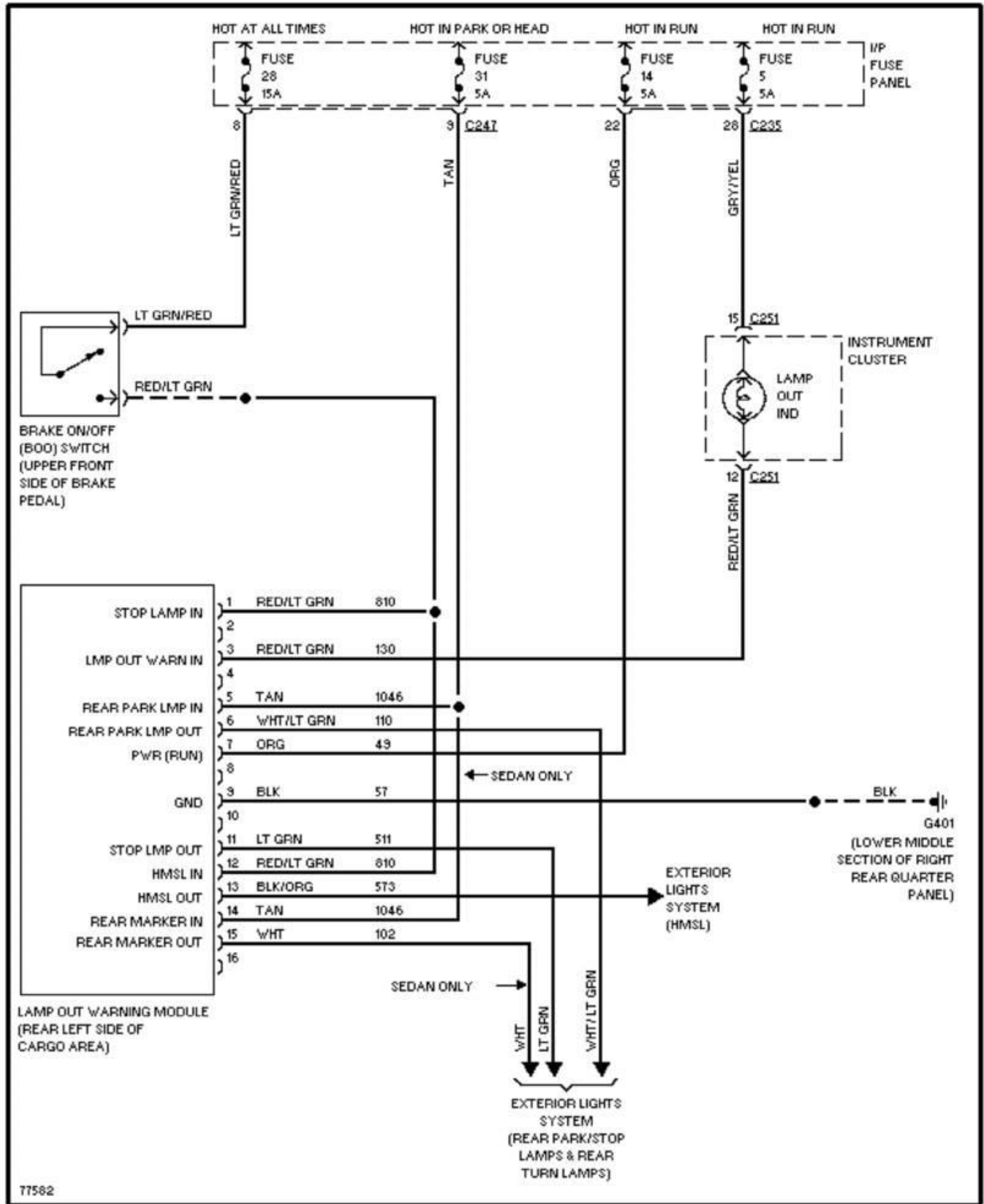
Fig. 48: Lamp Monitor Circuit 1996 Ford Taurus LX
