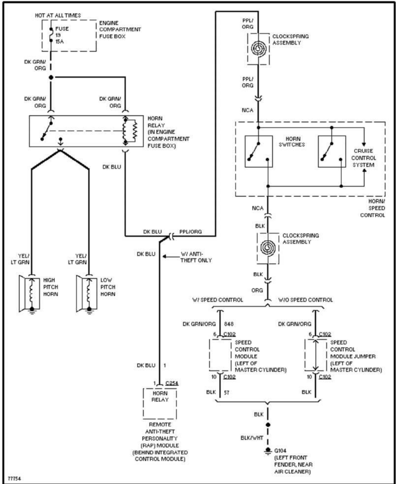
Fig. 45: Horn Circuit 1996 Ford Taurus LX
