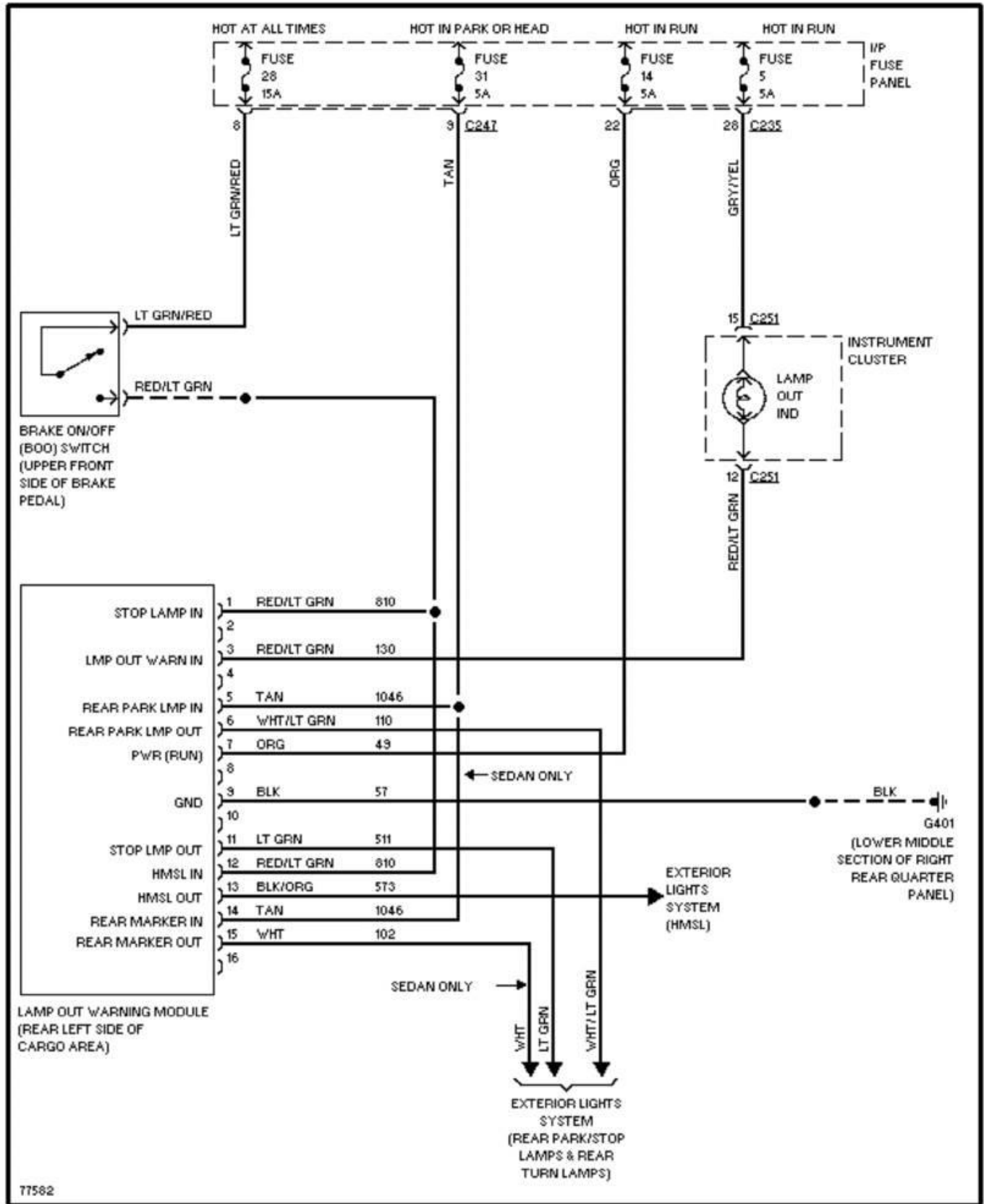
Fig. 50: Lamp Monitor Circuit 1996 Ford Taurus LX
