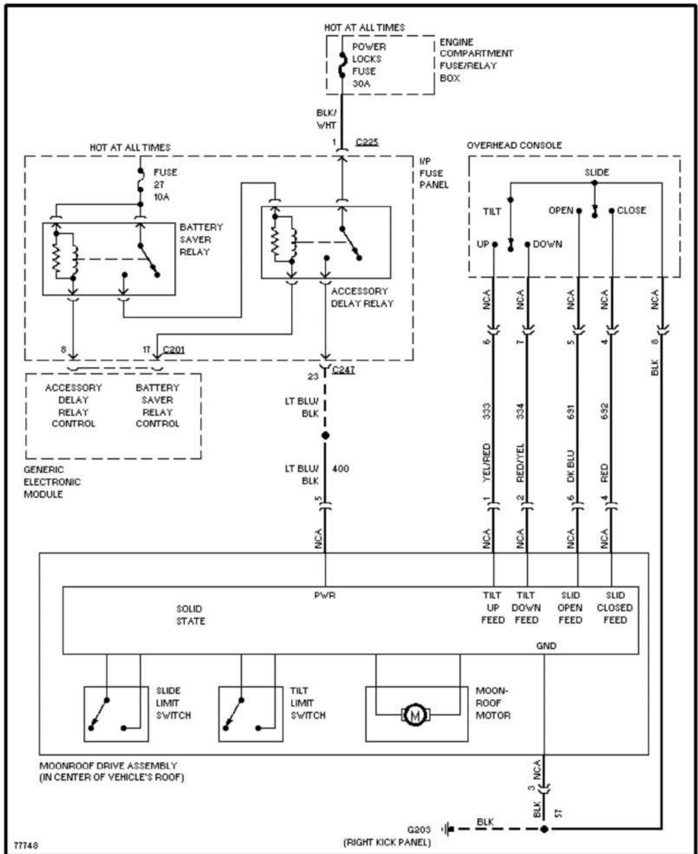
Fig. 60: Power Top/Sunroof Circuits 1996 Ford Taurus LX
