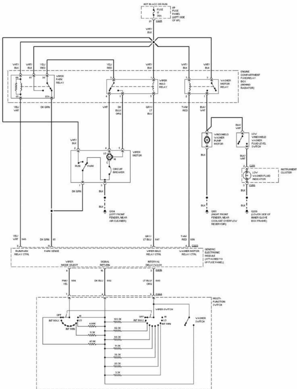
Fig. 78: Front Wiper/Washer Circuit 1996 Ford Taurus LX
