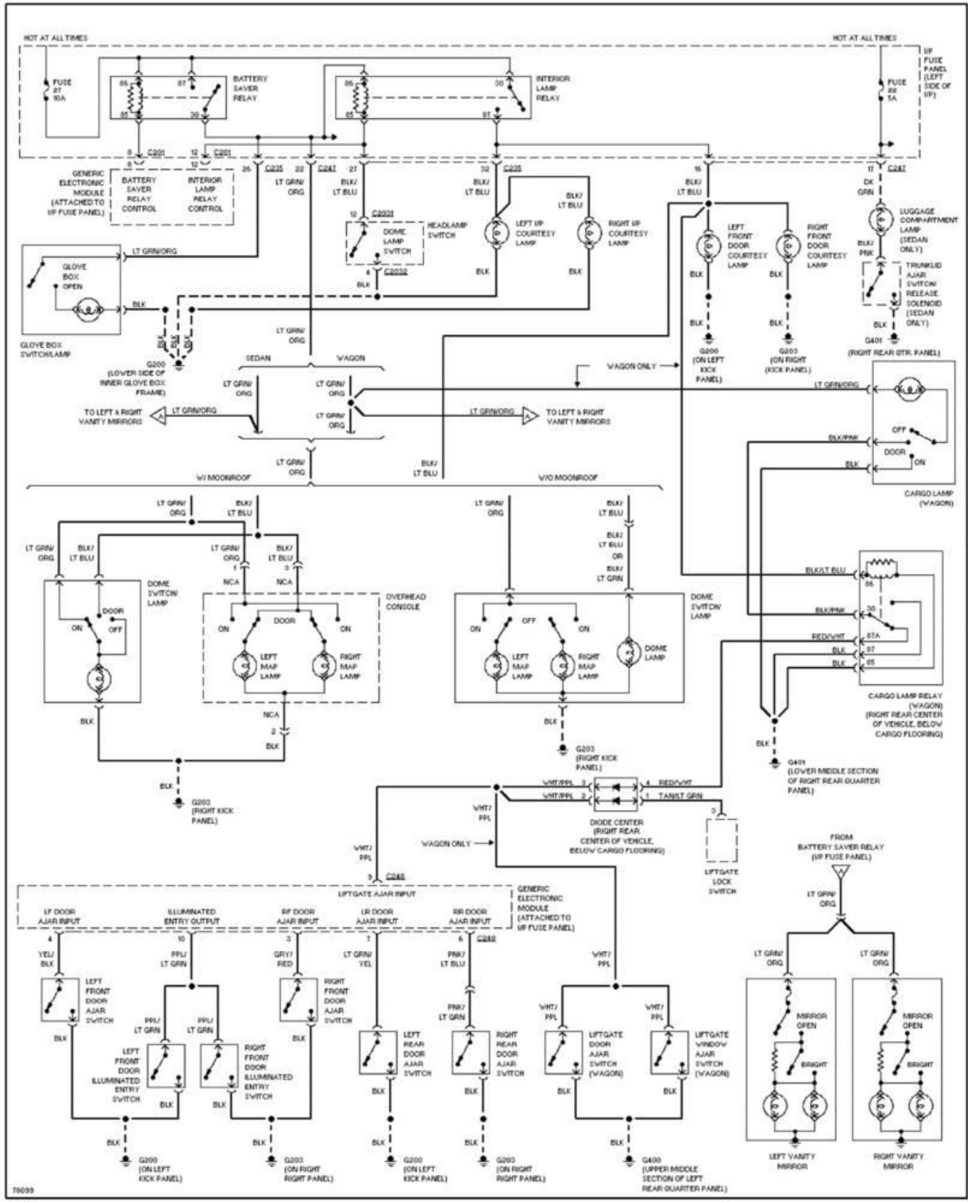
Fig. 51: Courtesy Lamps Circuit 1996 Ford Taurus LX
