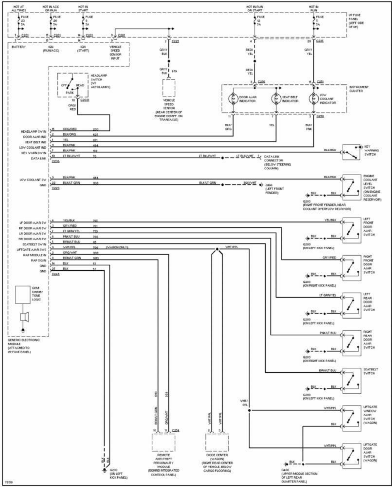
Fig. 77: Warning System Circuits 1996 Ford Taurus LX
