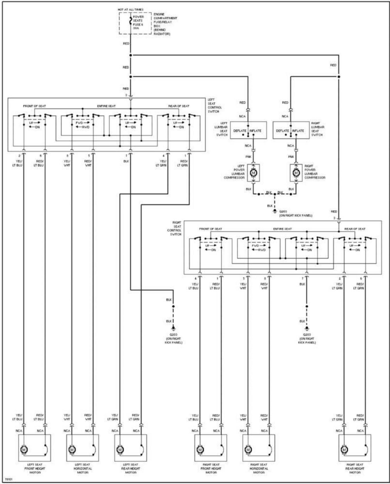
Fig. 59: Power & Lumbar Seat Circuit 1996 Ford Taurus LX
