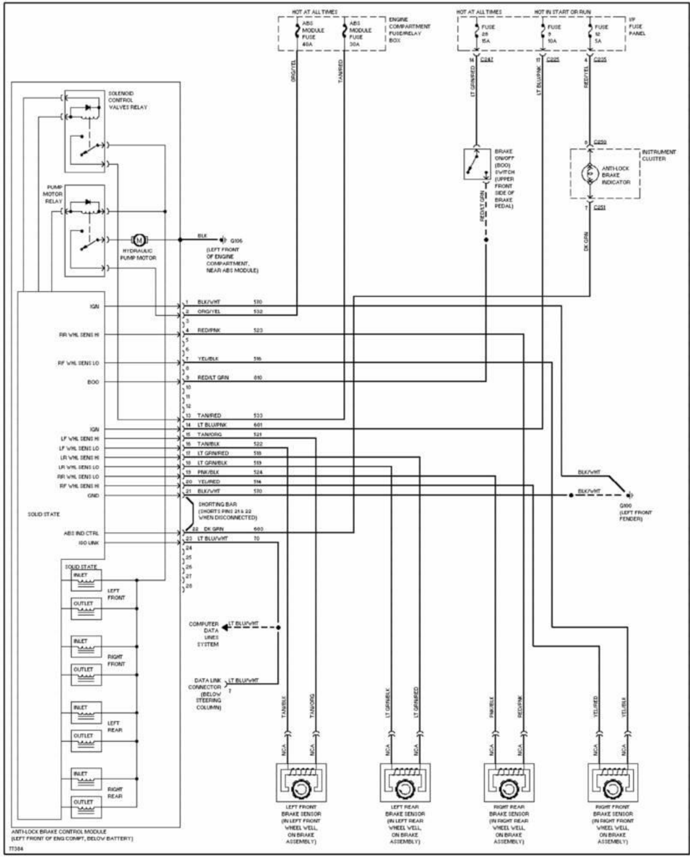
Fig. 3: Anti-lock Brake Circuits 1996 Ford Taurus LX
