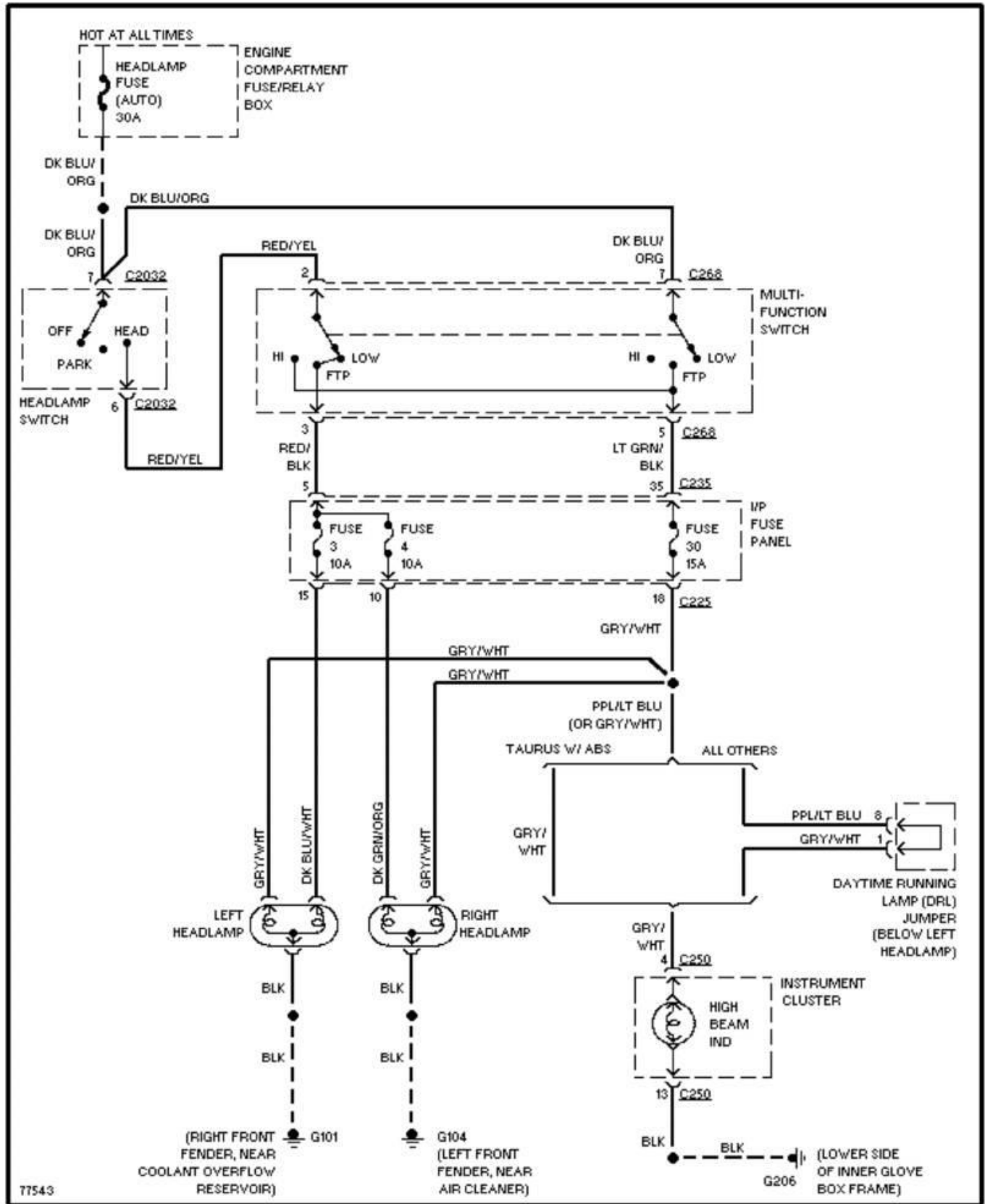
Fig. 44: Headlamps Circuit, W/O DRL 1996 Ford Taurus LX
