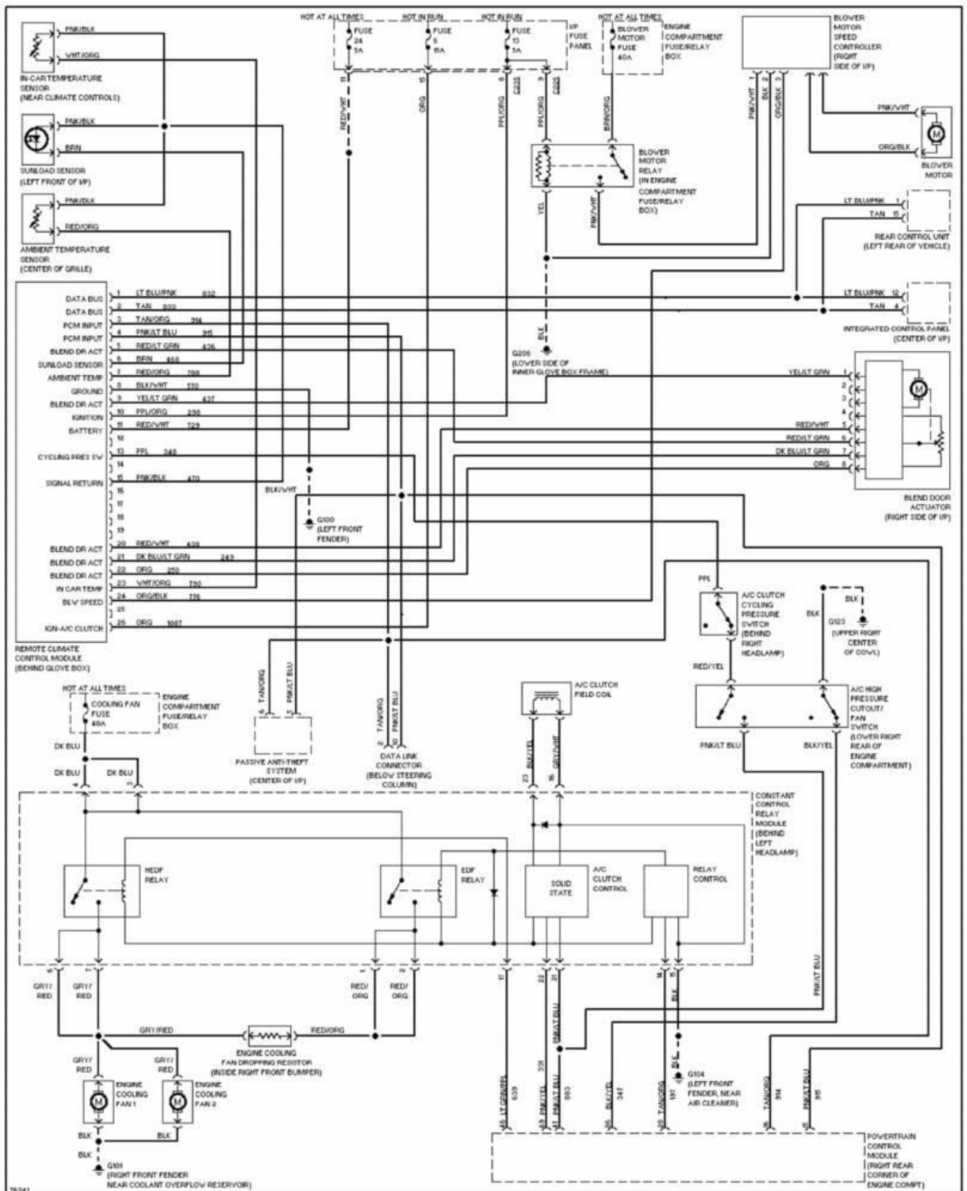
Fig. 1: A/C Circuit, Auto A/C 1996 Ford Taurus LX
