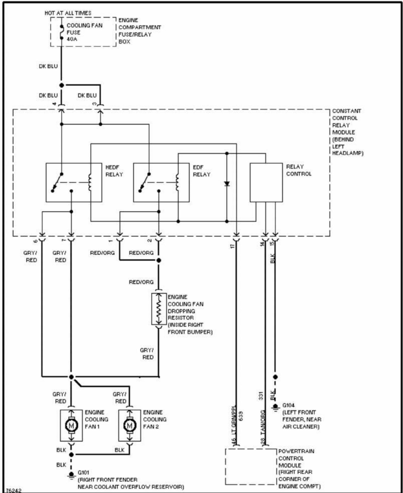
Fig. 7: Cooling Fan Circuit 1996 Ford Taurus LX
