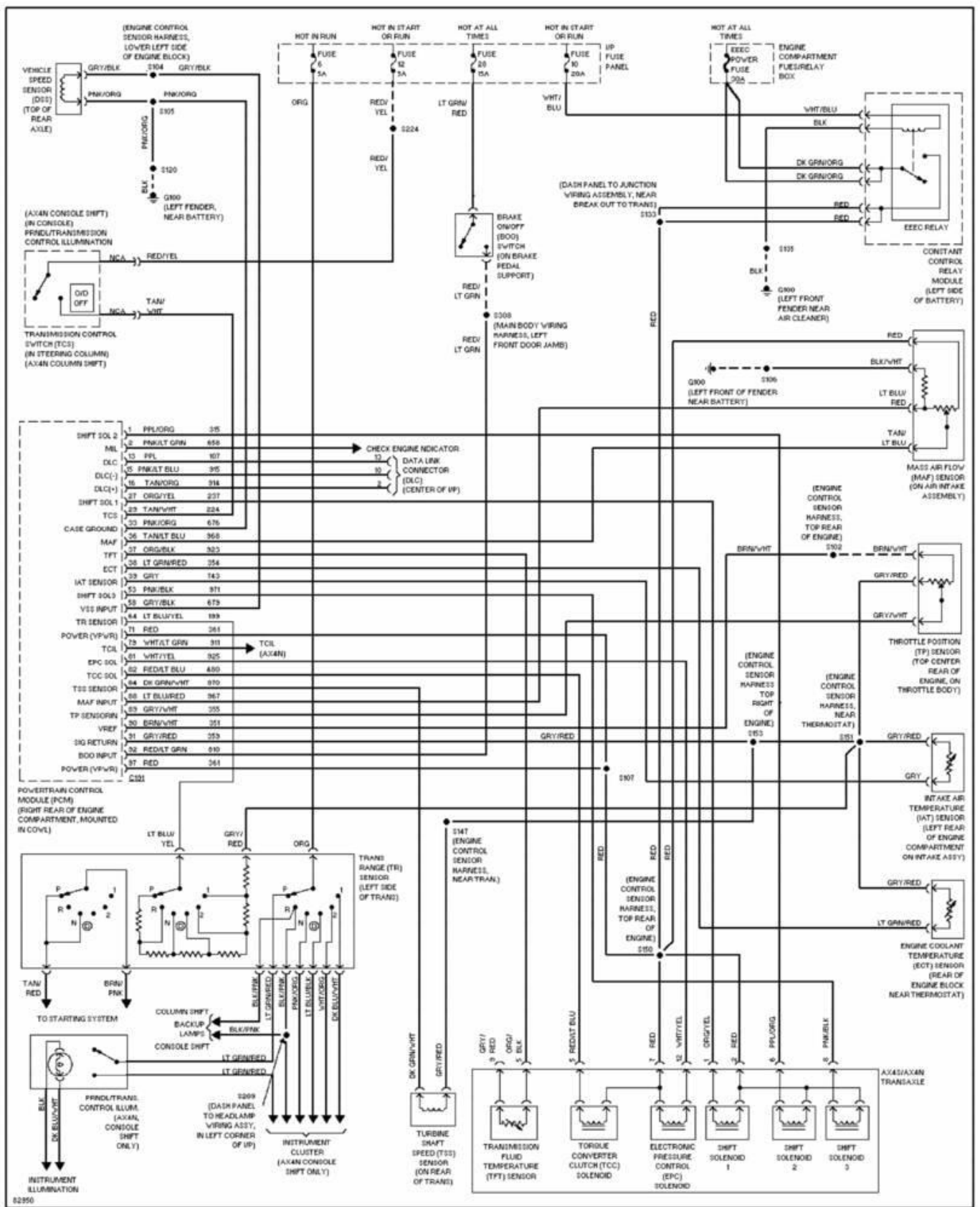
Fig. 75: 3.4L SHO, Transmission Circuit 1996 Ford Taurus LX
