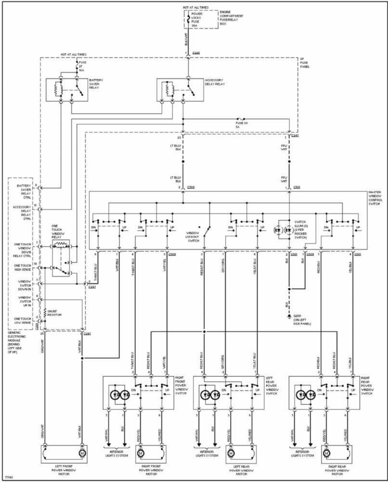
Fig. 61: Power Window Circuit 1996 Ford Taurus LX
