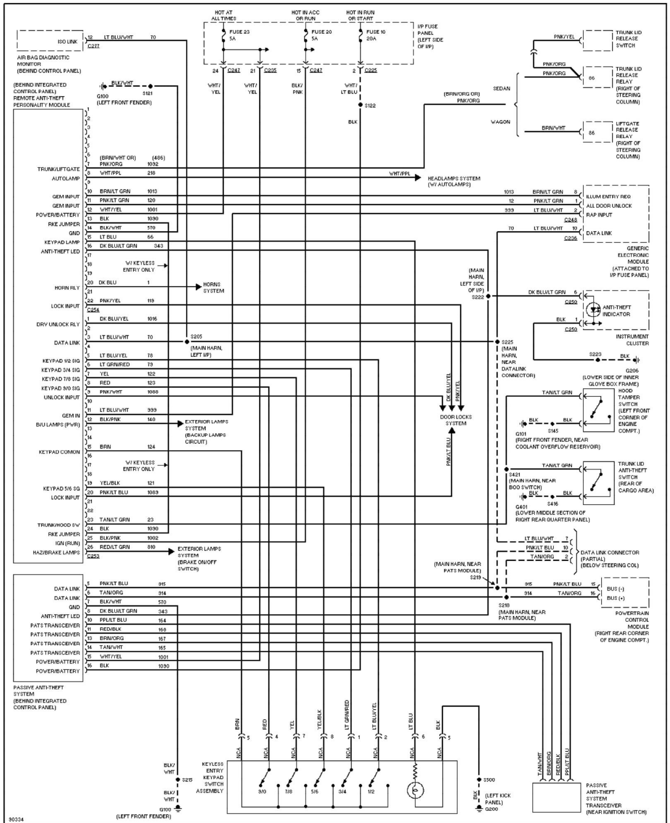
Fig. 4: Anti-theft Circuit 1997 Ford Taurus LX
