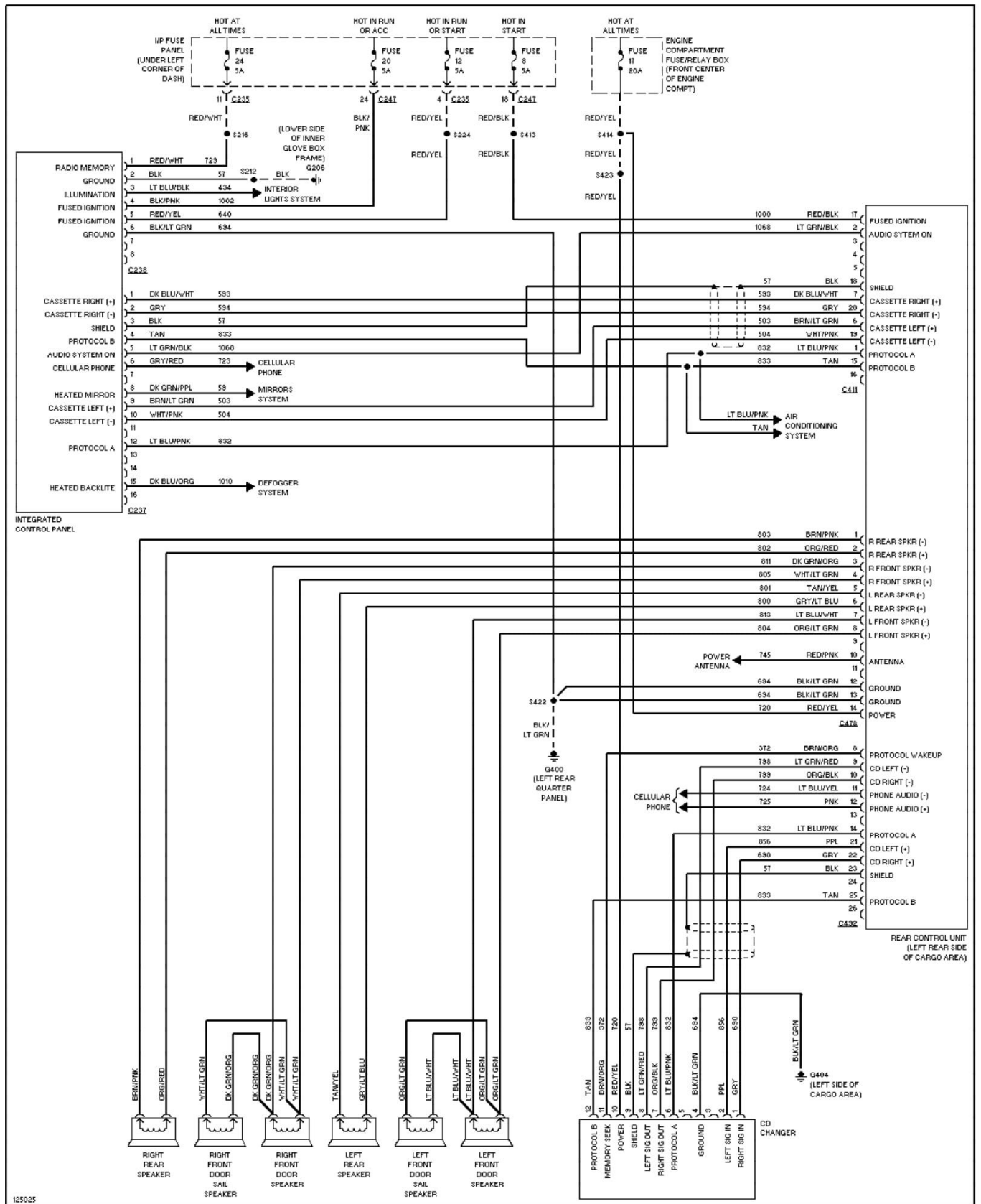
Fig. 59: Radio Circuits, W/ Cassette Deck 1997 Ford Taurus LX
