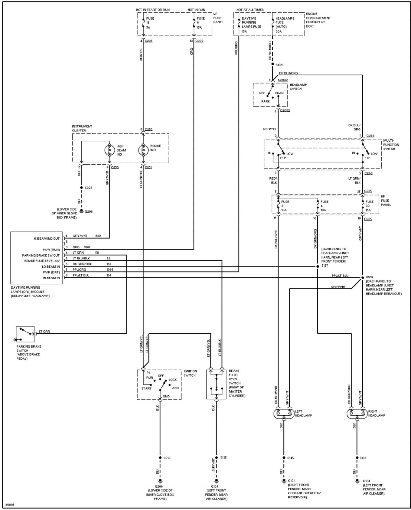
Fig. 40: Headlamps Circuit, W/ DRL 1997 Ford Taurus LX
