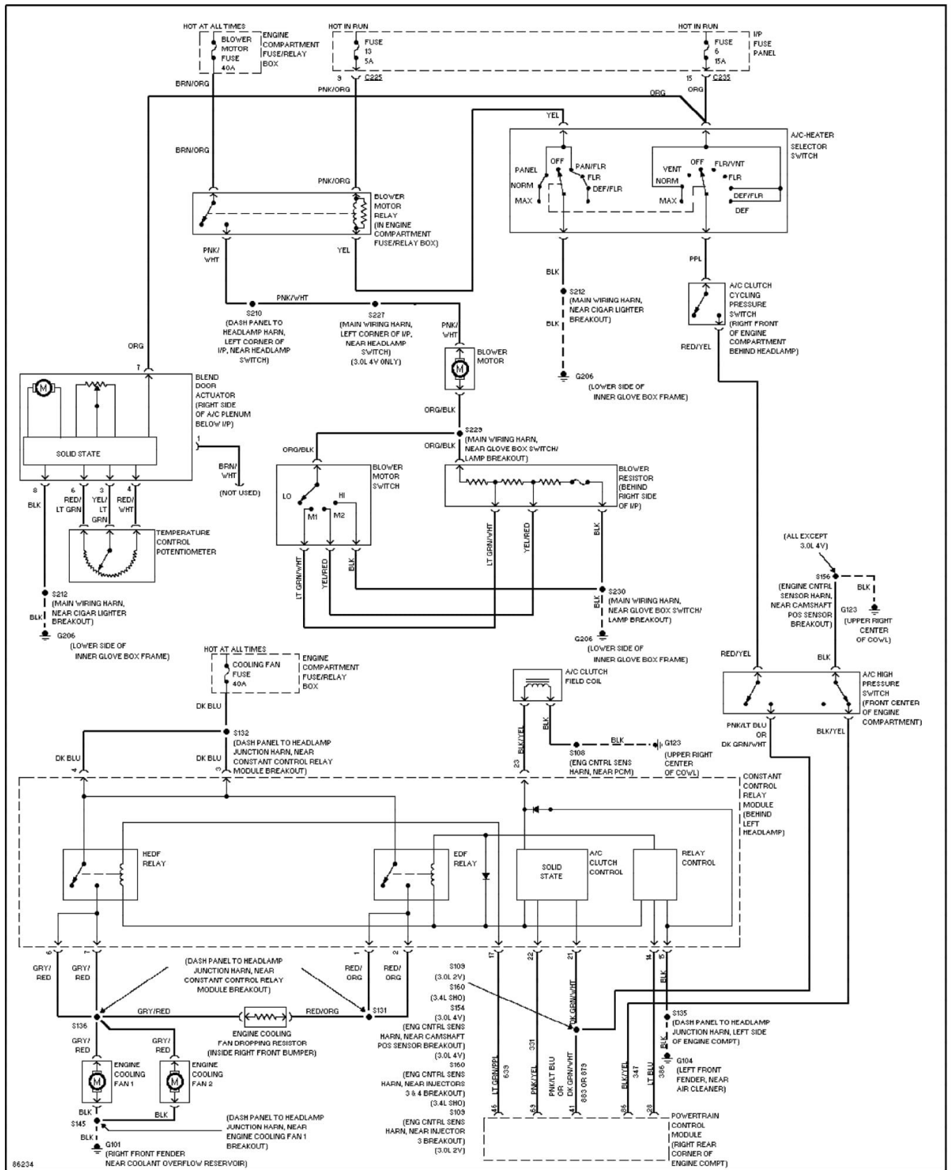
Fig. 2: A/C Circuit, Manual A/C 1997 Ford Taurus LX
