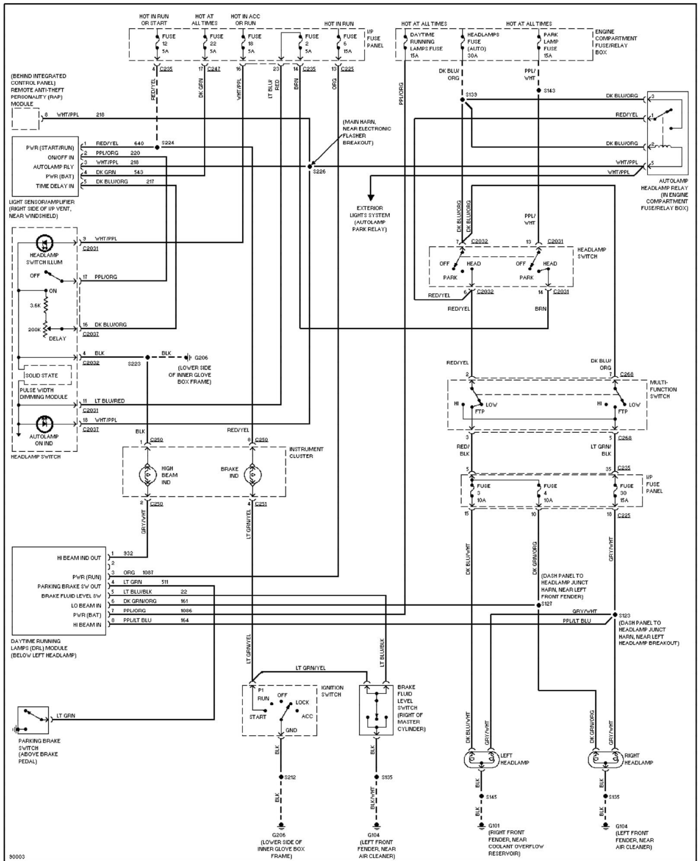
Fig. 38: Autolamps Circuit, W/ DRL 1997 Ford Taurus LX
