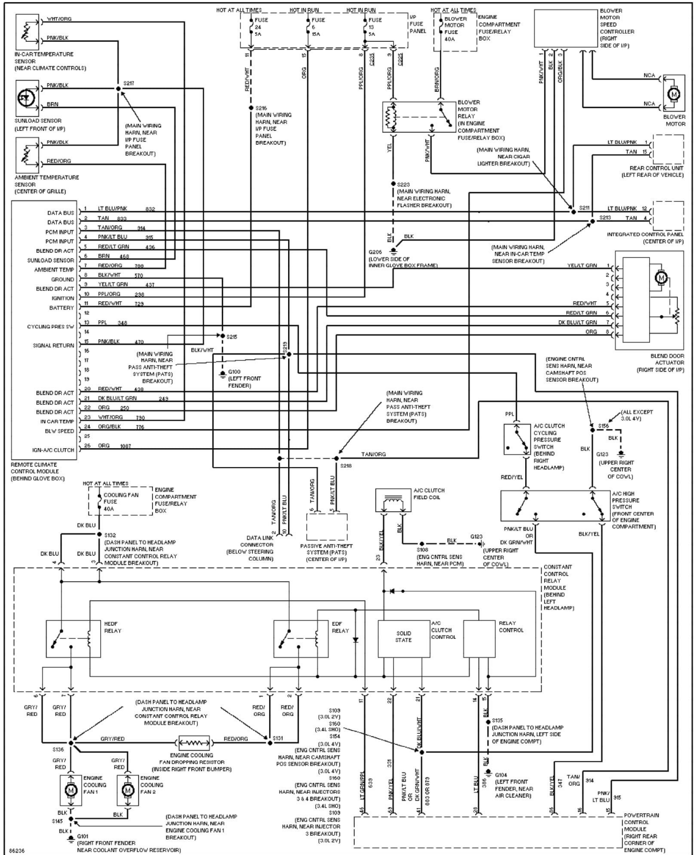
Fig. 1: A/C Circuit, Auto A/C 1997 Ford Taurus LX
