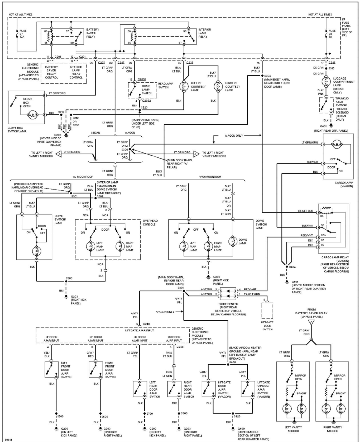
Fig. 48: Courtesy Lamps Circuit 1997 Ford Taurus LX
