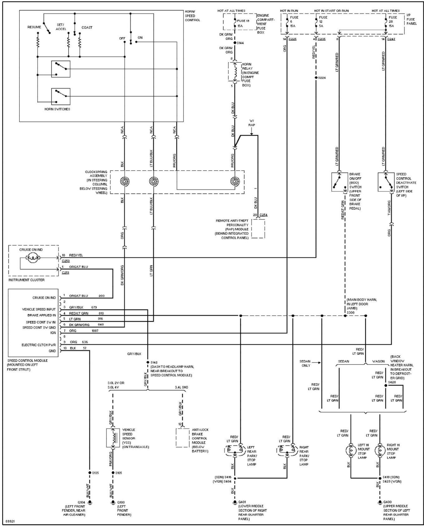
Fig. 8: Cruise Control Circuit 1997 Ford Taurus LX
