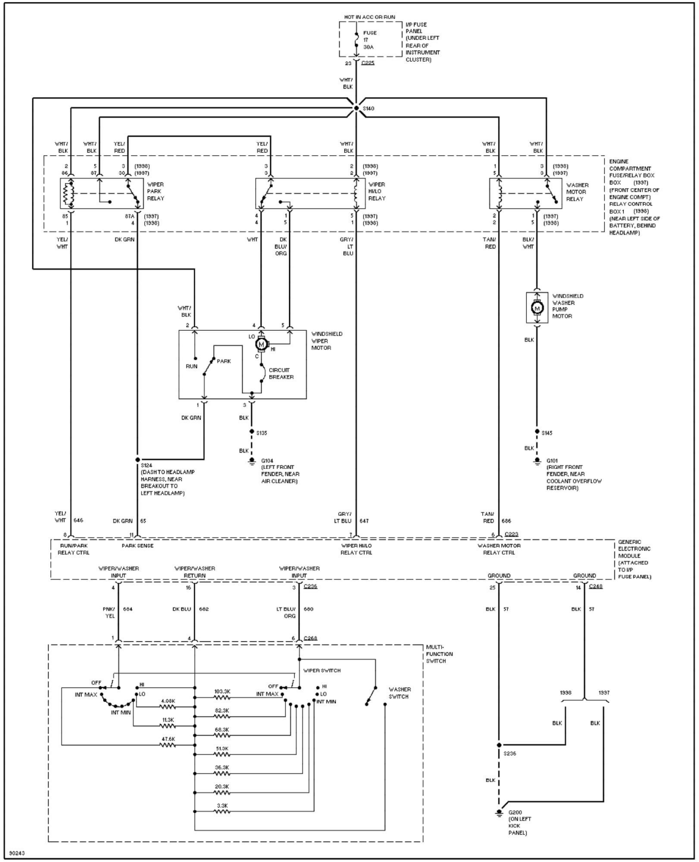
Fig. 75: Front Wiper/Washer Circuit 1997 Ford Taurus LX
