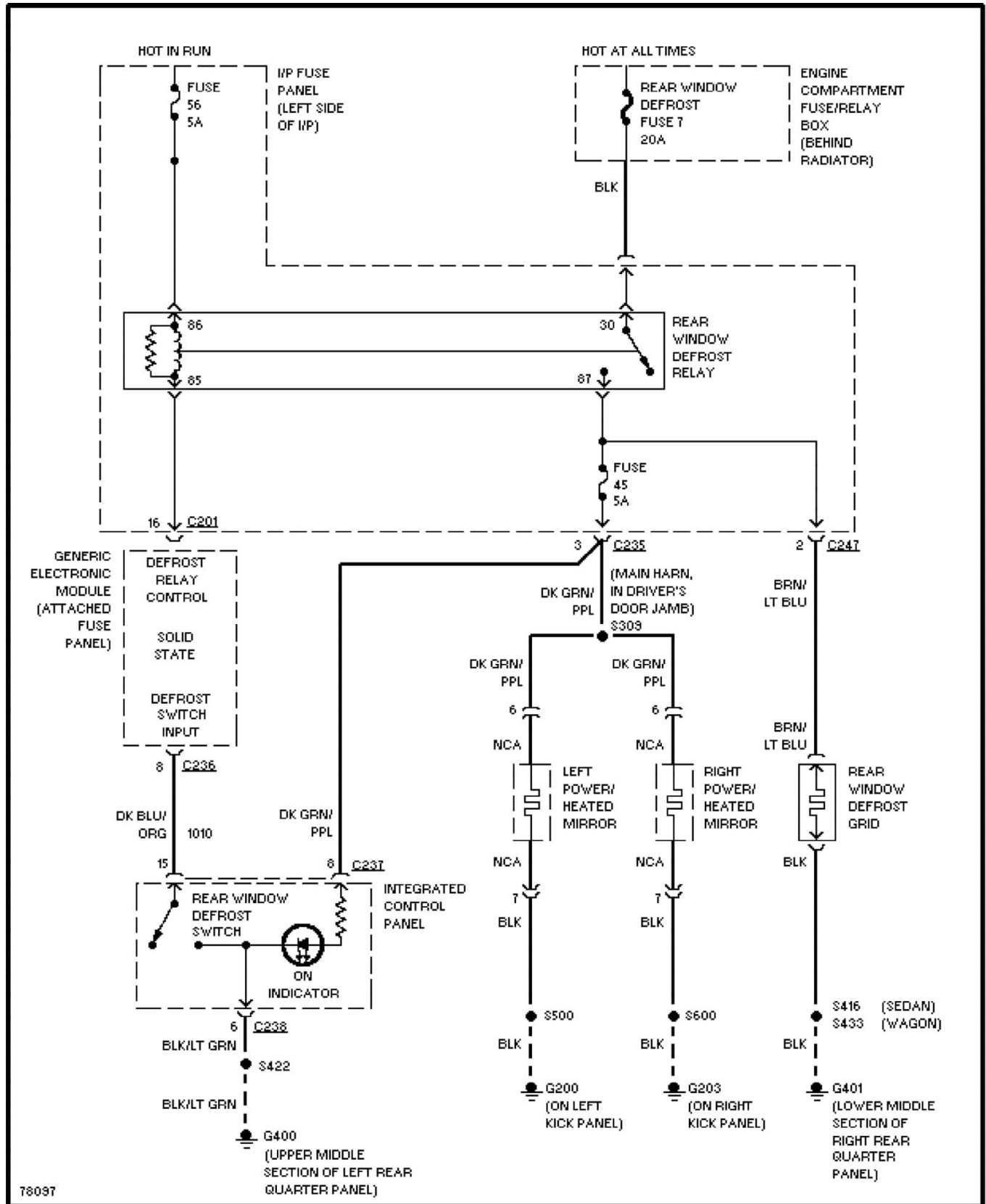
Fig. 9: Defogger Circuit 1997 Ford Taurus LX
