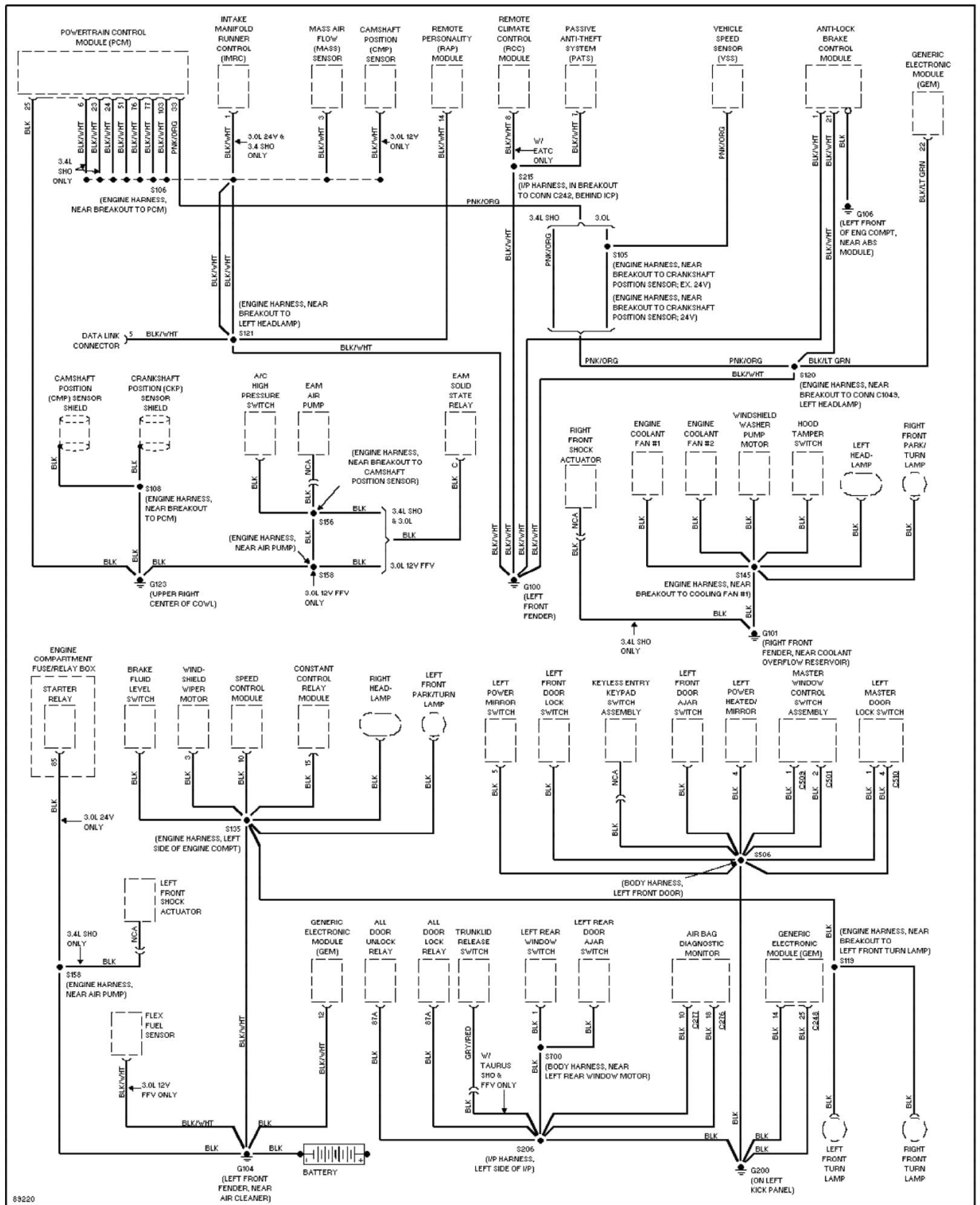
Fig. 35: Ground Distribution Circuit (1 of 3) 1997 Ford Taurus LX
