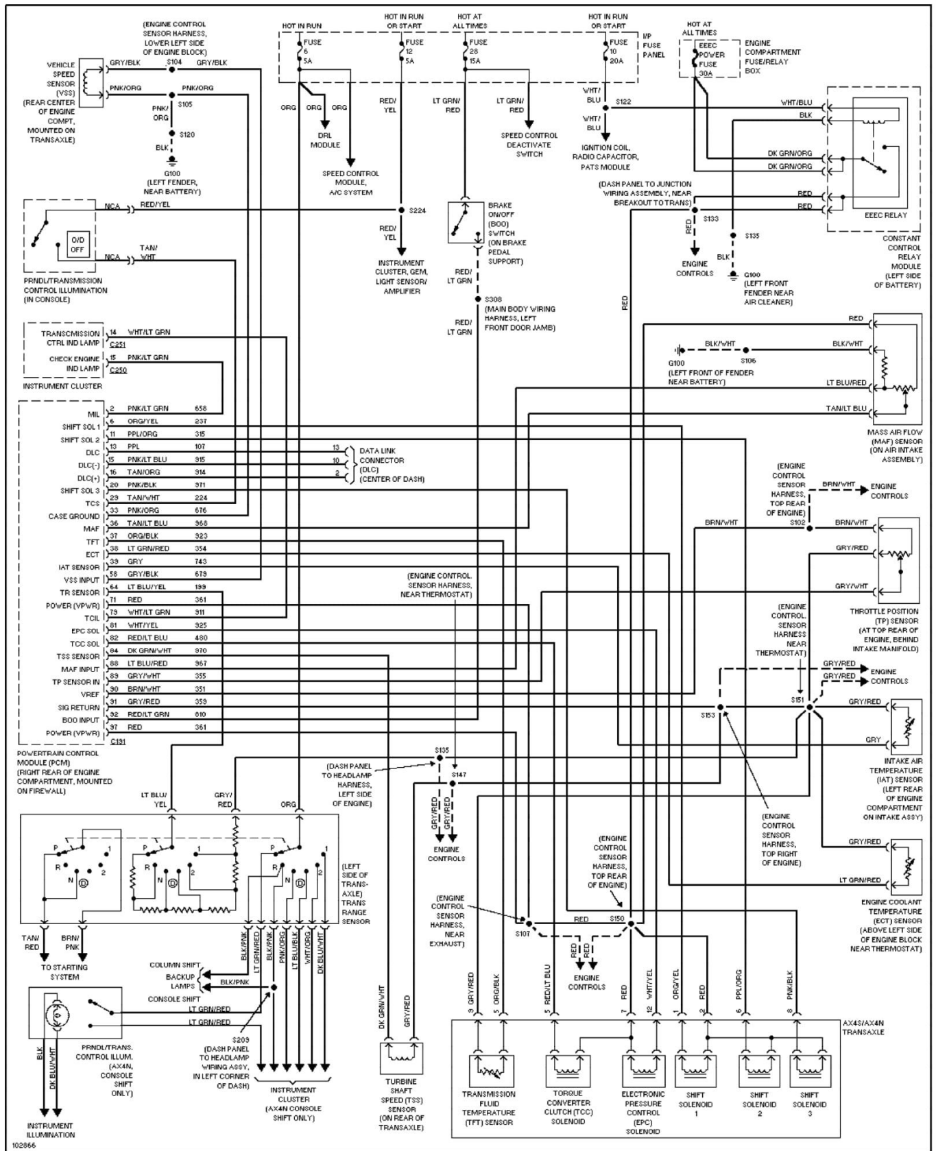
Fig. 72: 3.4L SHO, Transmission Circuit 1997 Ford Taurus LX
