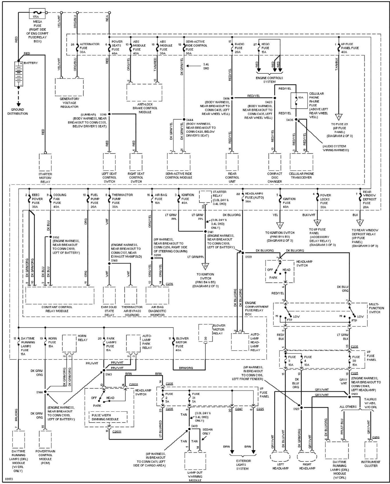
Fig. 51: Power Distribution Circuit (1 of 3) 1997 Ford Taurus LX
