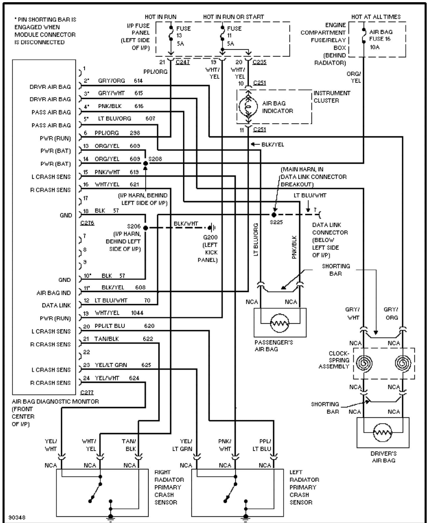
Fig. 68: Supplemental Restraint Circuit 1997 Ford Taurus LX
