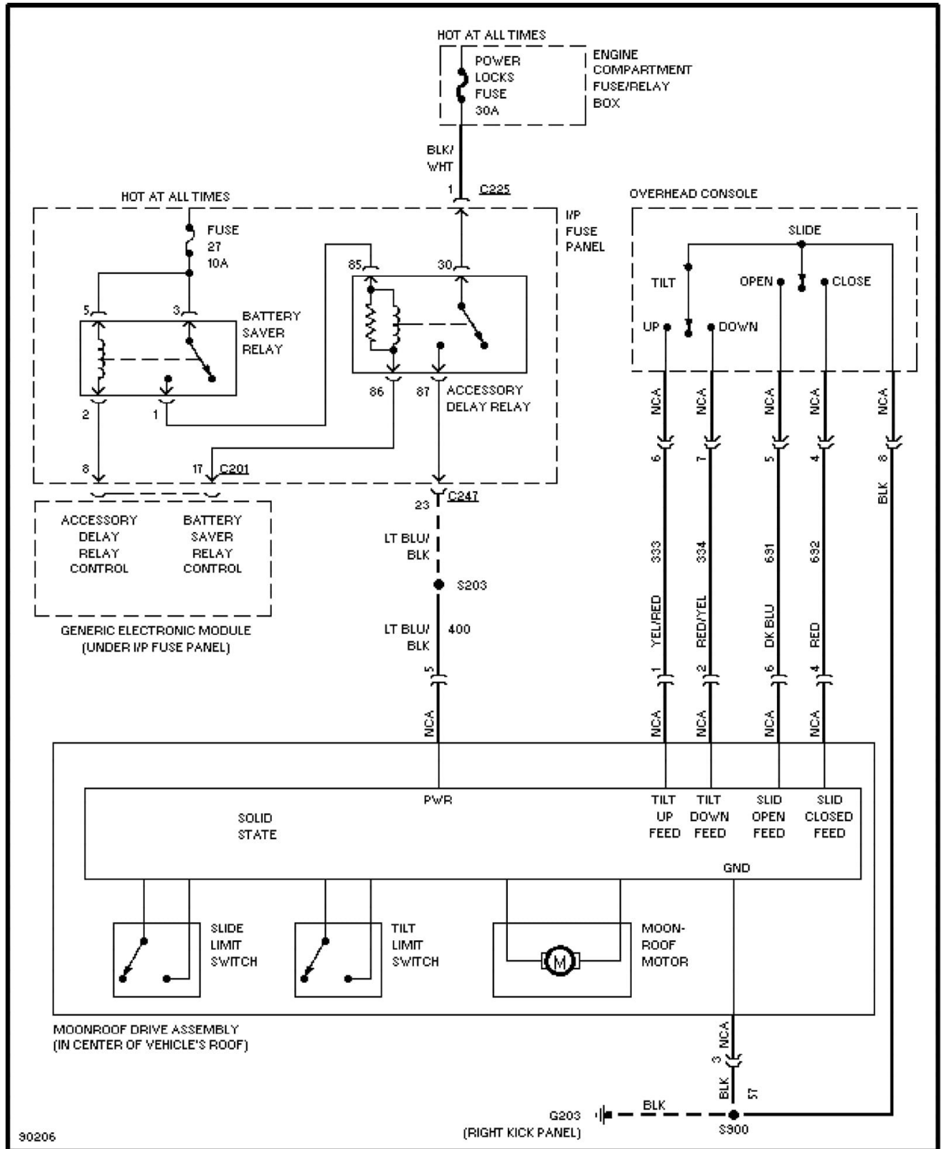
Fig. 57: Power Top/Sunroof Circuits 1997 Ford Taurus LX
