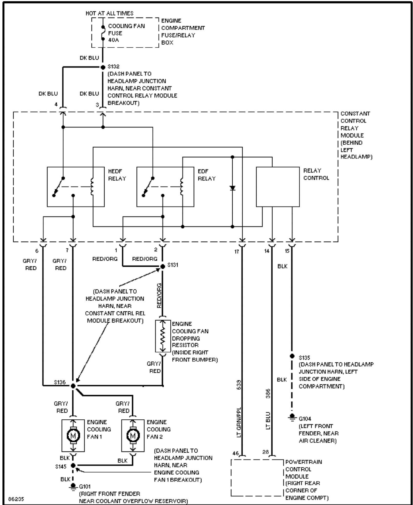
Fig. 7: Cooling Fan Circuit 1997 Ford Taurus LX
