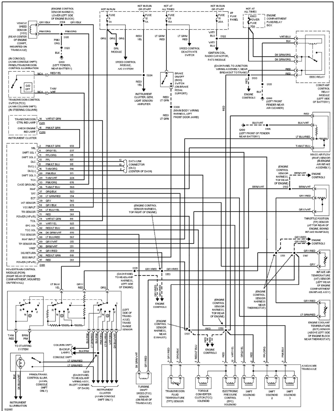
Fig. 70: 3.0L 24-Valve, Transmission Circuit 1997 Ford Taurus LX
