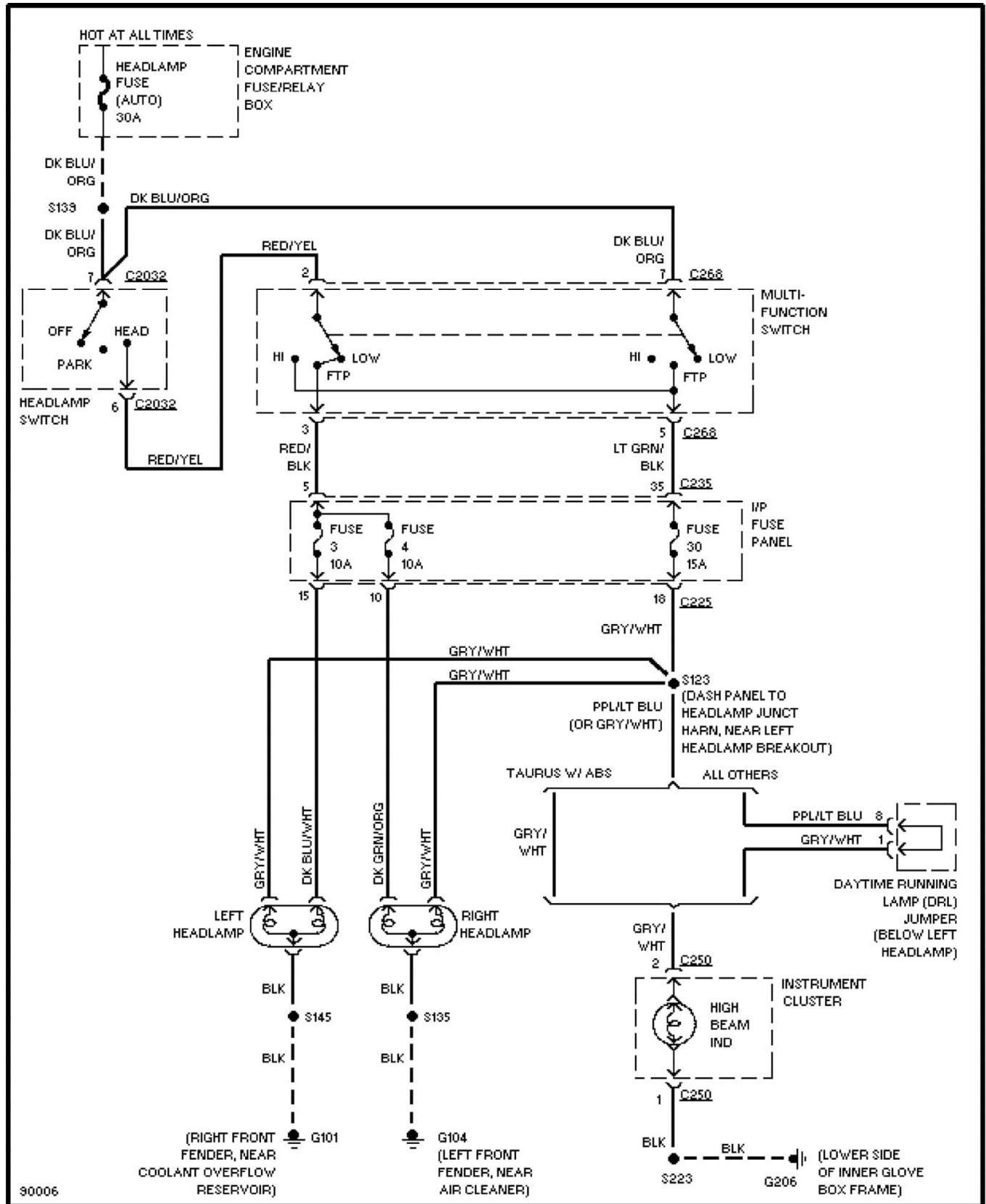
Fig. 41: Headlamps Circuit, W/O DRL 1997 Ford Taurus LX
