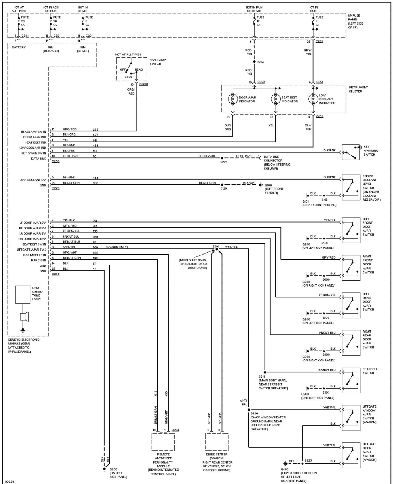
Fig. 74: Warning System Circuits 1997 Ford Taurus LX
