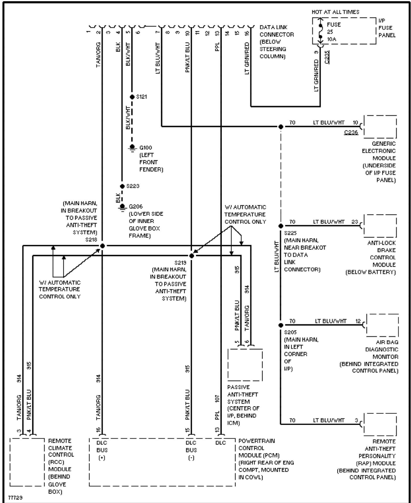
Fig. 6: Computer Data Lines 1997 Ford Taurus LX
