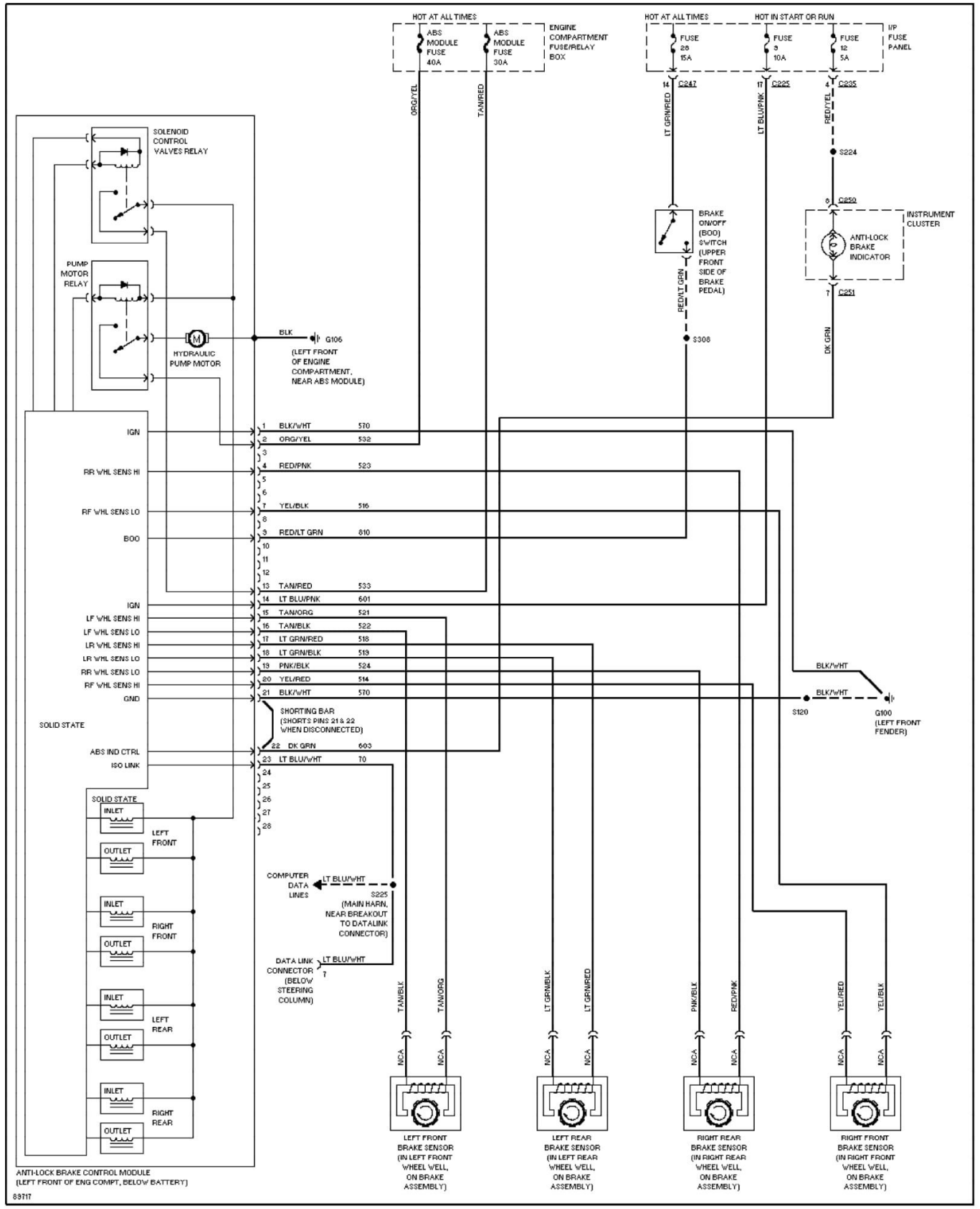
Fig. 3: Anti-lock Brake Circuits 1997 Ford Taurus LX
