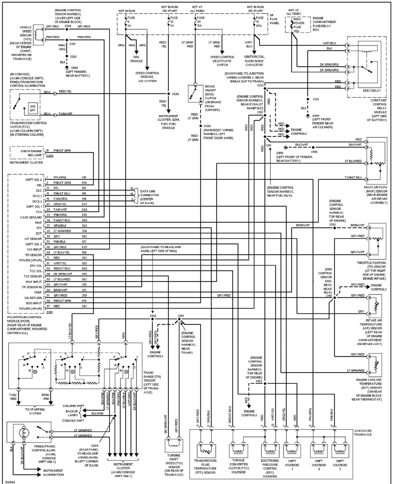
Fig. 69: 3.0L 12-Valve, Transmission Circuit 1997 Ford Taurus LX
