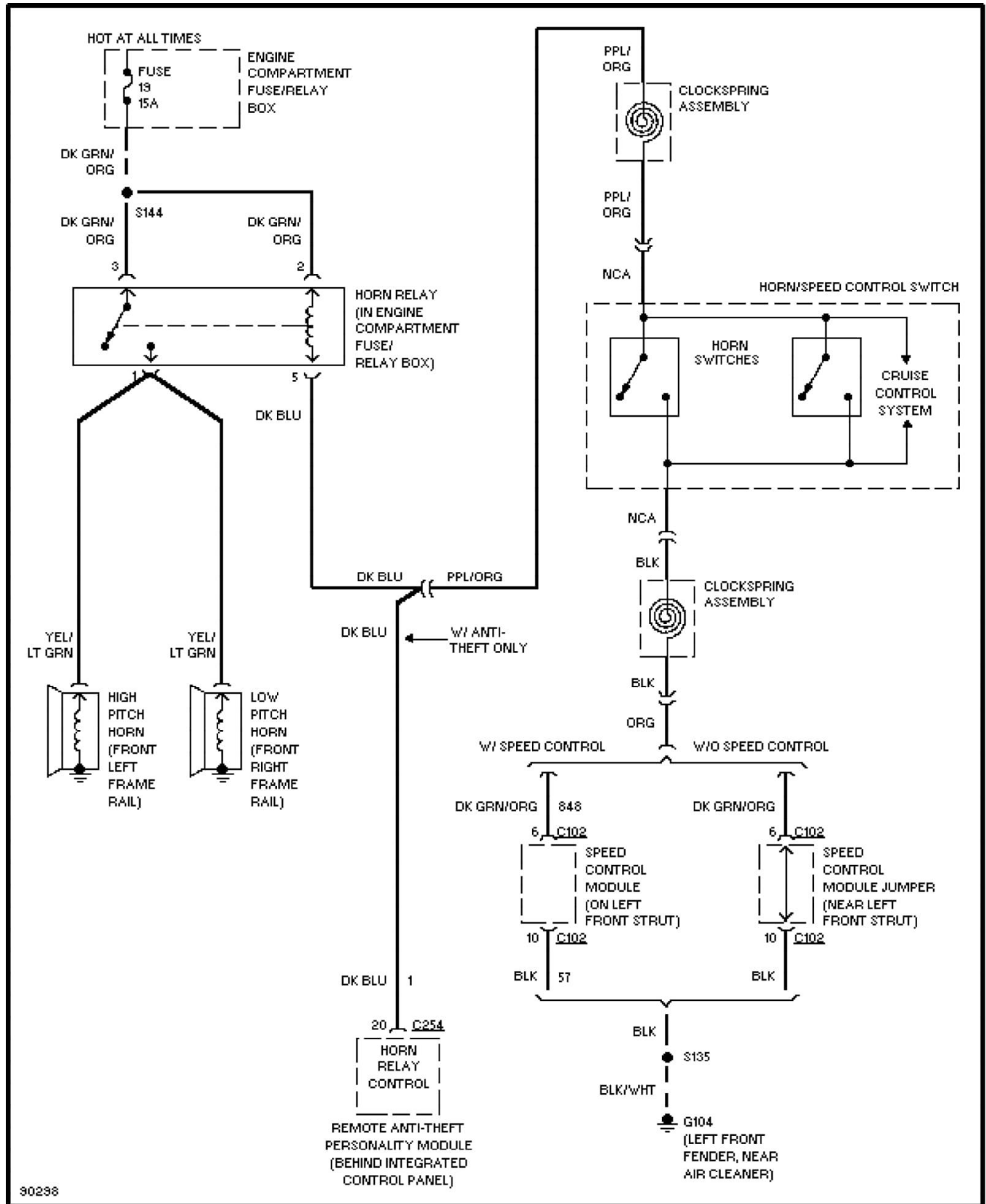
Fig. 42: Horn Circuit 1997 Ford Taurus LX
