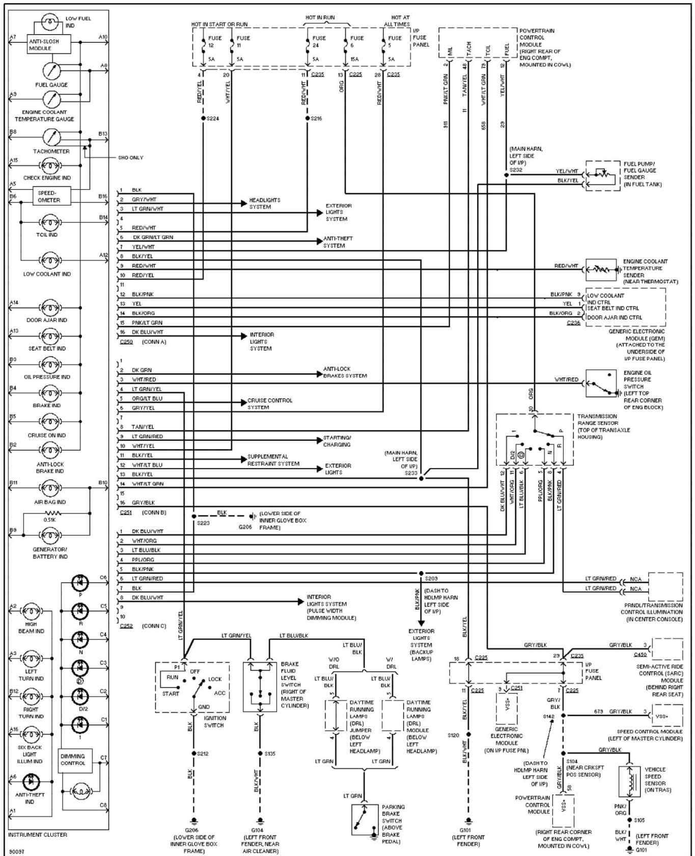
Fig. 44: 3.0L, Instrument Cluster Circuit 1997 Ford Taurus LX
