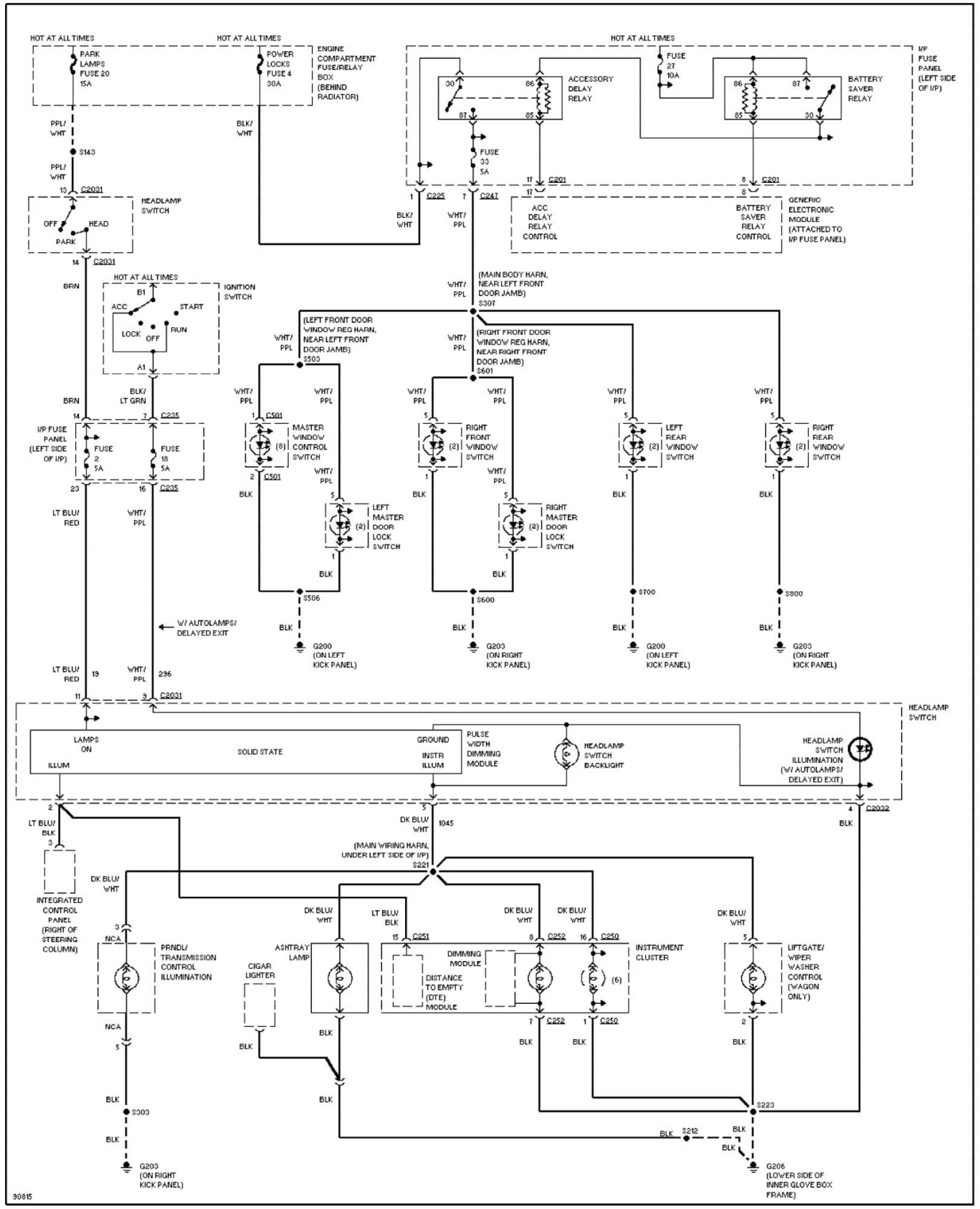
Fig. 49: Instrument Illumination Circuit 1997 Ford Taurus LX
