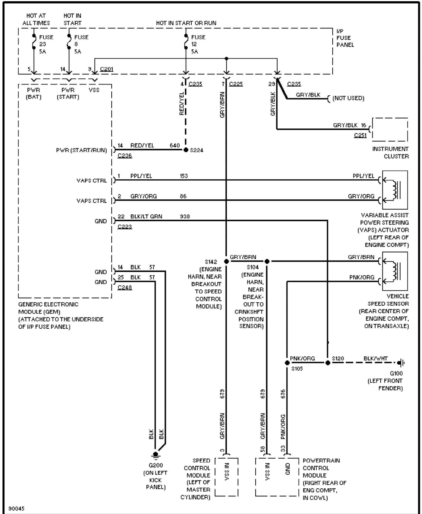
Fig. 10: Electronic Power Steering Circuit 1997 Ford Taurus LX
