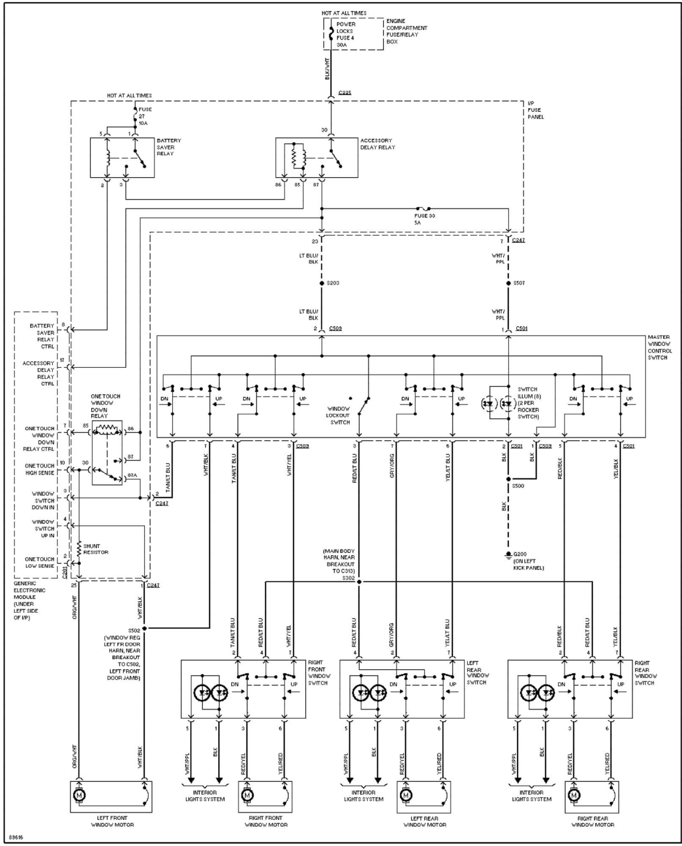
Fig. 58: Power Window Circuit 1997 Ford Taurus LX
